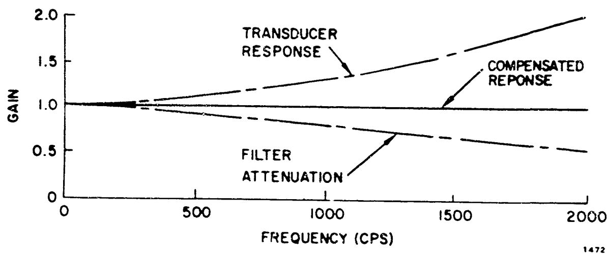
Figure 15. Graph Showing Calculated Action of Filter and Compensated Response When Used in Conjunction With Transducer.
