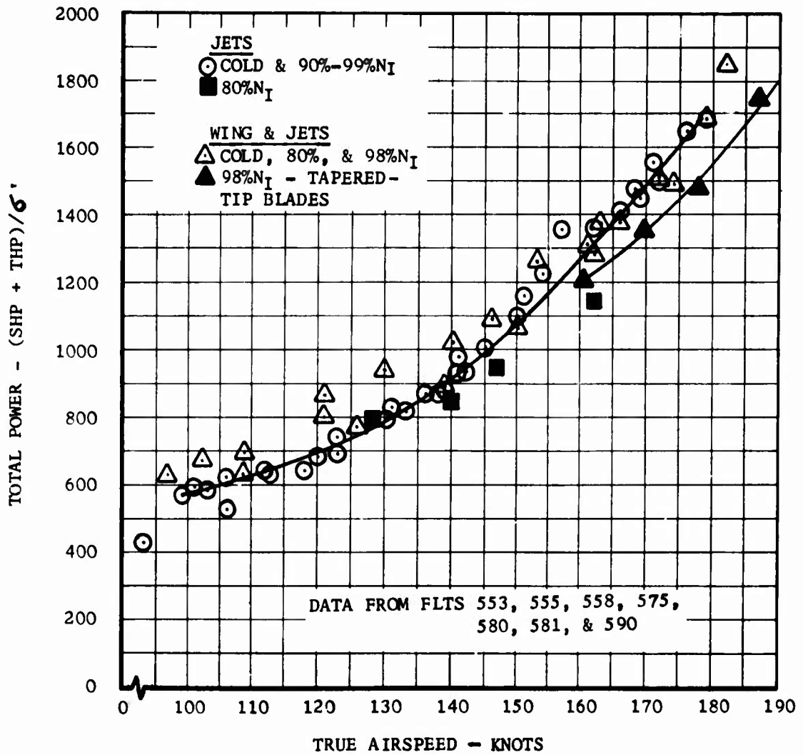
FIGURE 16. TOTAL POWER REQUIRED (T53 SHP + J69 THP).
