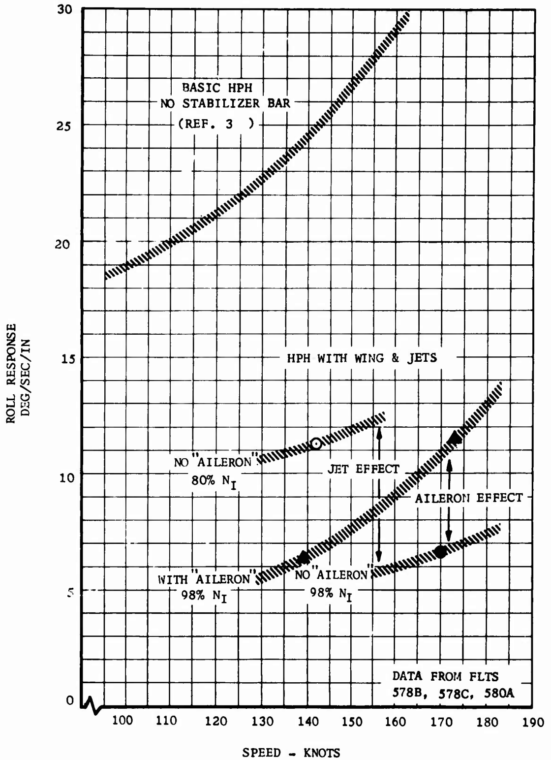
FIGURE 30. ROLL CONTROL RESPONSE - AILERON, JET, AND SPEED EFFECTS.
