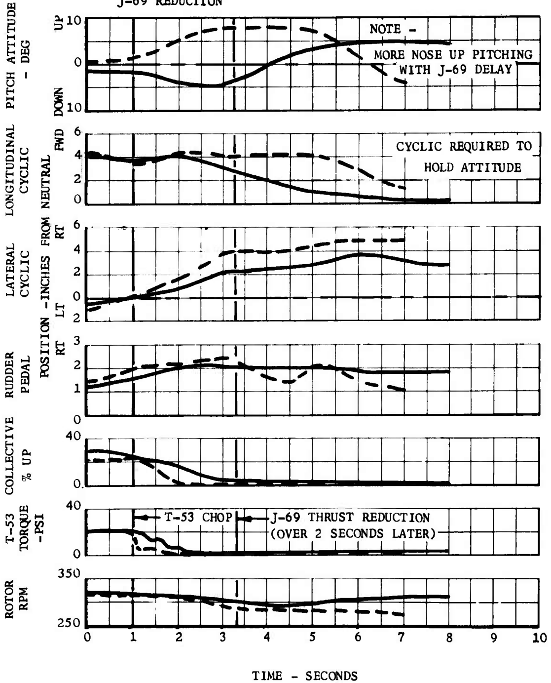
FIGURE 35. EFFECT OF DELAY IN J-69 POWER REDUCTION FOLLOWING SIMULATED T-53 FAILURE.
