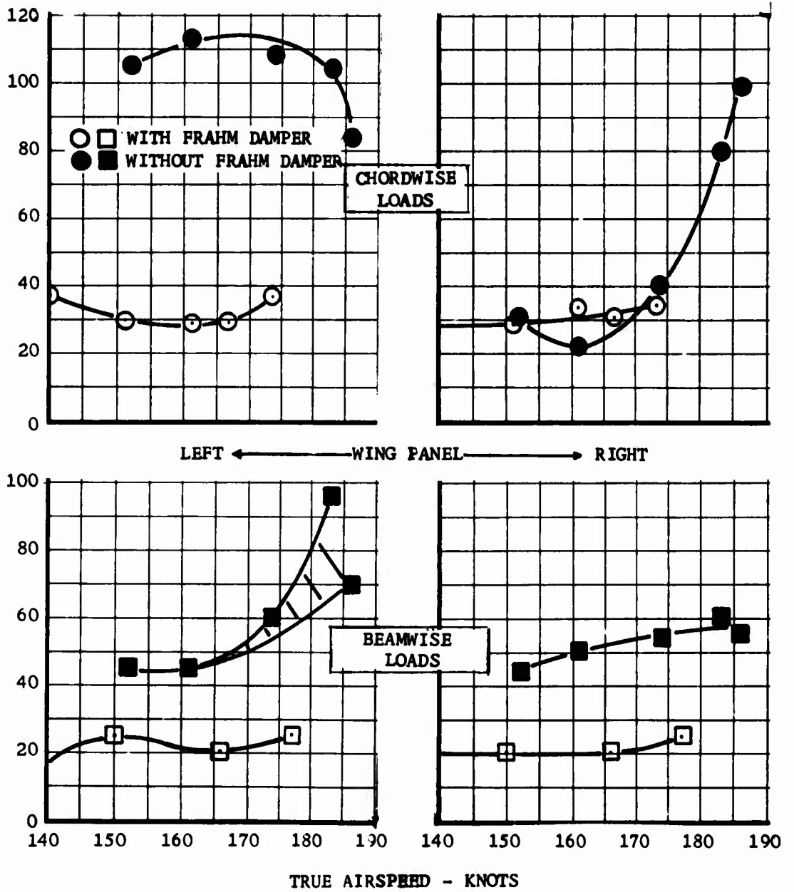
FIGURE 52 EFFECT OF FRAHM DAMPER ON WING LOADS
