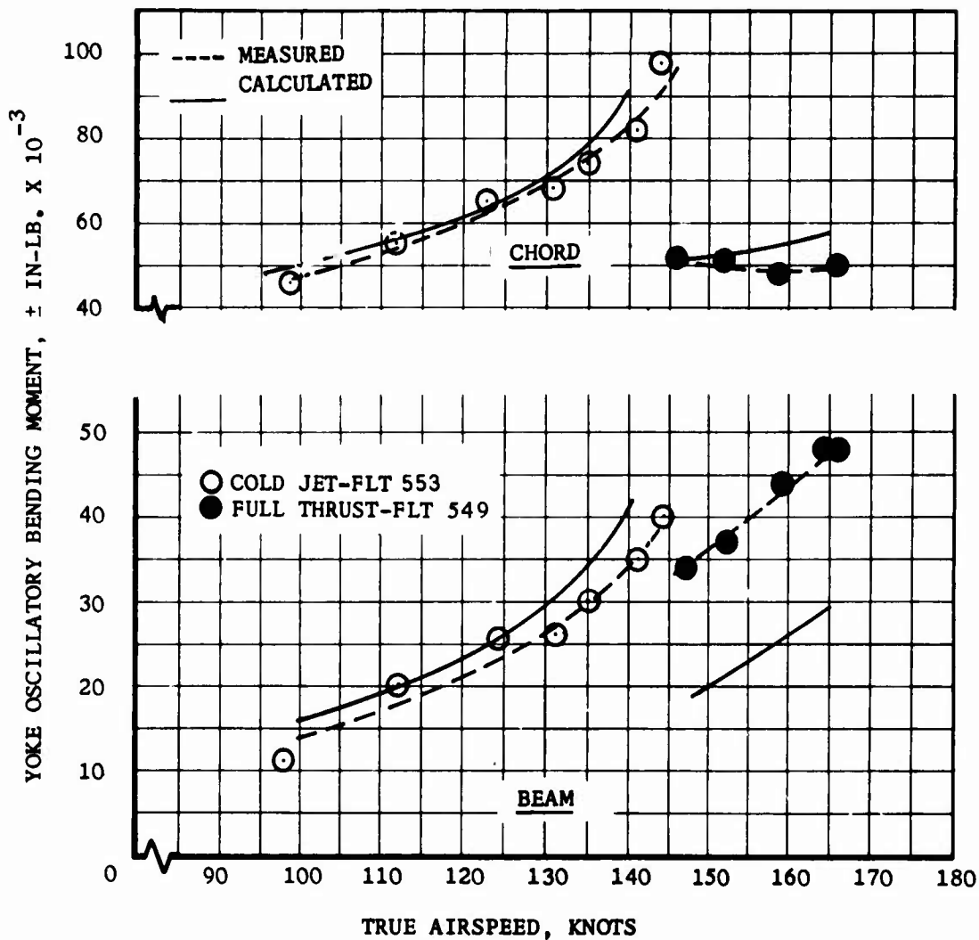
FIGURE 46 COMPARISON OF CALCULATED AND MEASURED MAIN ROTOR LOADS FOR HPH WITH AUXILIARY PROPULSION
