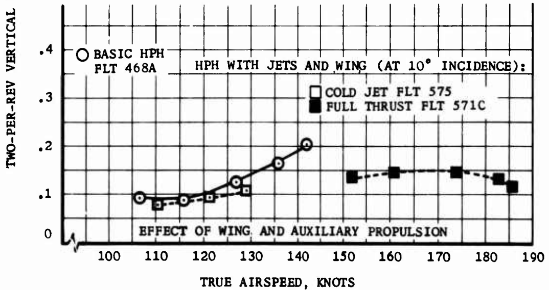
FIGURE 41. PILOT STATION VIBRATION LEVELS
