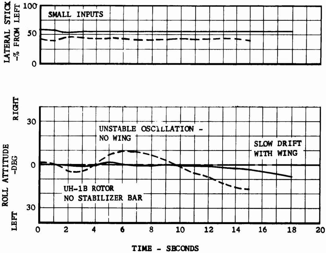
FIGURE 32. WING EFFECT ON ROLL STABILITY.
