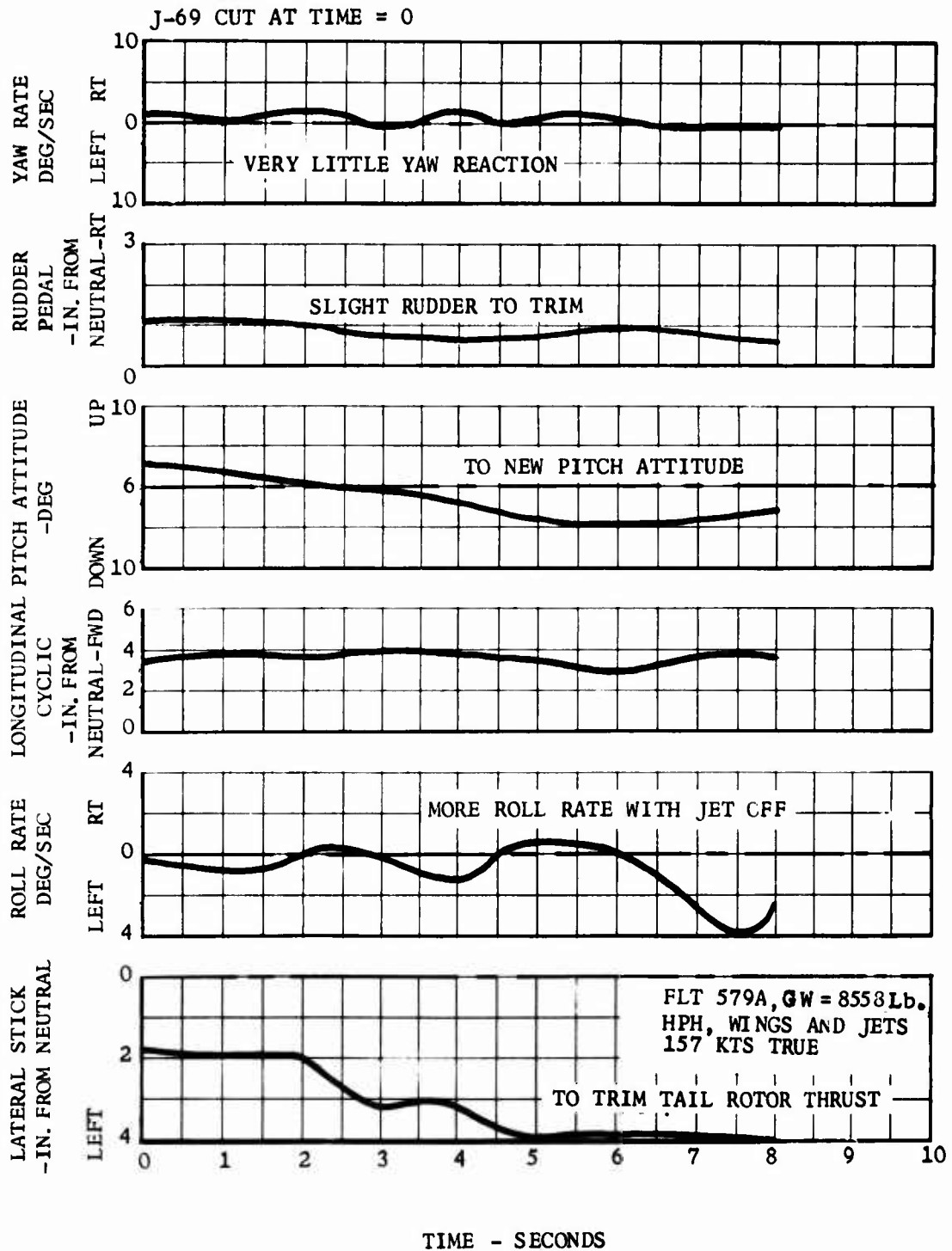
FIGURE 36. TIME HISTORY FOLLOWING SIMULATED RIGHT-HAND J-69 JET FAILURE
