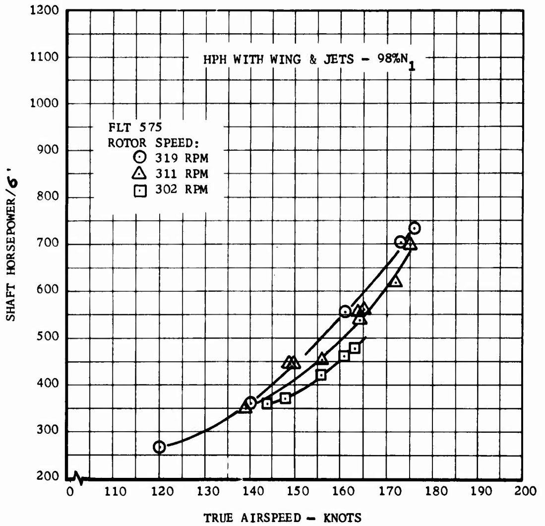
FIGURE 25. INFLUENCE OF ROTOR SPEED ON POWER REQUIREMENTS.
