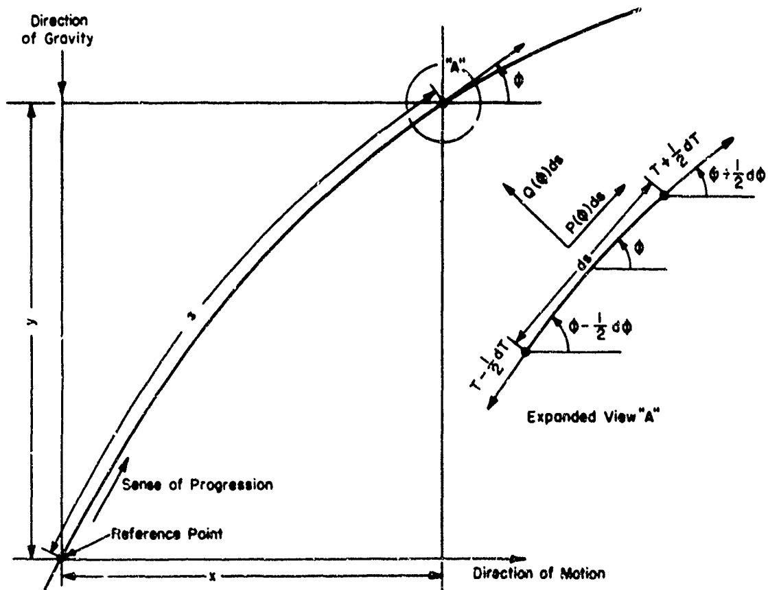
Figure 1 - Coordinate System
