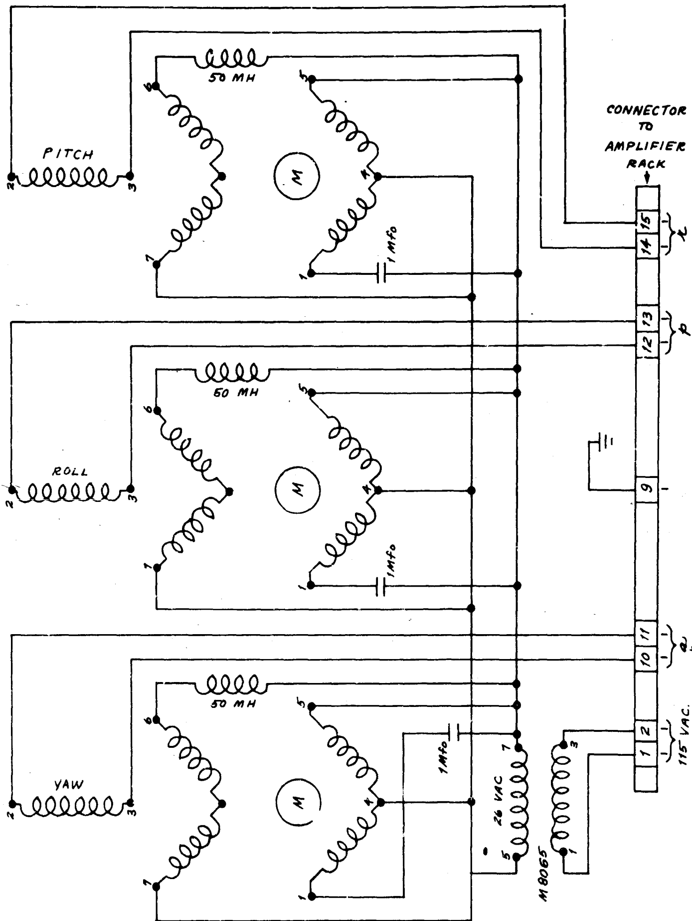
Figure A-23 RATE GYRO CONNECTIONS
