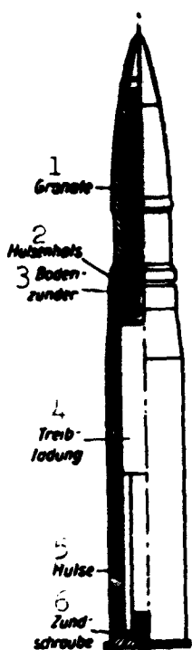
Fig. 14. Fixed-ammunition shell. 1) Shell; 2) casing neck; 3) base detonating fuse; 4) charge; 5) casing; 6) threaded primer.
