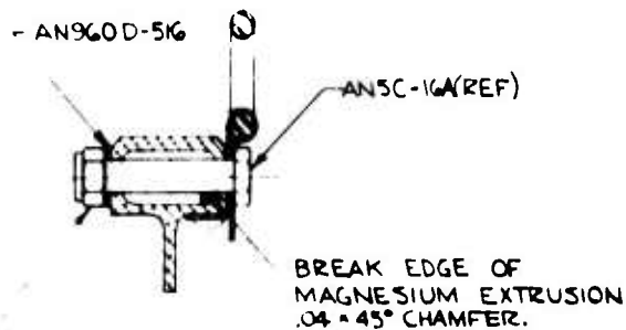
SECTION B-B (TYPICAL FOR ALL -4 INSTALL)
