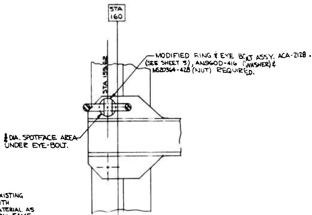
SECTION E-E THIS SECTION APPLIES TO R.H. SIDE ONLY.
