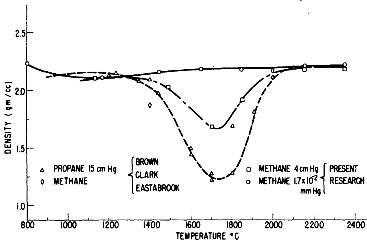
Fig. 2 The room temperature density of pyrolytic graphite as a function of deposition temperature.
