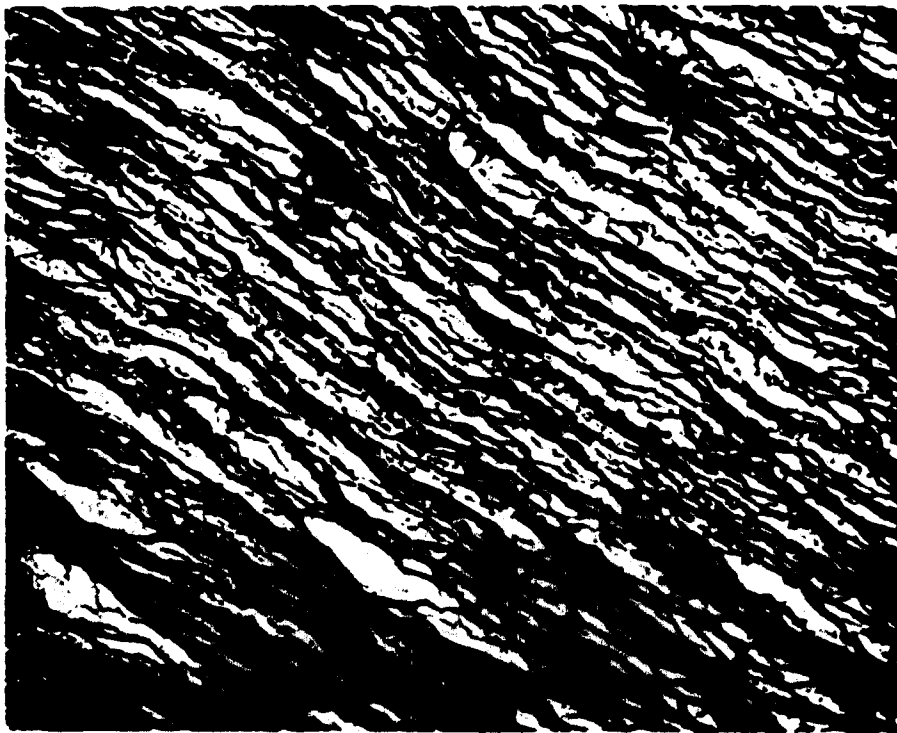
Fig. 3 An electronmicrograph of a fracture surface of a nonsooty pyrolytic graphite deposit. A carbon replica of the fracture surface was made and shadowed with chromium. 5,000X
