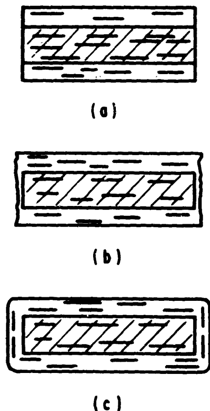
Fig. 1 The cross sections of pyrolytic graphite deposits on pyrolytic graphite substrates. The hatched areas show the initial pieces. (a) At low supersaturations, an unetched substrate coats only on the basal planes. (b) If the substrate is etched with hydrogen prior to deposition at low supersaturations, deposition can occur on all surfaces, but the coating has the same crystallographic orientation as the substrate. (c) At high supersaturations, the substrate is coated on all surfaces, but the coating is deposited such that the C-axis is always normal to the surface.
