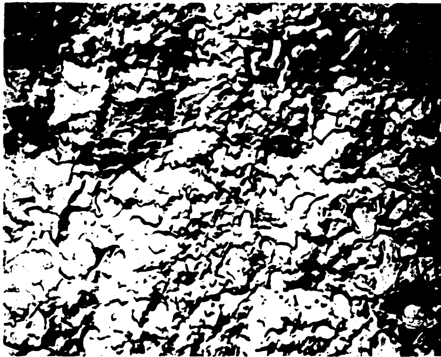
Fig. 4 An electronmicrograph of a fracture surface of a sooty pyrolytic graphite deposit. A carbon replica of the fracture surface was made and shadowed with chromium. 5,000X
