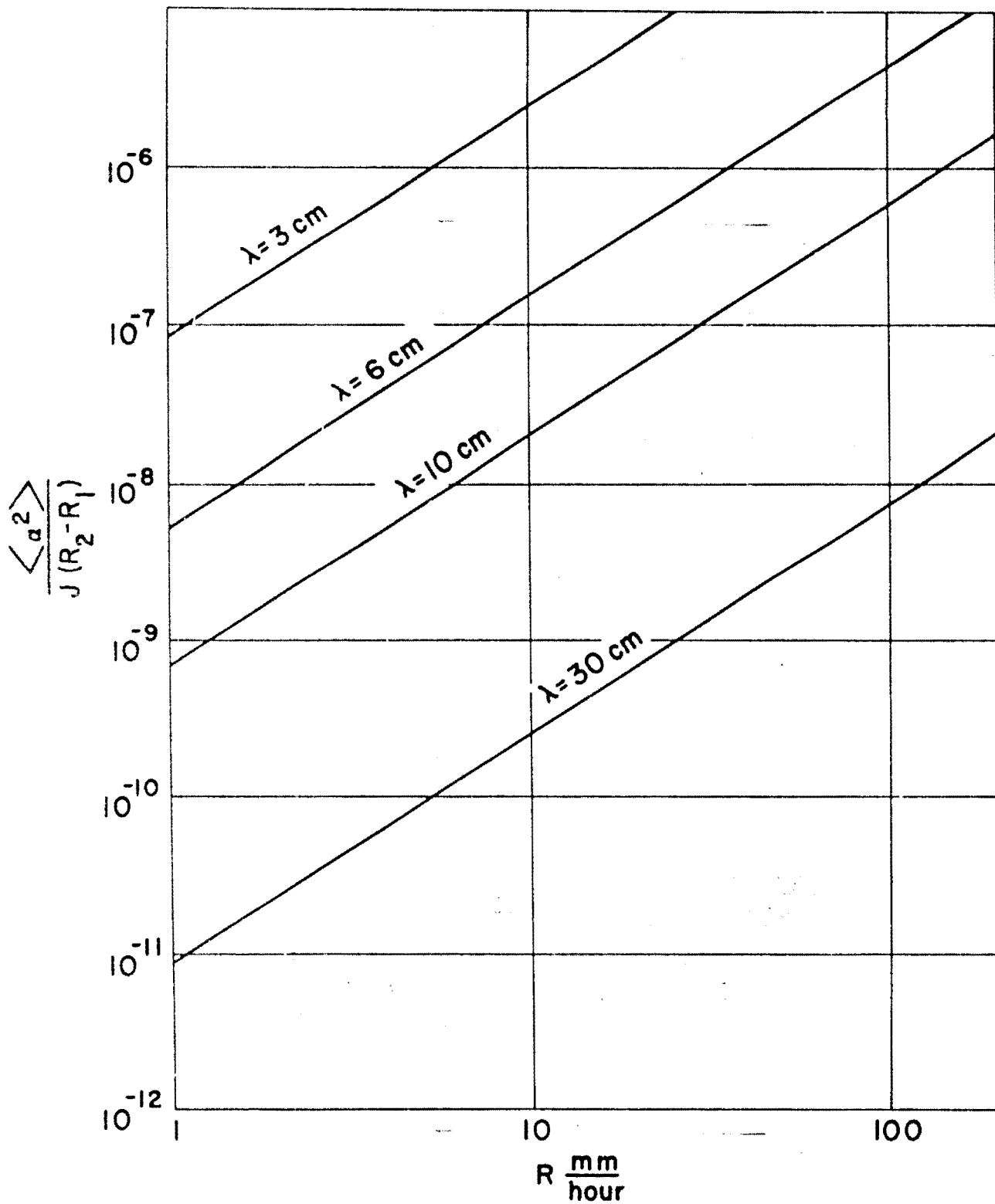
Figure 11 RMS Phase Error for Scattering by Rainfall
