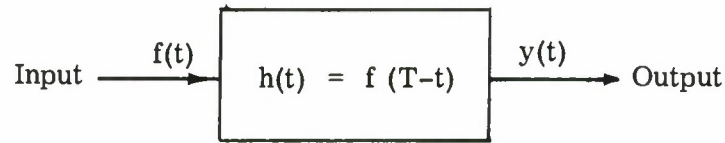
Fig. 1. Matched Filter
