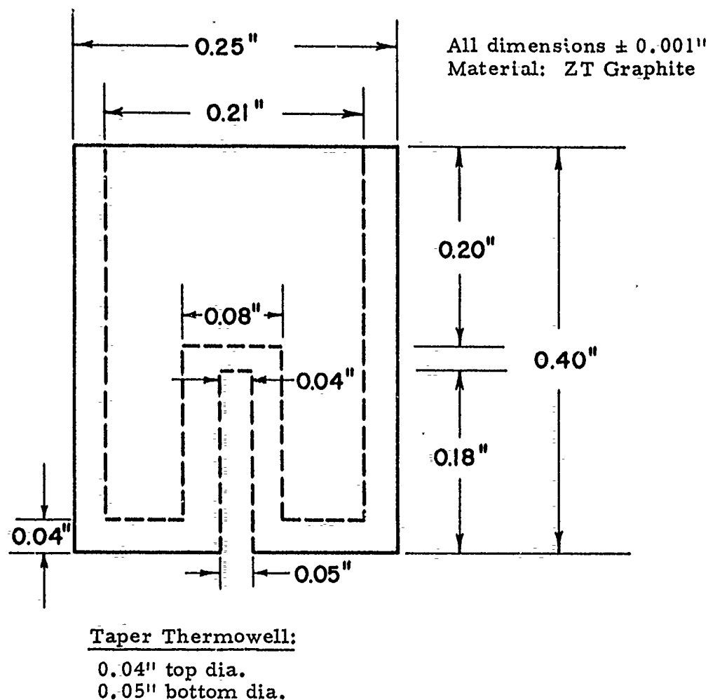
Figure 45. DTA Capsule
