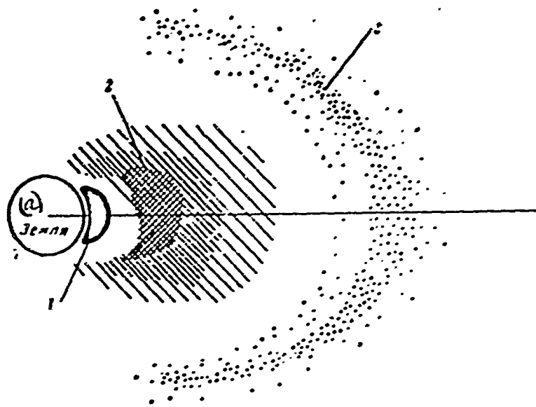
Fig. 6. Configuration of belts of charged particles surrounding Earth. 1—Internal radiation belt; 2—External radiation belt; 3—The most external belt of charged particles. KEY: (a) Earth.
