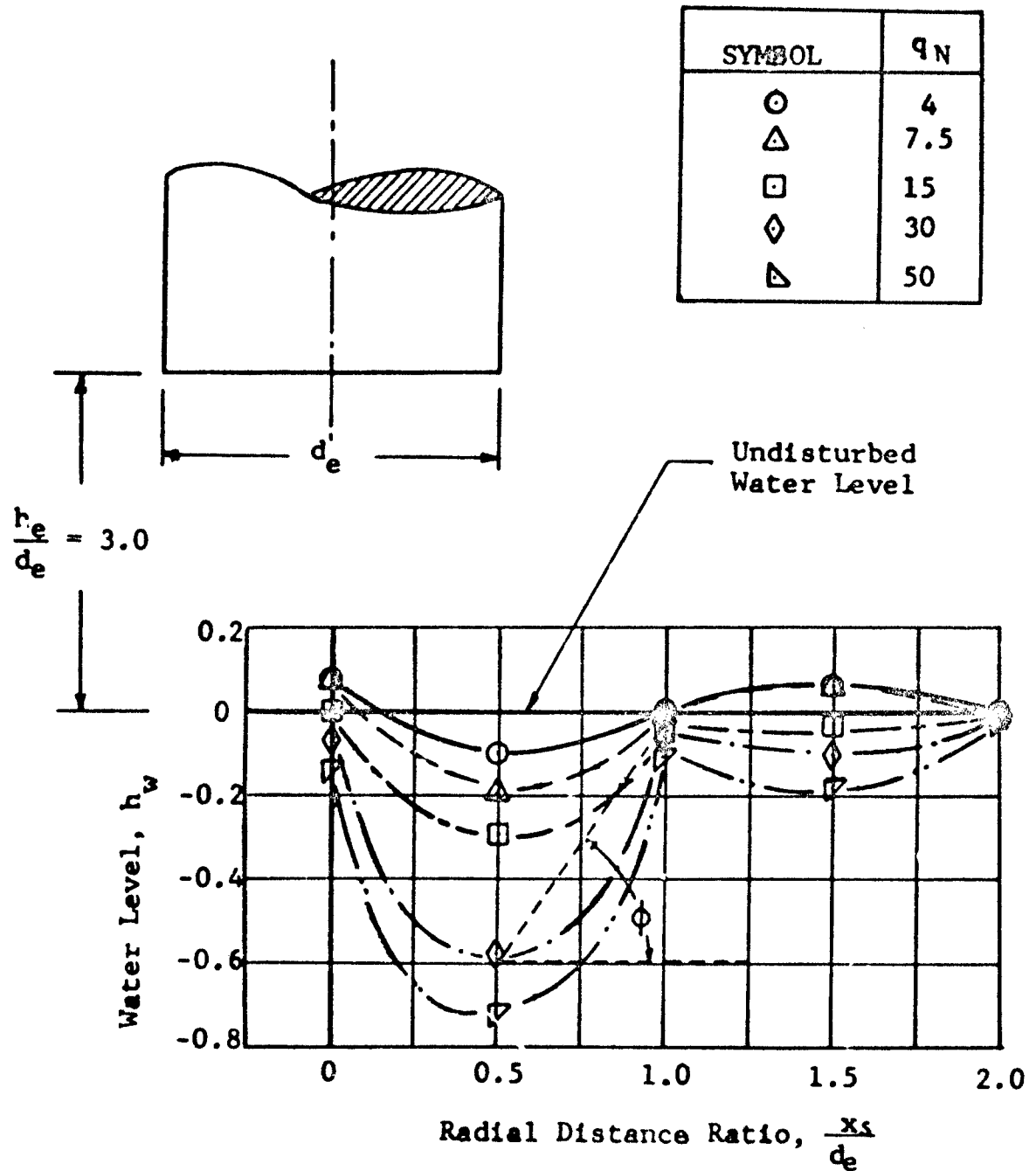
FIGURE 11: WATER SURFACE DEFLECTION FOR VARIOUS DYNAMIC PRESSURES AS A FUNCTION OF RADIAL DISTANCE (Reference 9)
