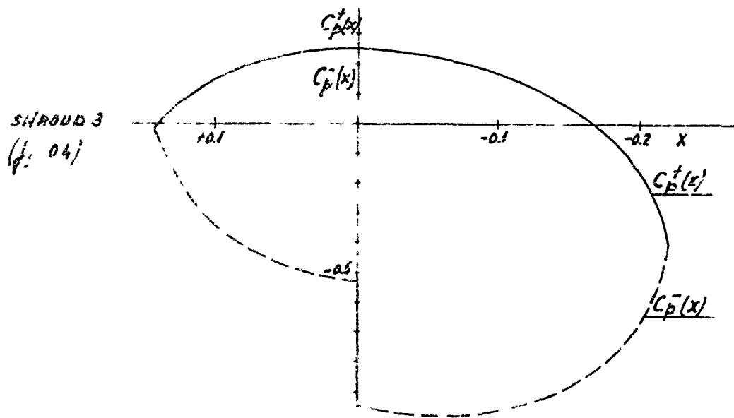
PRESSURE COEFFICIENTS ALONG THE SHROUD AS A FUNCTION OF THE LOADING OF THE SHROUD.
