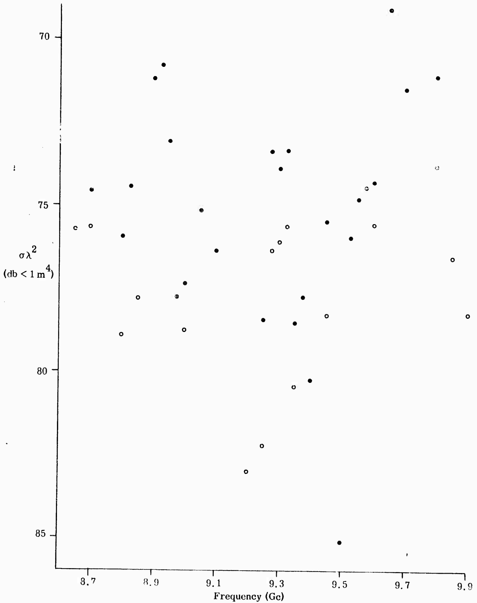
Fig. 2-8 SCATTERING BEHAVIOR OF BLOCKS N (•••) AND R (ooo)
