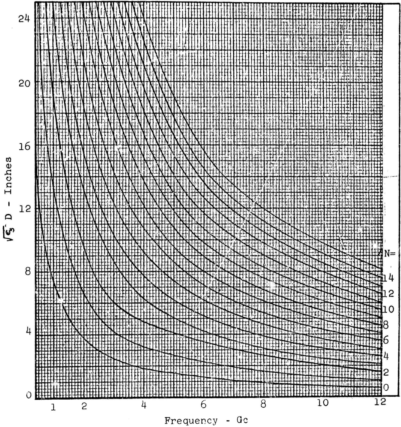
Fig. 3-2 COLUMN DIAMETER VERSUS FREQUENCY FOR MINIMUM BROADSIDE CROSS SECTION OF A PLASTIC FOAM CYLINDER
