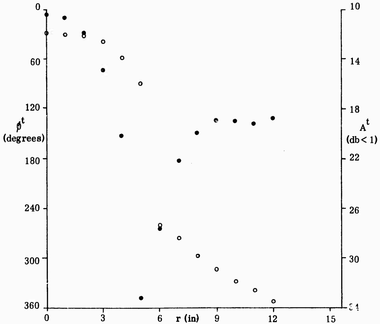
Fig. 2-19 AMPLITUDE (●) AND PHASE (○) OF TOTAL FIELD FOR d = 64\text{-}1/2 IN.
