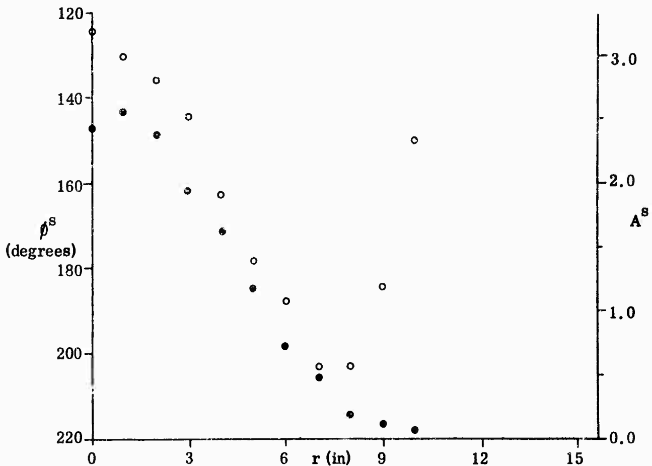
Fig. 2-23 RELATIVE AMPLITUDE (●) AND PHASE (○) OF SCATTERED FIELD FOR d = 64\text{-}1/2 IN.
