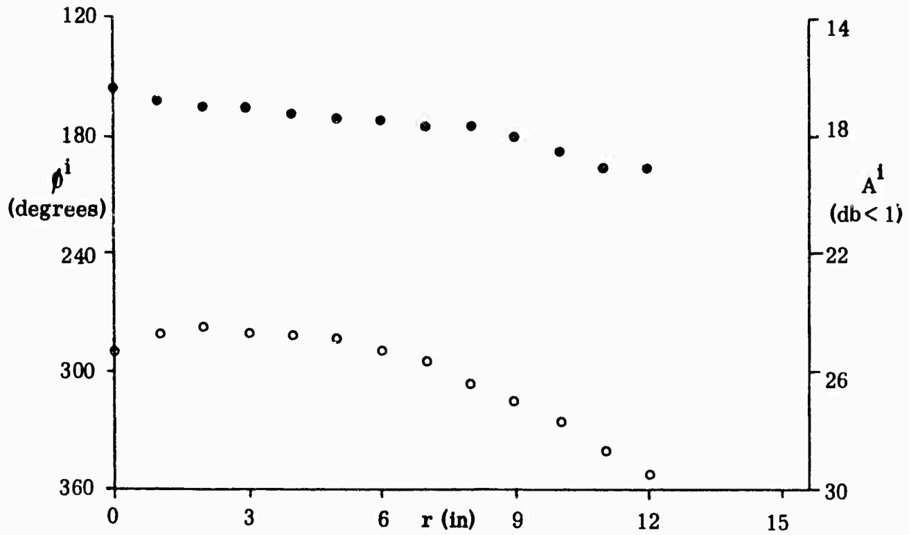
Fig. 2-18 AMPLITUDE (●) AND PHASE (○) OF INCIDENT FIELD FOR d = 64\text{-}1/2 IN.
