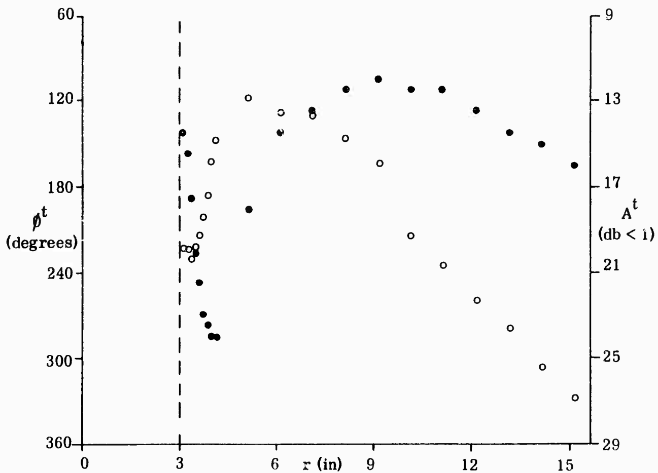
Fig. 2-15 AMPLITUDE (●) AND PHASE (○) OF TOTAL FIELD FOR d = 41-1/2 IN.
