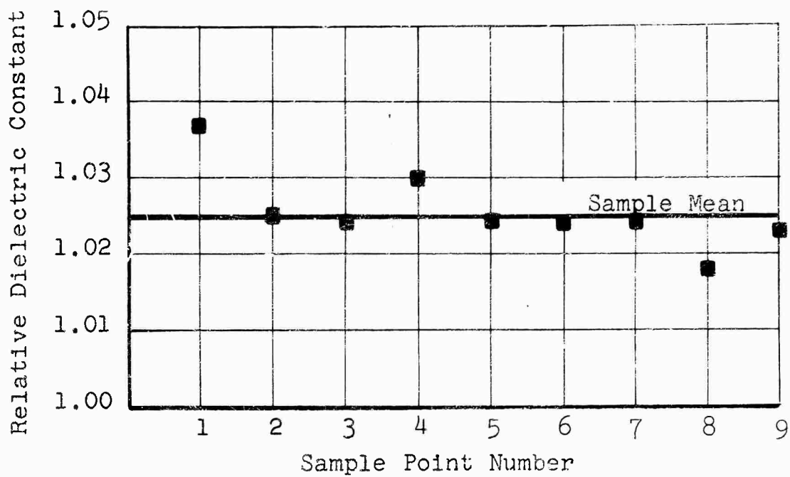
Fig. 3-1 CALCULATED DIELECTRIC CONSTANT FOR STYROFOAM
