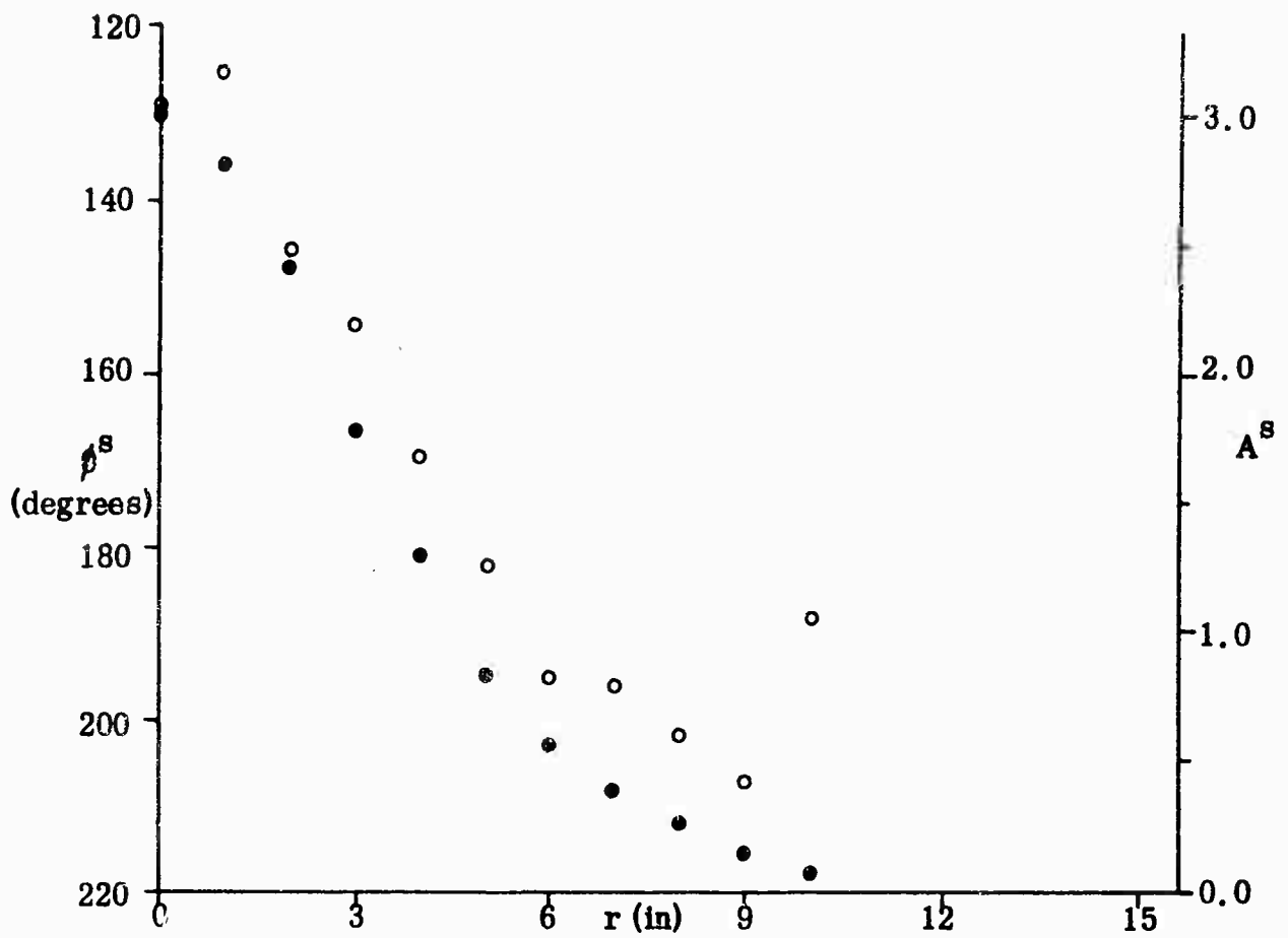
Fig. 2-22 RELATIVE AMPLITUDE (●) AND PHASE (○) OF SCATTERED FIELD FOR d = 56\text{-}3/4 IN.
