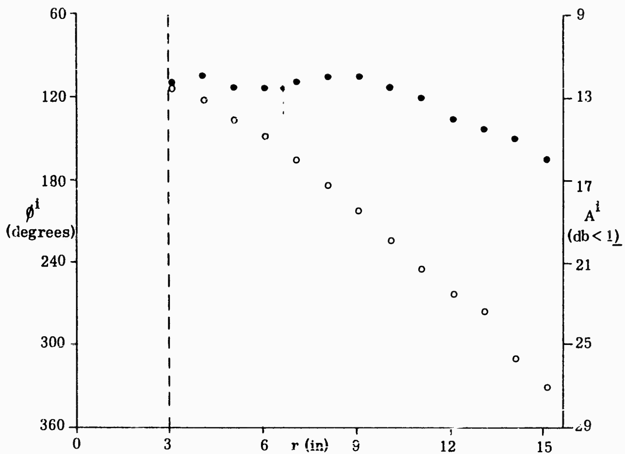
Fig. 2-14 AMPLITUDE (●) AND PHASE (○) OF INCIDENT FIELD FOR d = 41-1/2 IN.
