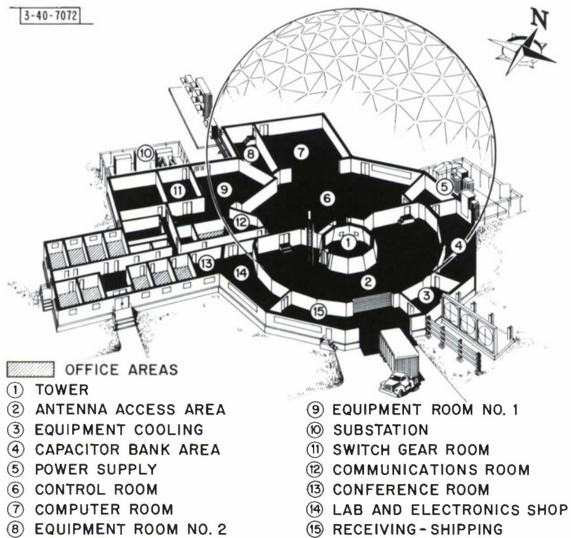
Fig. 17. Building layout.
