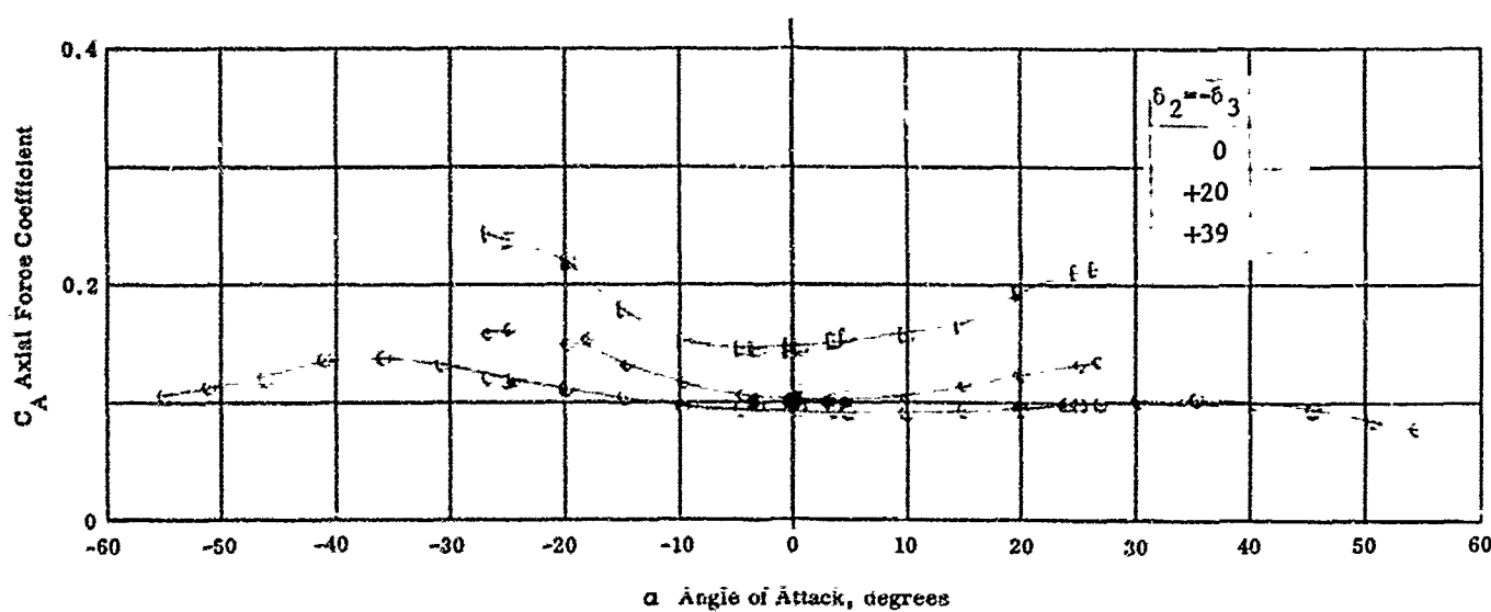
Fig. 23d Configuration IV - M_\infty = 8.08 , C_N & C_A vs. \alpha Re_\infty / ft \times 10^{-6} = 2.26 \delta_1 = 0 \delta_2 = -\delta_3 = 0, +20, +39
