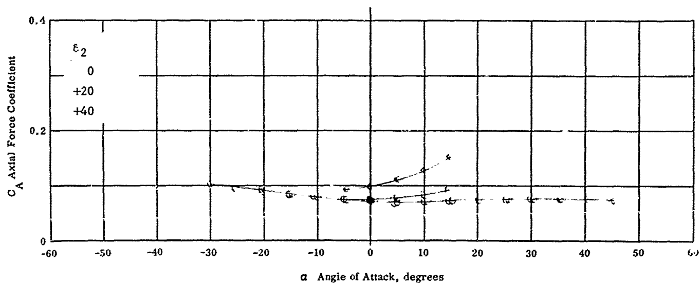
Fig. 11b Configuration I - M_\infty = 5.01 C_N & C_A vs. \alpha Re_c / ft \times 10^{-6} \gamma_1 = \gamma_3 = 0 \delta_2 = 0, +20, +40
