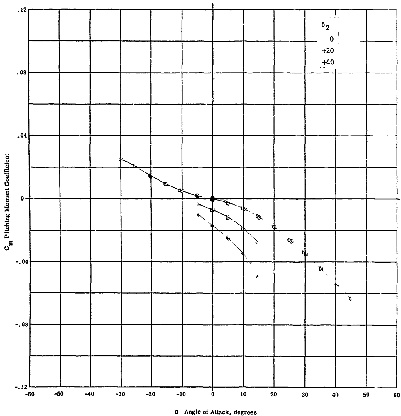
Fig. 11e Configuration I - M_\infty = 5.01 C_m vs. \alpha R_\infty / ft \times 10^{-6} = 2.26 \delta_1 = \delta_3 = 0 \delta_2 = 0, +20, +40
