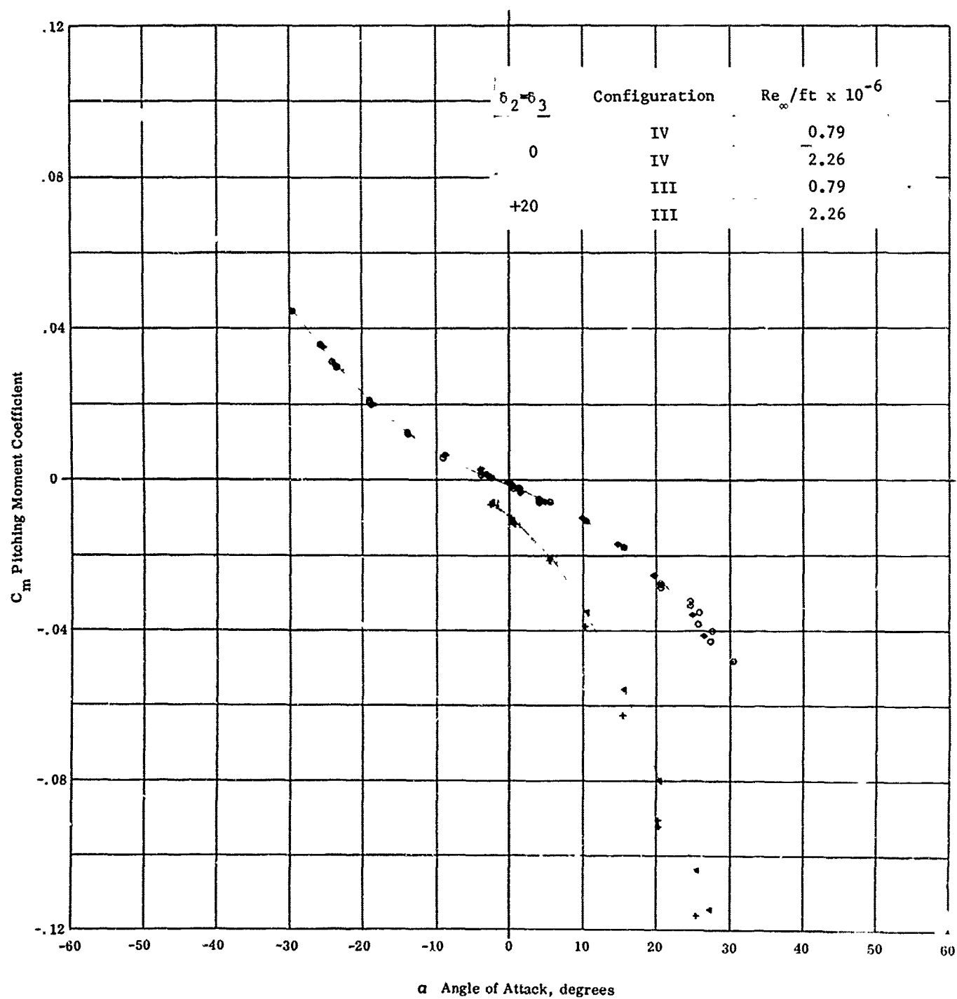
Fig. 18b Configuration III - M_\infty = 8.08 , C_m vs. \alpha Re_\infty / ft \times 10^{-6} = 0.79, 2.26 \delta_1 = 0 \delta_c = \delta_2 = \delta_3 = 0, +20
