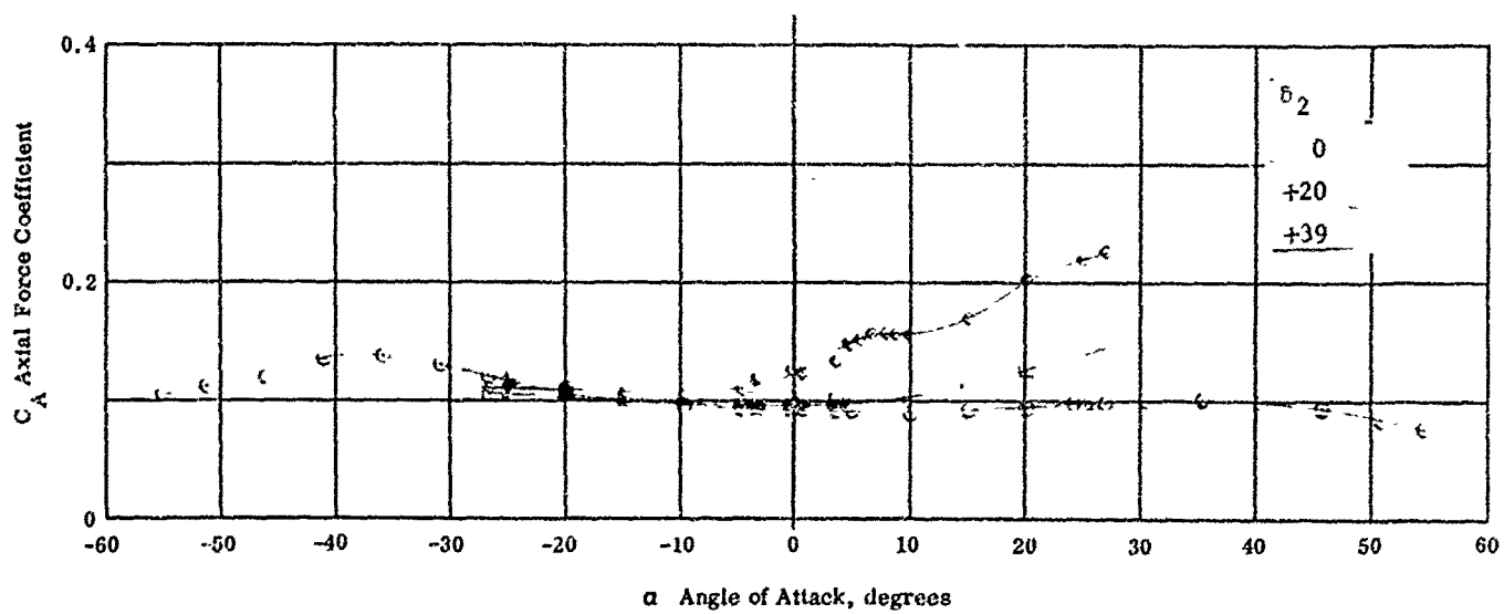
Fig. 23a Configuration IV - M_\infty = 8.03 , C_N & C_A vs. Re_\infty / ft \times 10^{-6} = 2.26 b_1 = b_3 = 0 \delta_2 = 0, +20, +39 129
