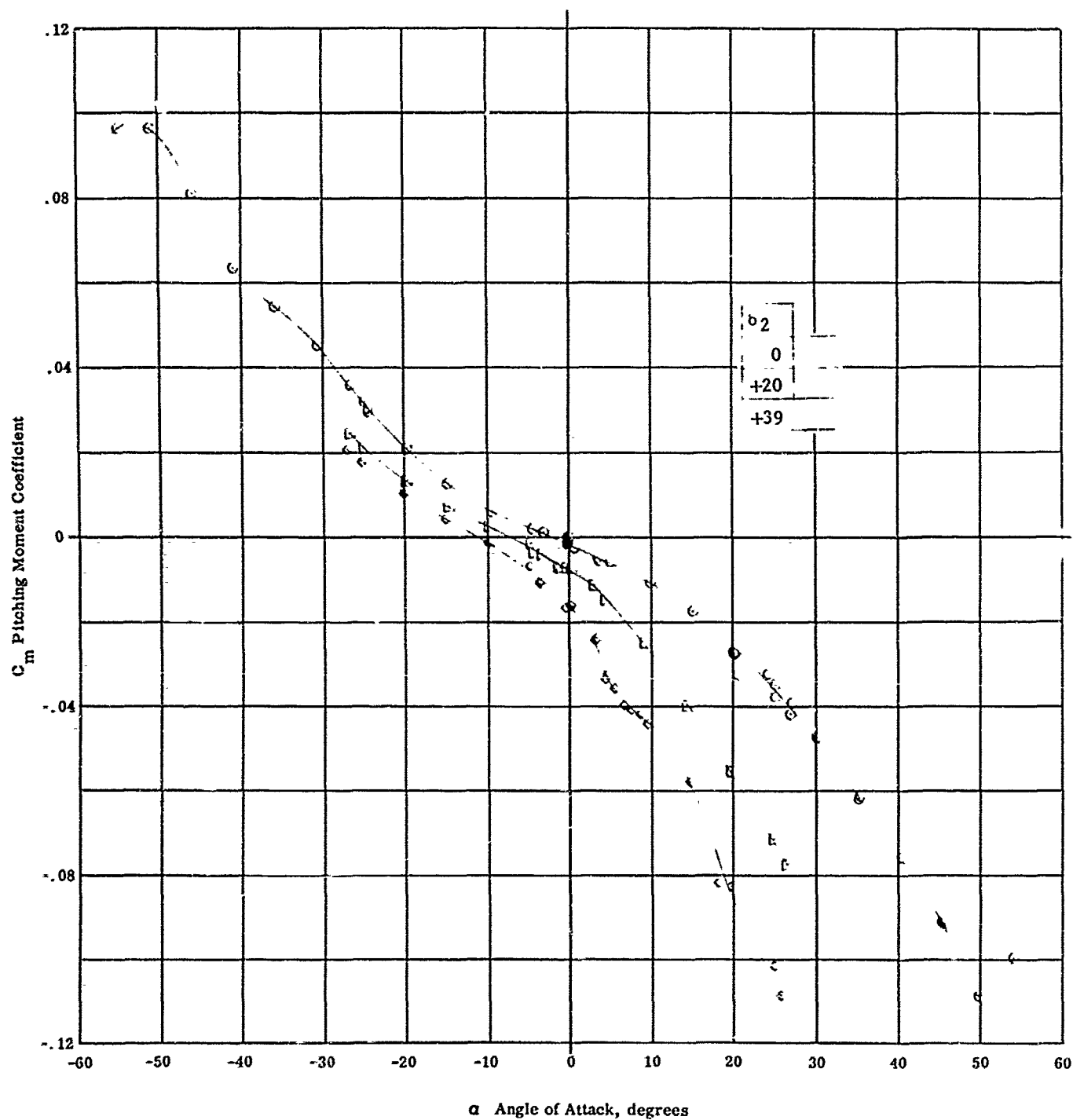
Fig. 23f Configuration IV - M_\infty = 8.08 , C_m vs. \alpha
