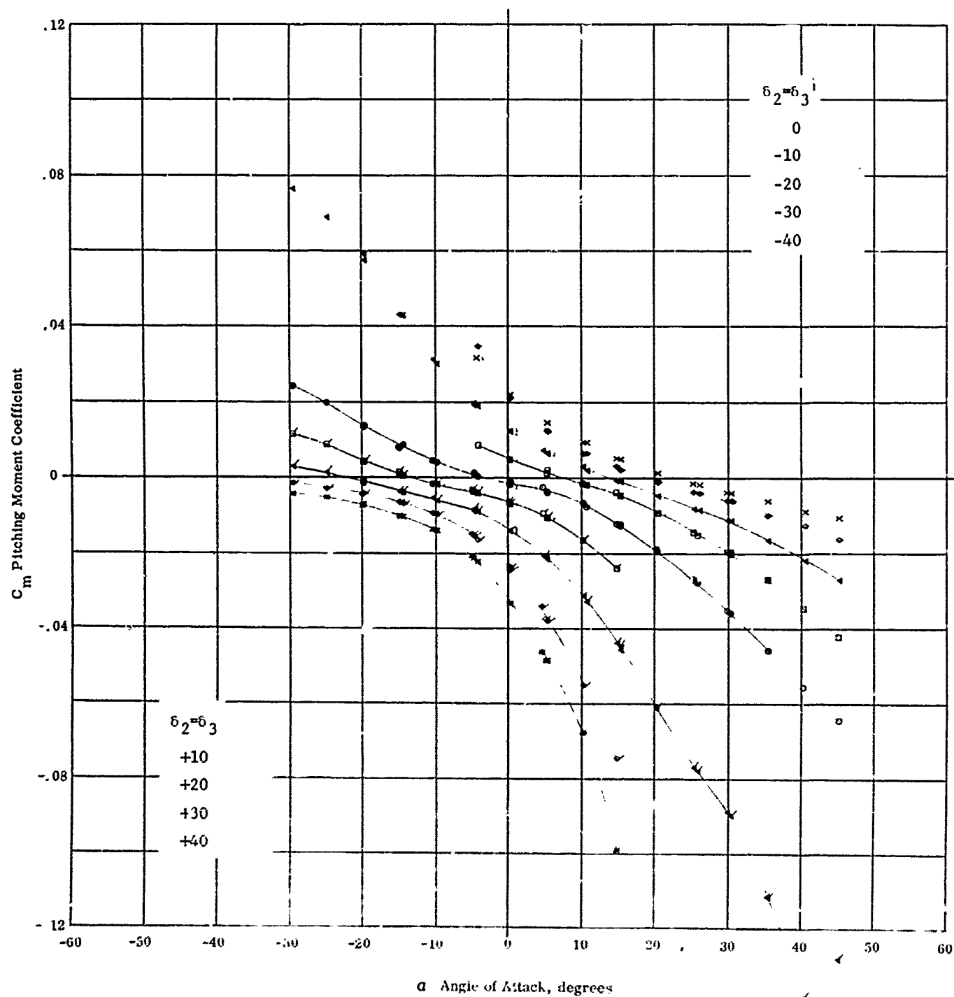
Fig. 3e Configuration I - M_\infty = 5.01 , C_{m_0} vs. \alpha , Re / ft \times 10^{-6} = 2.26 \delta_1 = 0 , \delta_2 = \delta_3 = 0, \pm 10, 20, 30, 40
