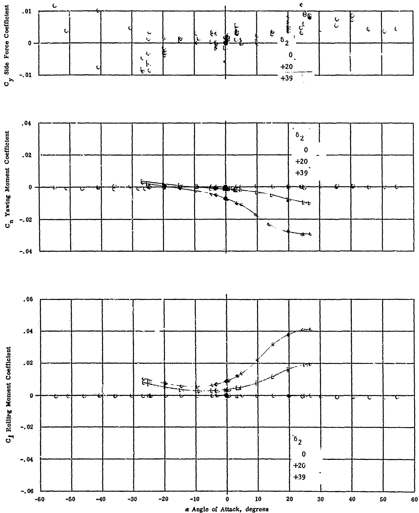
Fig. 22k Configuration I - M_\infty = 8.08 , C_y , C_n , C_l vs. \alpha Re_\infty / ft \times 10^{-6} = 2.26 \delta_1 = \delta_3 = 0 \delta_2 = 0, +20, +39 124
