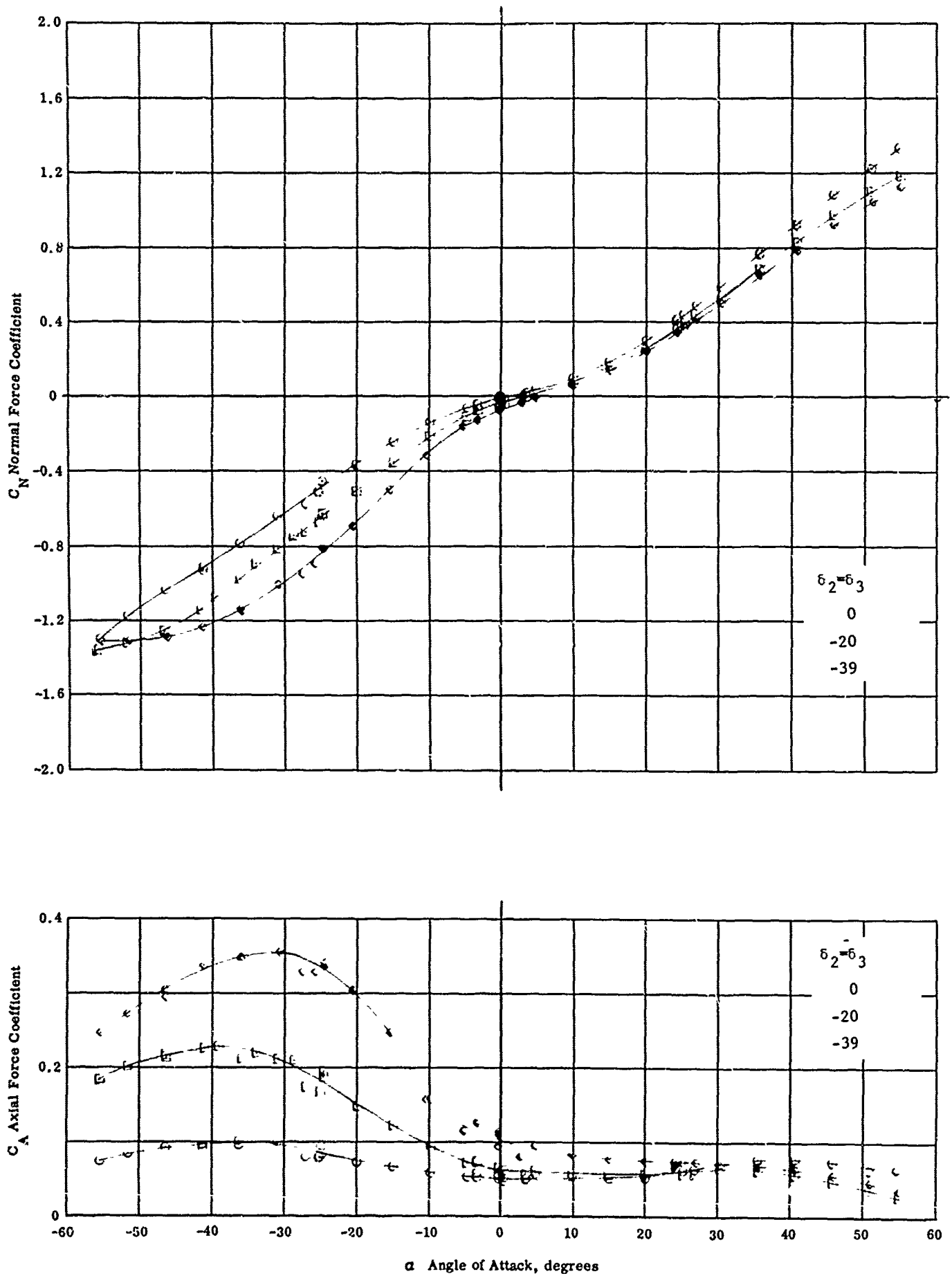
Fig. 13b Configuration I - M_\infty = 8.08 , C_N & C_A vs. \alpha
