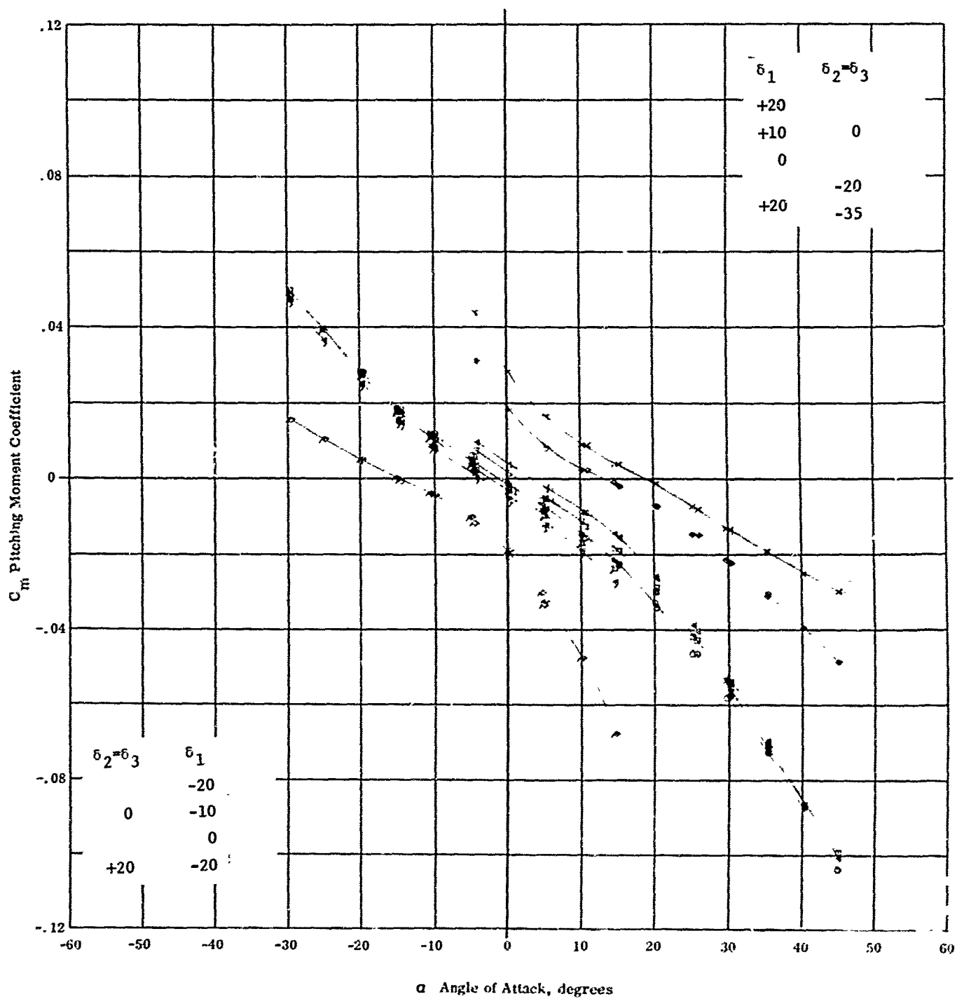
Fig. 10d Configuration IV - M = 5.01 , C_m vs. \alpha Re_\infty / \bar{c} \times 10^{-6} = 2.26 \delta_1 = 0, \pm 10, \pm 20 , \delta_2 = \delta_3 = 0 \delta_1 = -20 , \delta_2 = \delta_3 = +20 \delta_1 = +20 , \delta_2 = \delta_3 = -20, -35
