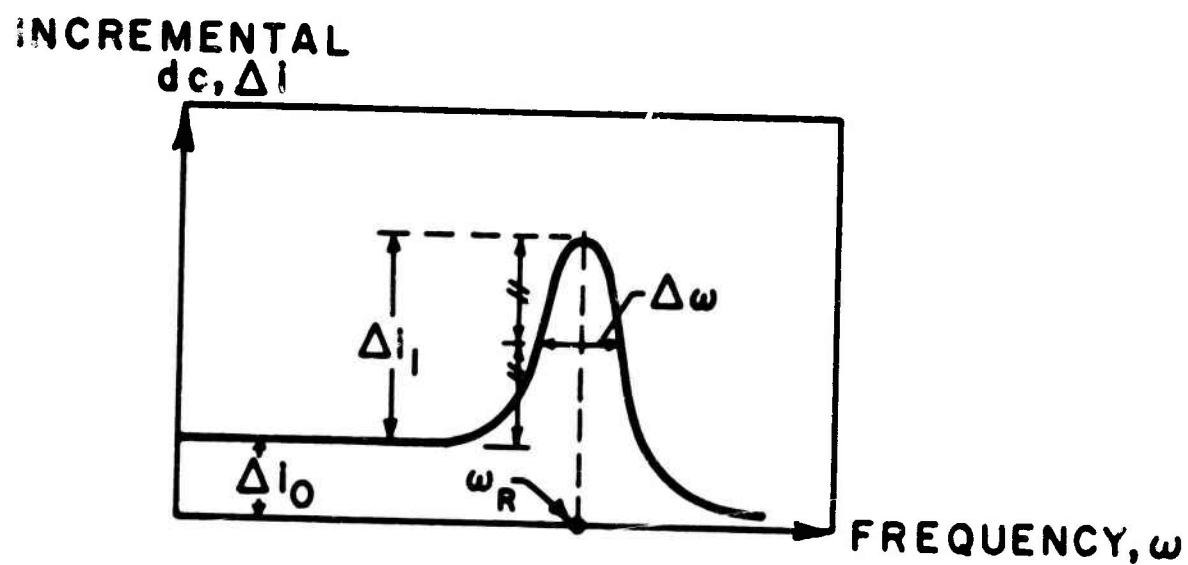
(b) VARIATION OF INCREMENTAL d c WITH FREQUENCY
