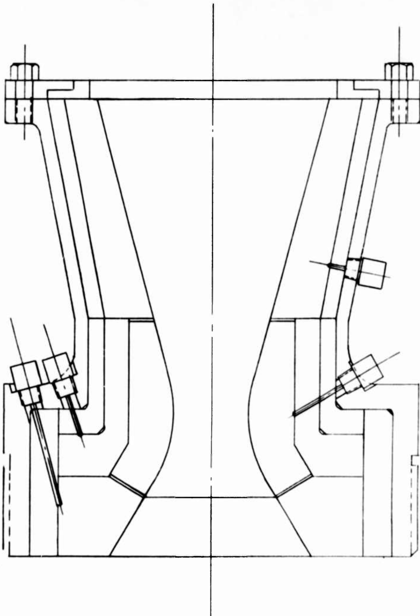
FIGURE 4 INSTRUMENTATION LOCATION
