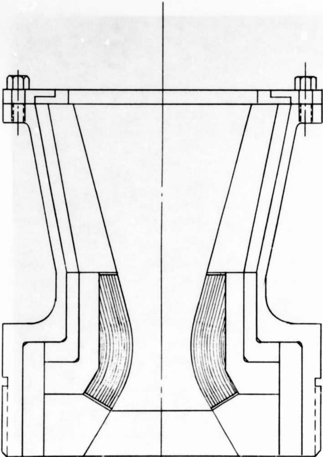
1. 1.12 Inch Diameter Throat Fixed Nozzles
