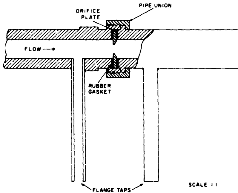
Fig. 4 - Diagram of orifice plate, holder, and flange taps
