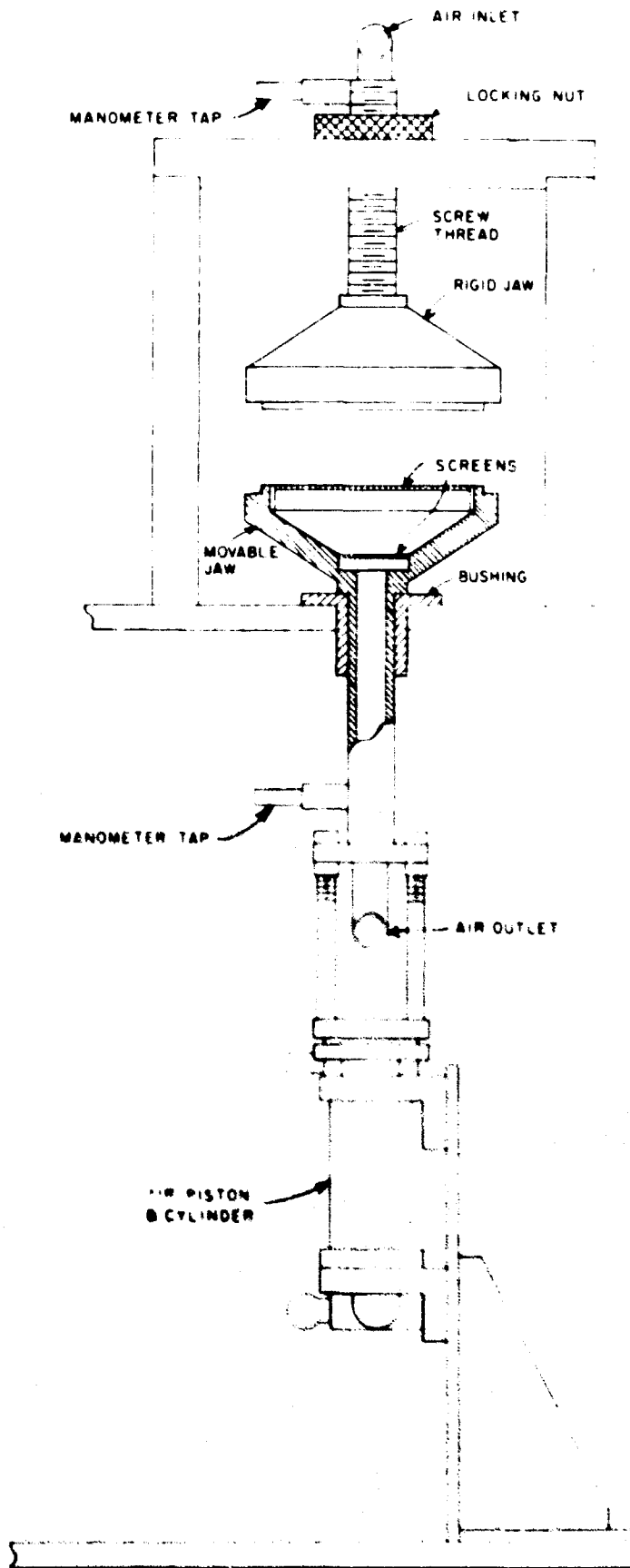
Fig. 5 - Sketch of clamping chuck and air piston.
