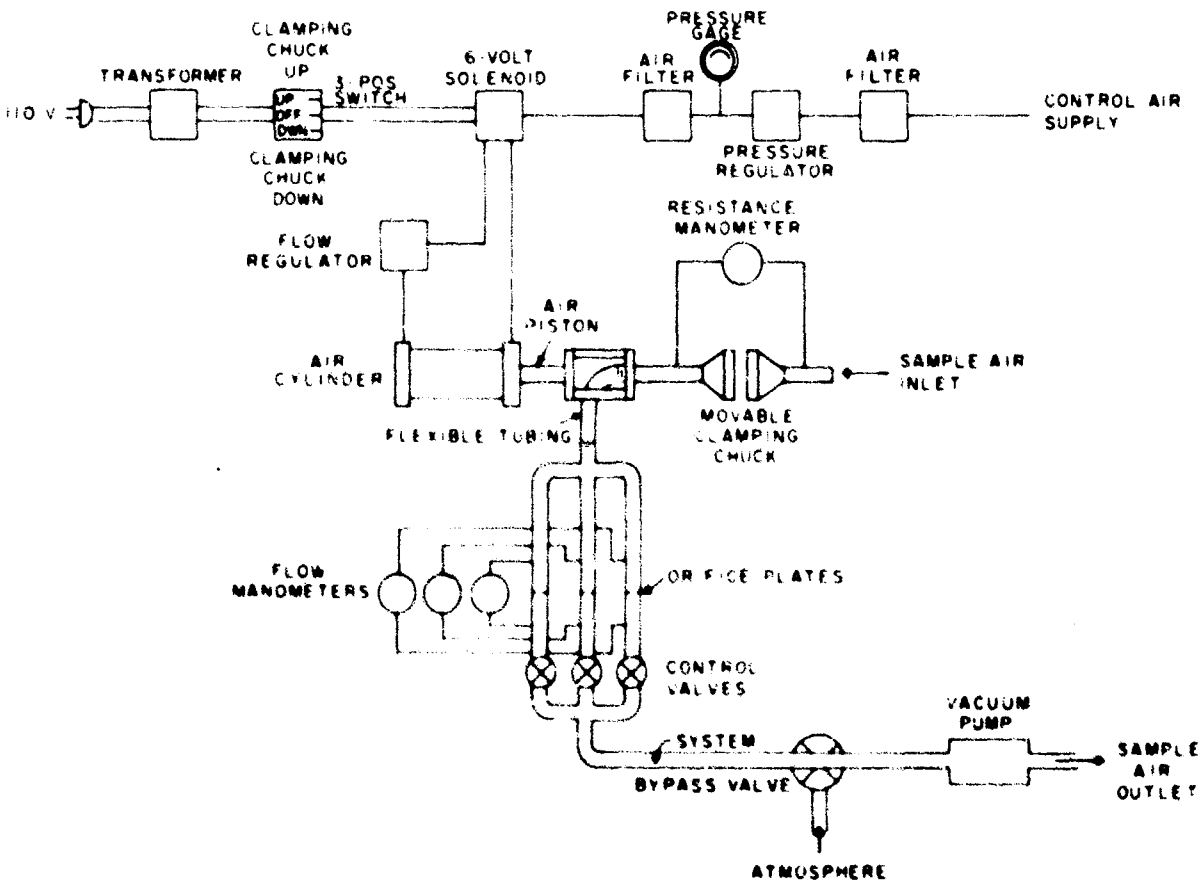
Fig. 3 - Flow diagram of the Air Resistance Meter, Model II
