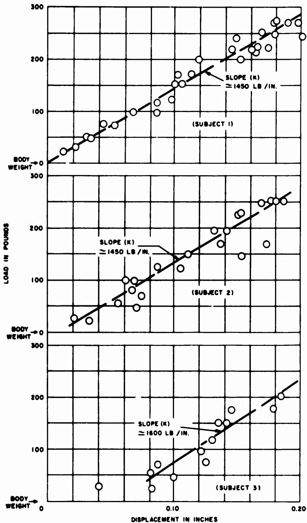
Figure 8 – Deflection of the Iliac Crest under Vertical Load (Note: Initial conditions correspond to the load and displacement due to body weight.)
