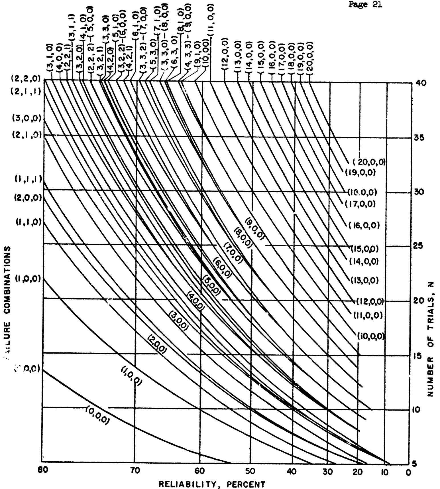
95 PER CENT LOWER CONFIDENCE LIMIT TO TRUE RELIABILITY FOR OBSERVED FAILURE COMBINATIONS OF A THREE-SUBSYSTEM SERIAL SYSTEM WITH N(5 \leq N \leq 40) TRIALS PER SUBSYSTEM (ALL PERMUTATIONS OF FAILURE COMBINATIONS (f_1, f_2, f_3) ARE EQUIVALENT.)
