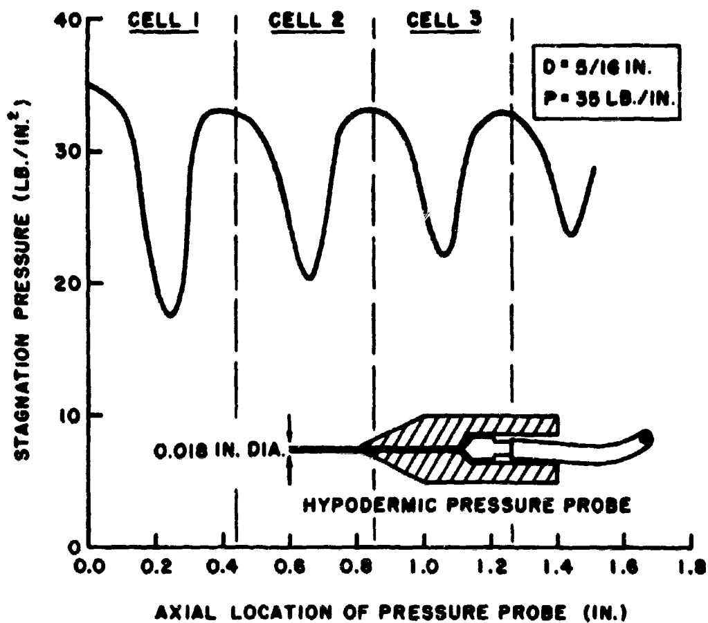
STAGNATION PRESSURE DISTRIBUTION ALONG CHOKED JET AS MEASURED BY FINE PROBE
