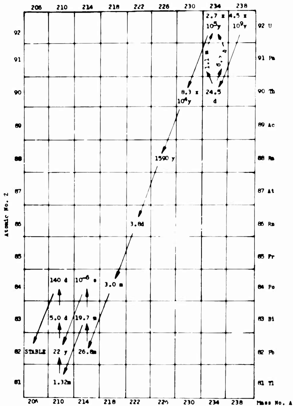
Figure 34. Uranium Decay Series (Half Lives Are Indicated for Each Step)
