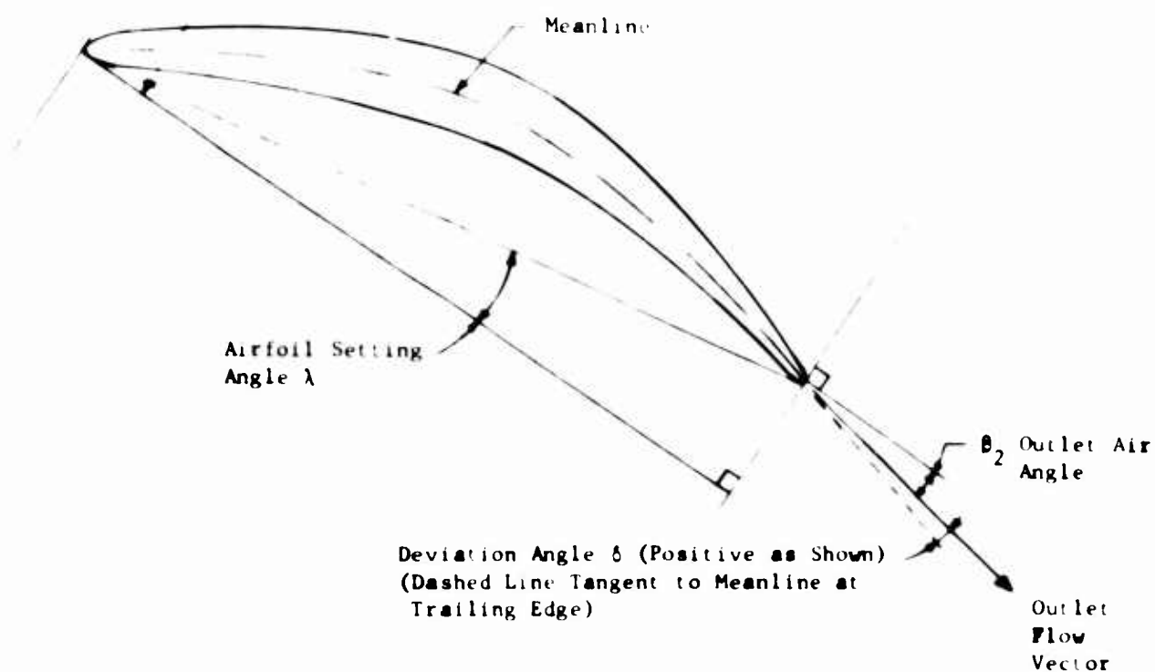
Figure 12. Cascade Geometry Nomenclature.
