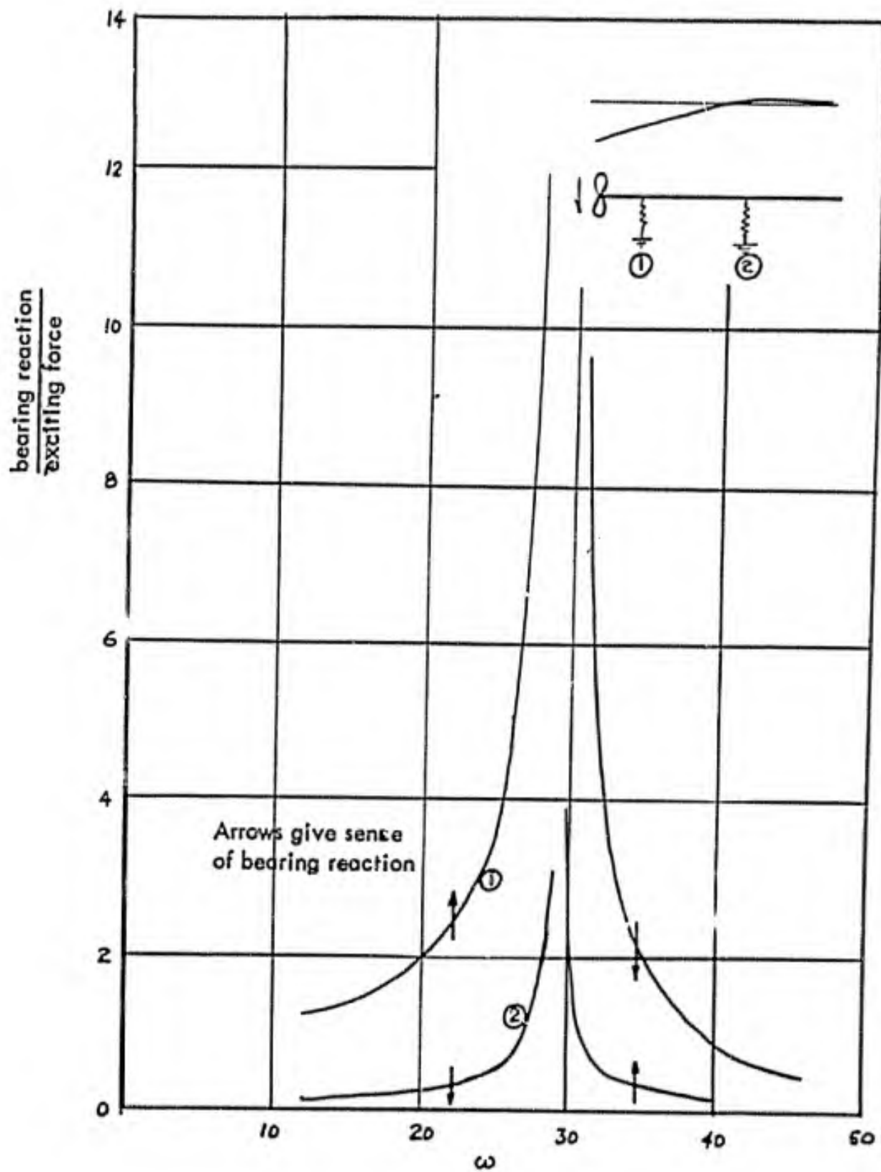
Figure 13 Force reactions at bearings
