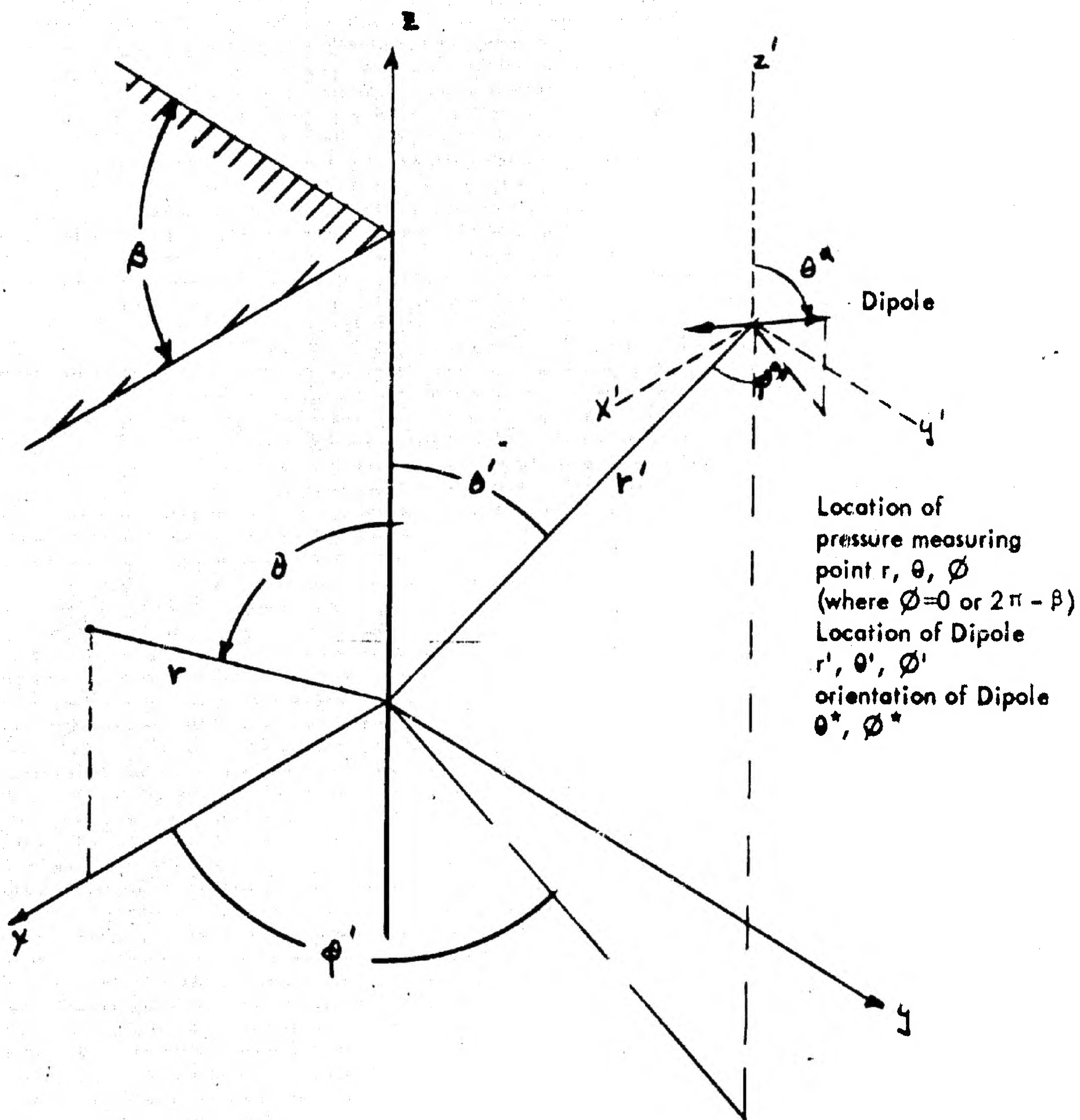
Coordinates in Study of Pressures on a Wedge
