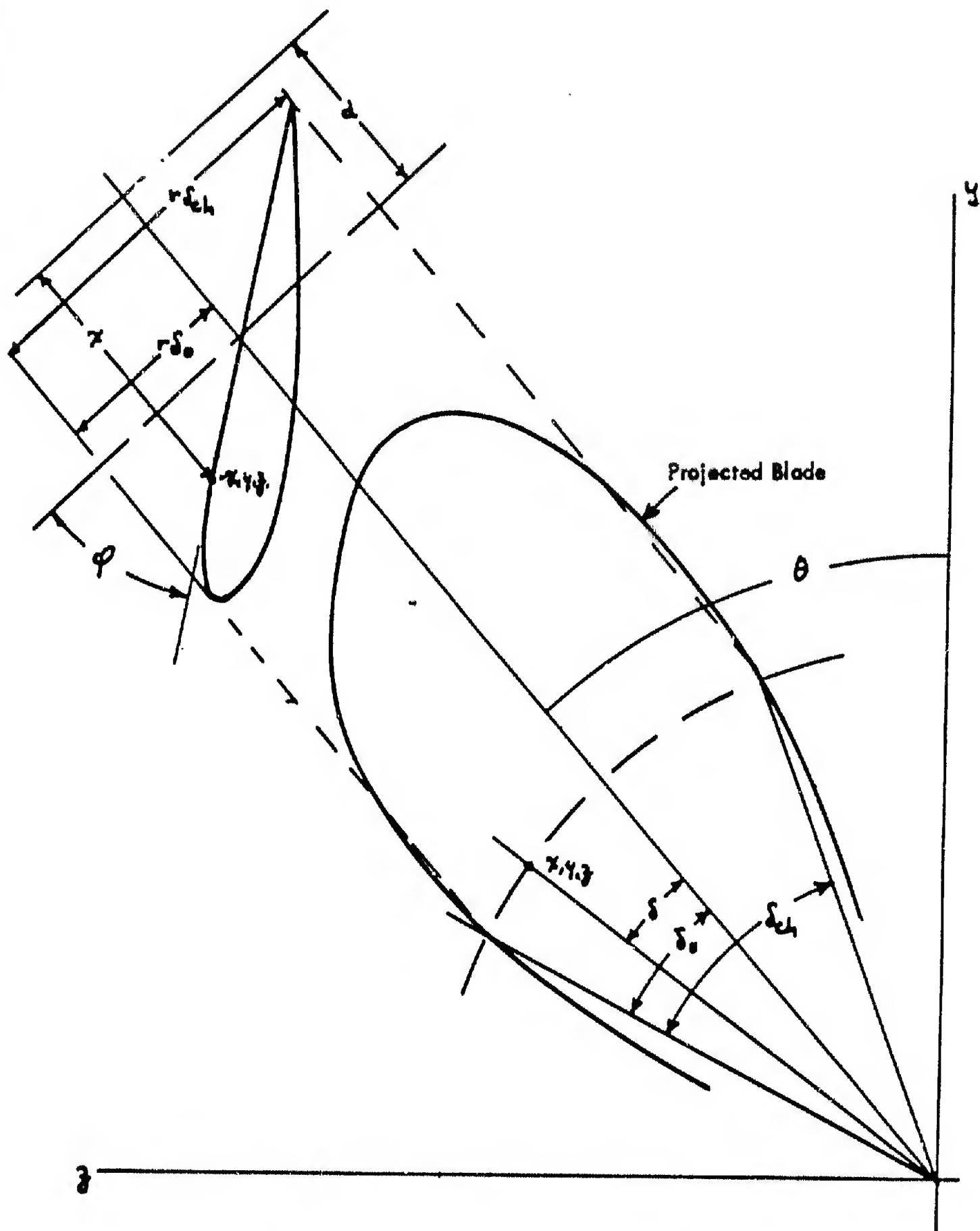
Variables used in Study of Effects of Pitch and Chordwise Lift Distribution on Free-Field Pressures
