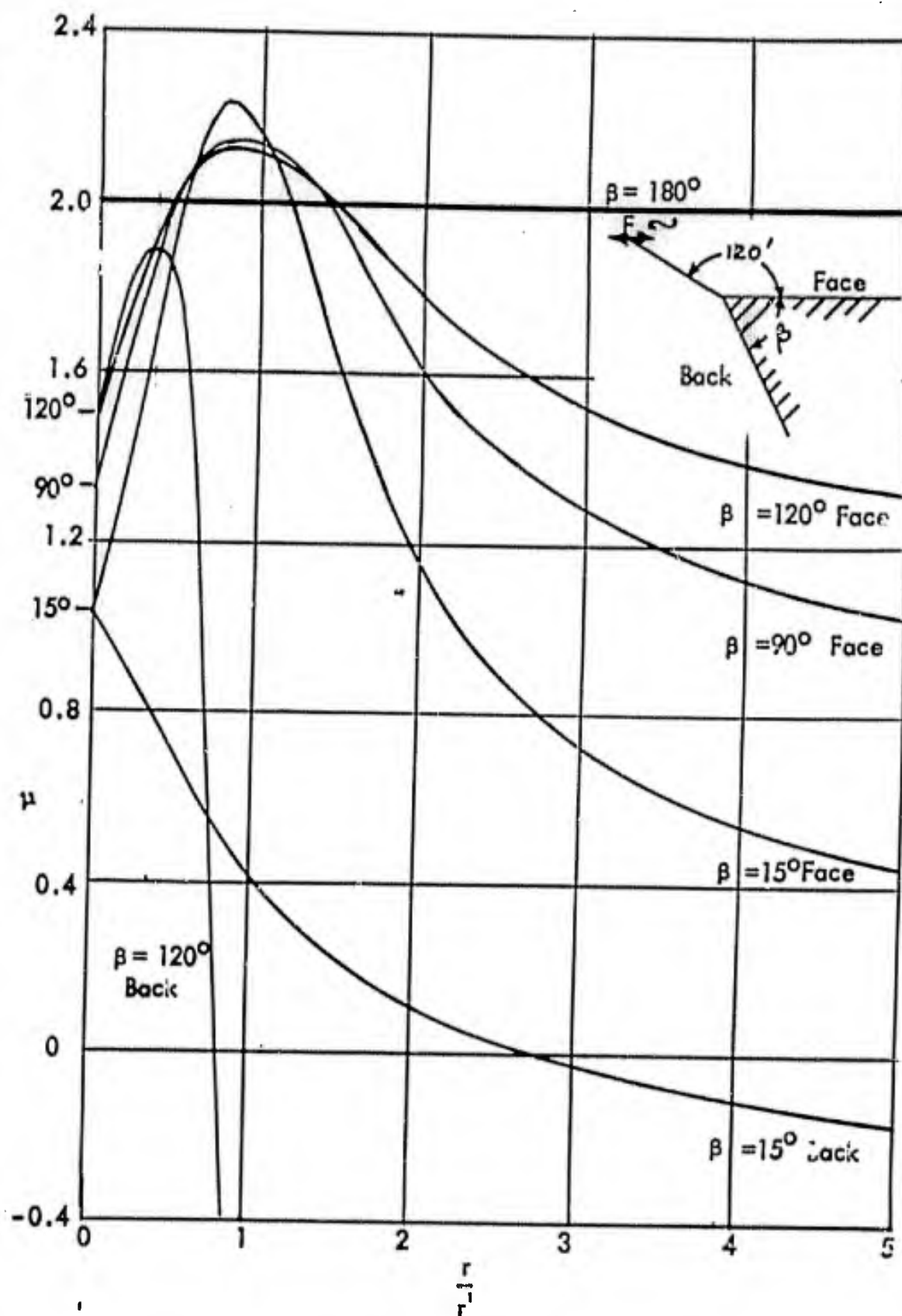
Fig. 10 Pressures on Wedges Caused by a Harmonic Force
