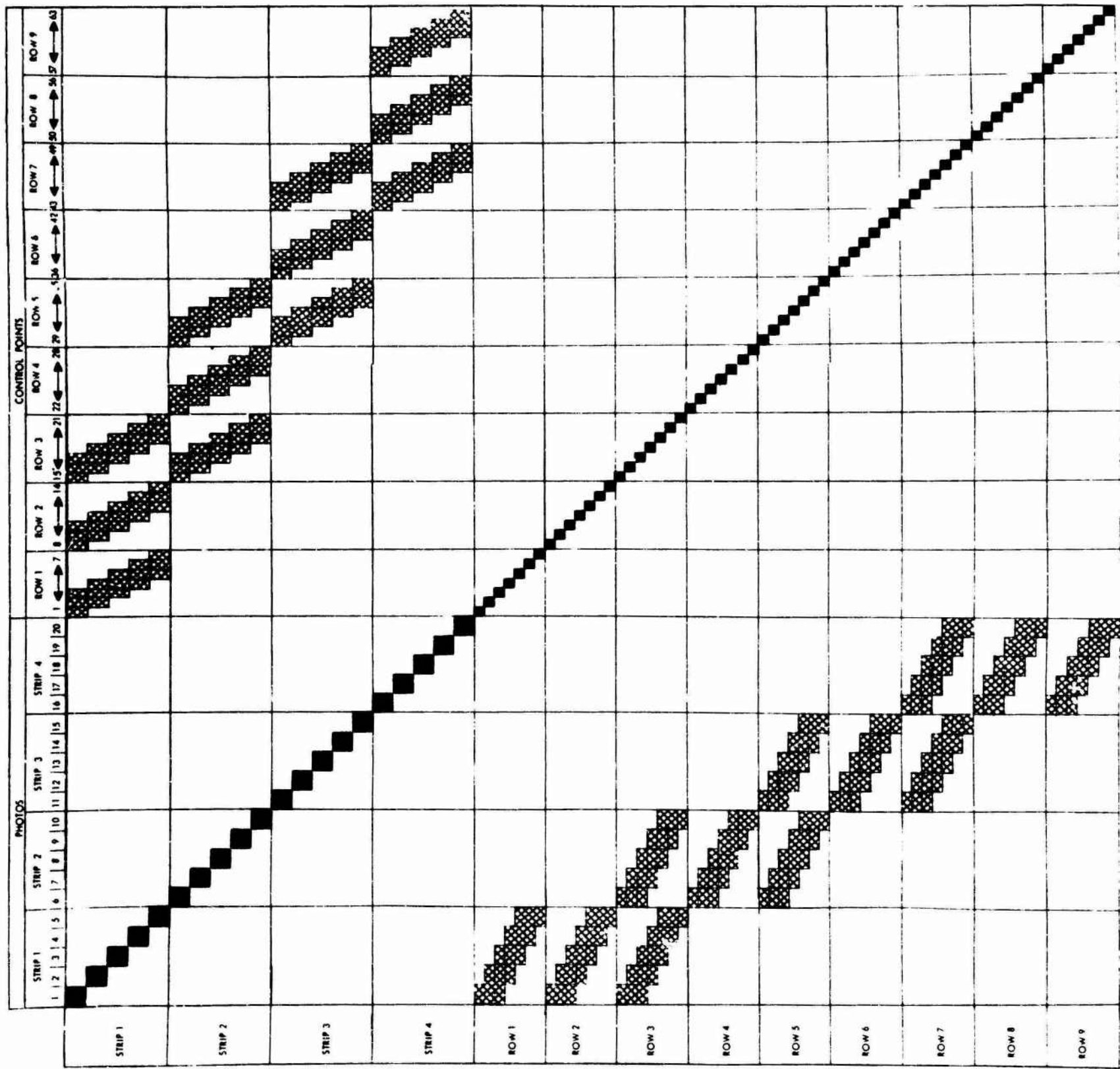
FIGURE 1.2a. FORM OF COEFFICIENT MATRIX GENERATED BY UNIFORM BLOCK WITH POINTS AND PHOTOS NUMBERED AS IN FIG. 1.1. EACH SMALL SQUARE REPRESENTS A 3x3 BLOCK OF ELEMENTS; ORDER OF FULL MATRIX IS 309x309.
