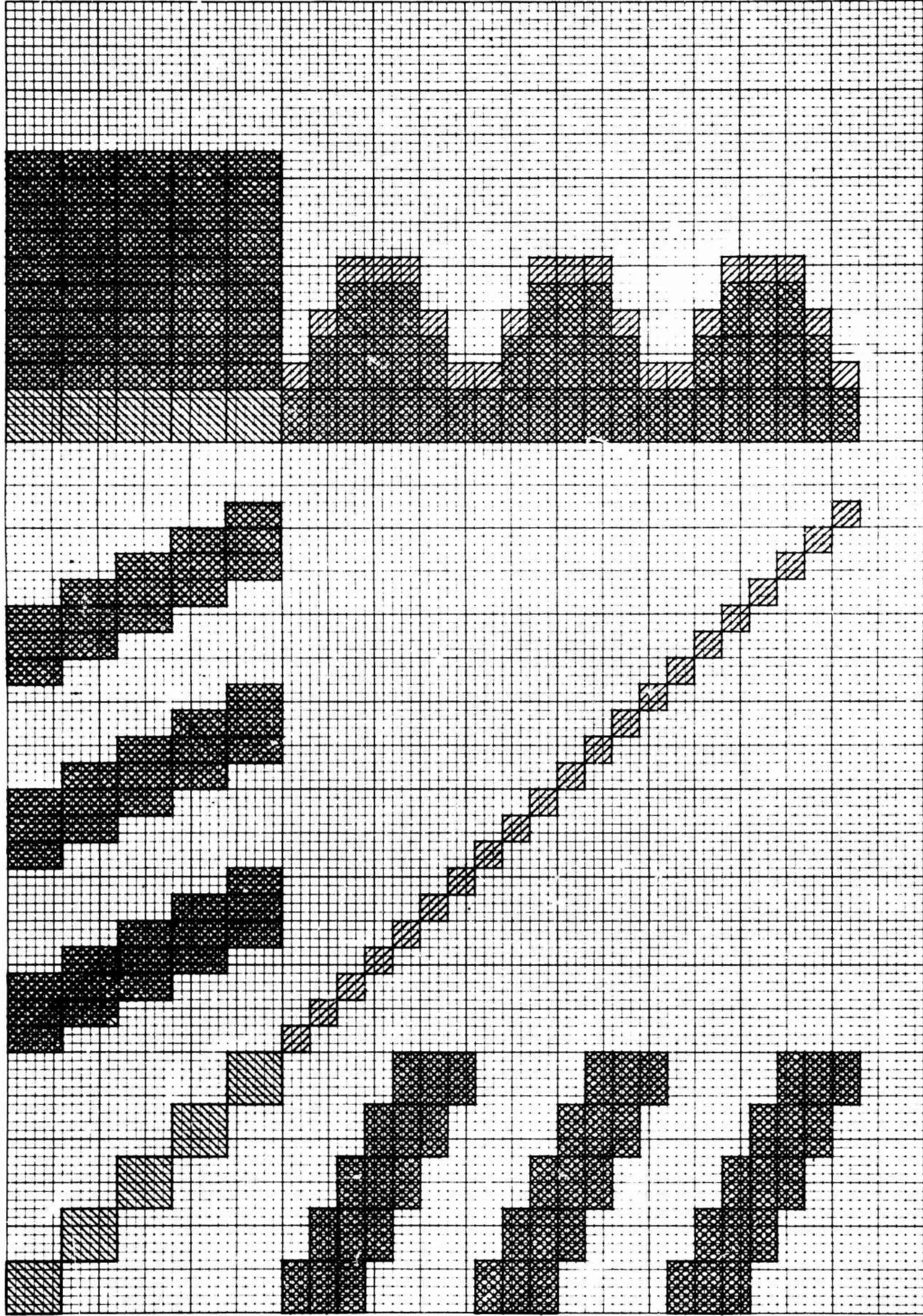
Figure 2.2a. The A form of the coefficient matrix of the general normal equations arising from adjustment of 1x5 strip of photography with photos and control points numbered as in Fig. 2.6.
