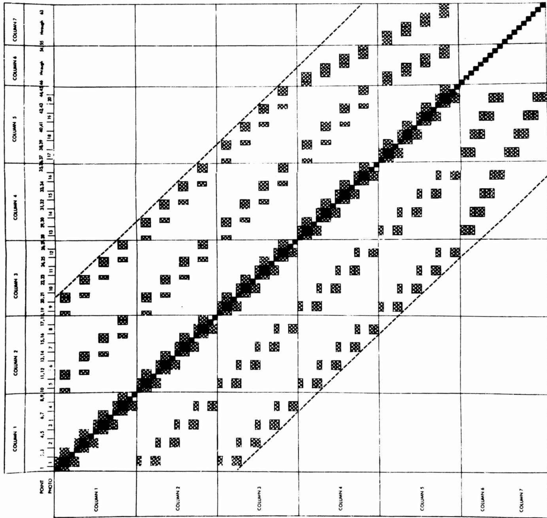
FIGURE 1.5a. EXAMPLE OF INTERMINGLED FORM OF COEFFICIENT MATRIX OF NORMAL EQUATIONS. NUMBERING OF PHOTOS AND CONTROL POINTS CORRESPONDS TO THAT OF FIGURE 1.3.
