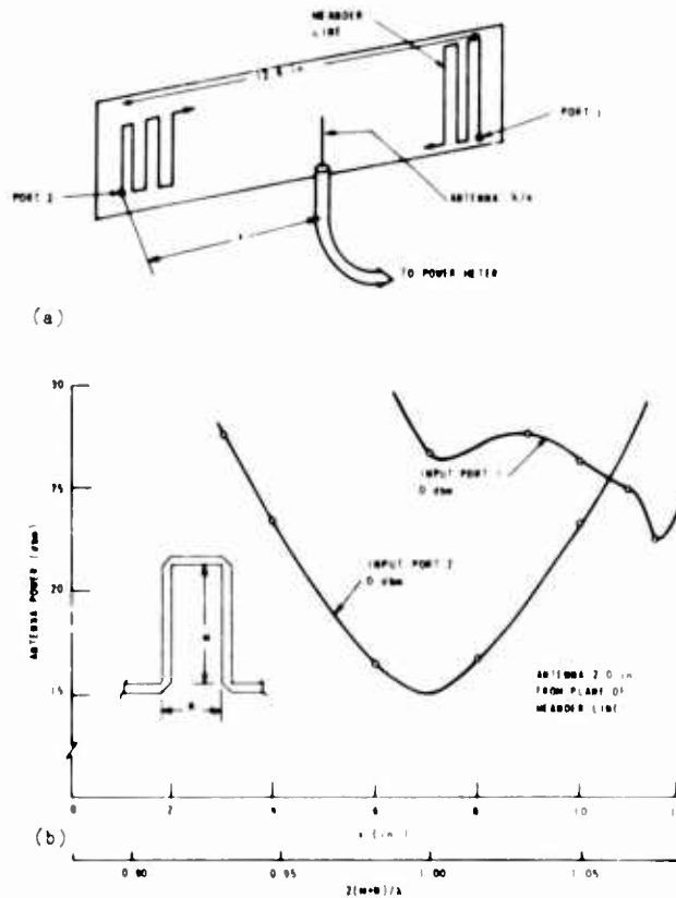
Figure 32. TML Radiation Pattern (a) Radiation Pattern Measurement (b) Power Received By Antenna Vs Distance Along Line and Normalized Wavelength
