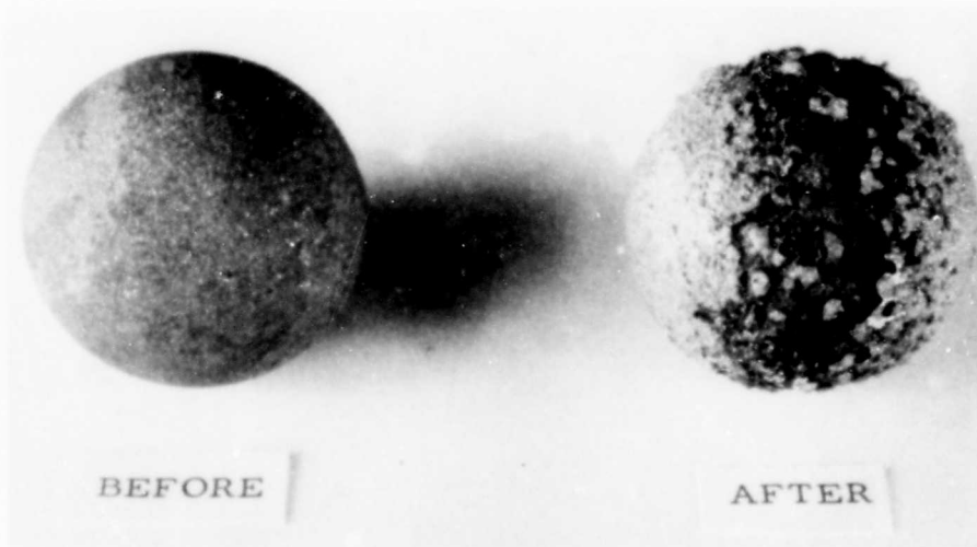
Figure 67. SiC-Coated RVC Graphite Before and After Oxidation at 1700°C
