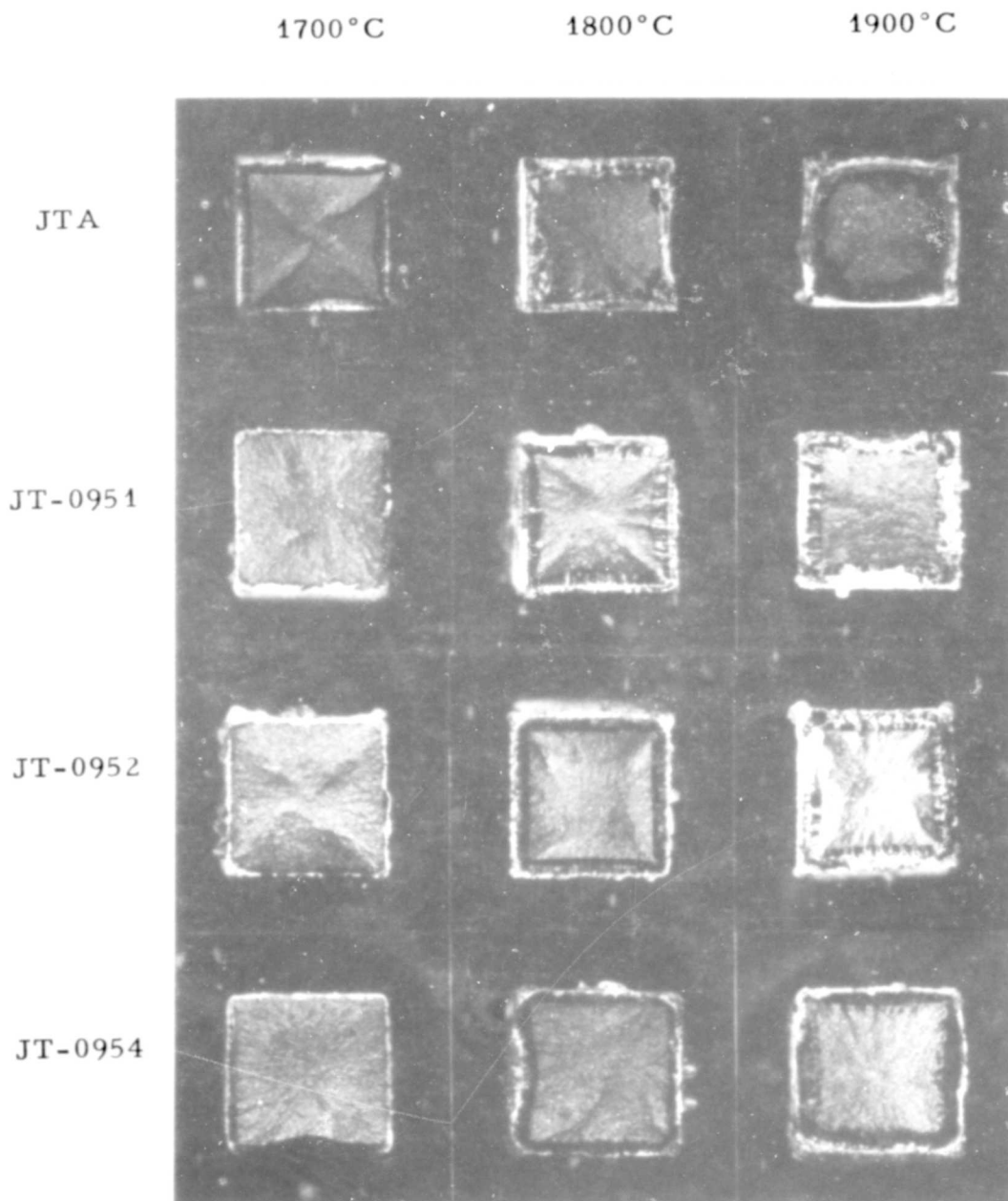
31 Figure 53. The Effect of Replacing Boron by Zirconium in JTA on the Cross Section of Test Samples Exposed for 10 Minutes, Actual Size of Cross Section, \frac{1}{4} Inch by \frac{1}{4} Inch
