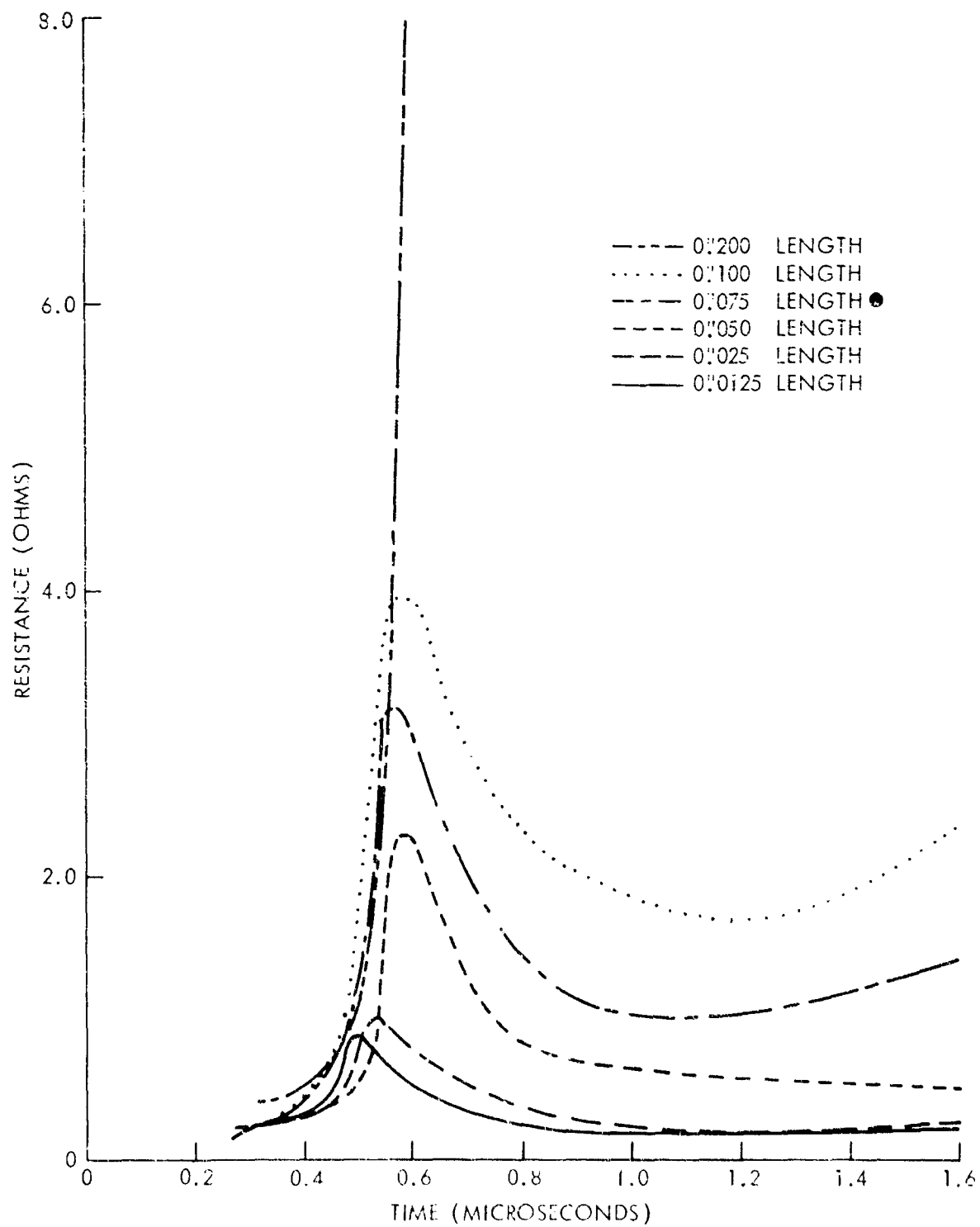
FIG. 11 RESISTANCE AS A FUNCTION OF TIME FOR VARIOUS LENGTHS OF 2-MIL DIAMETER ALUMINUM WIRE
