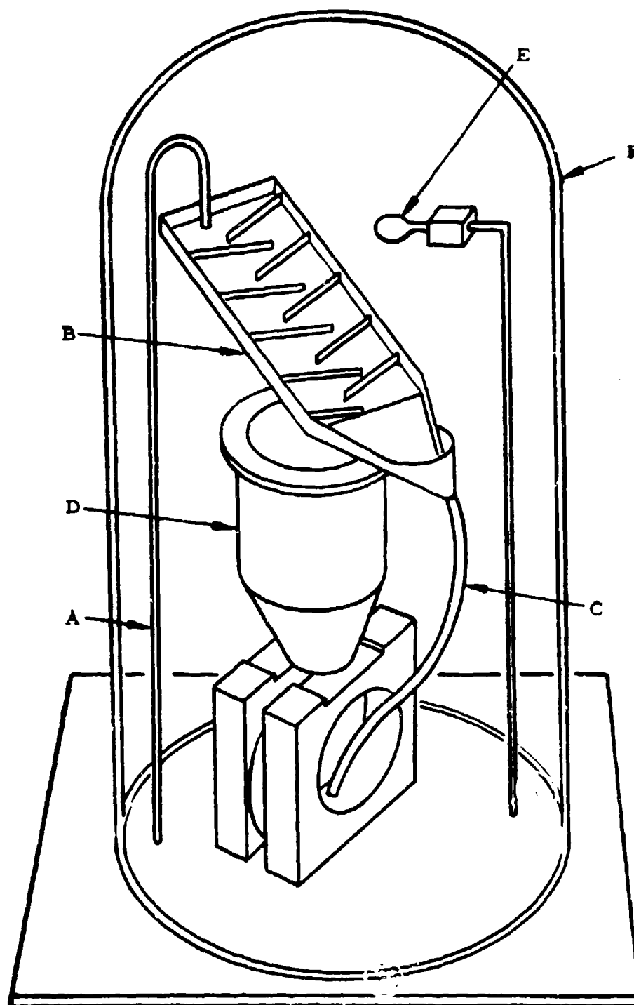
Figure B-2. Apparatus for Vacuum Pouring of Epoxy
