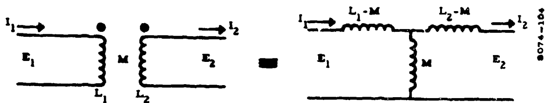
Figure K-1. Transformer and Its Equivalent Circuit
