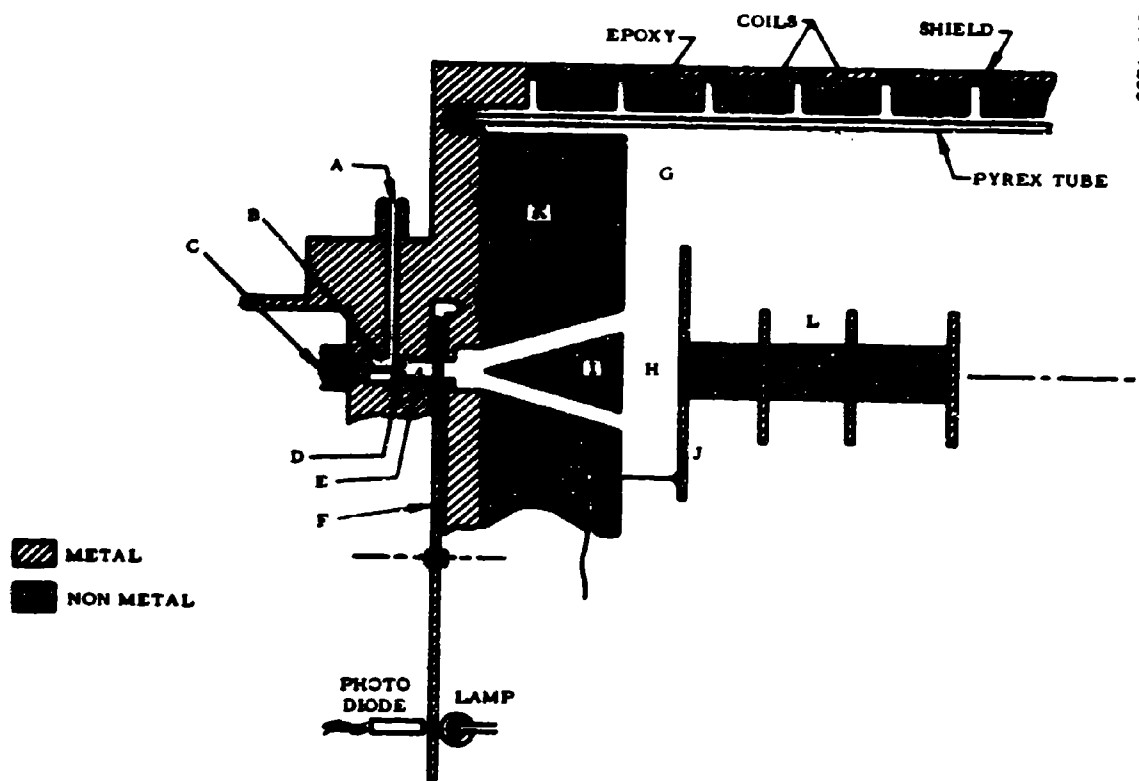
Figure 2-9. Gas Injector
