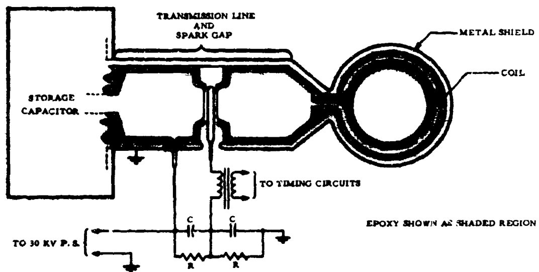
Figure B-1. Coil-Capacitor Assembly
