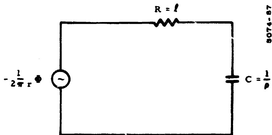
Figure 3-11. An Alternative Electrical Analog for Plasma
