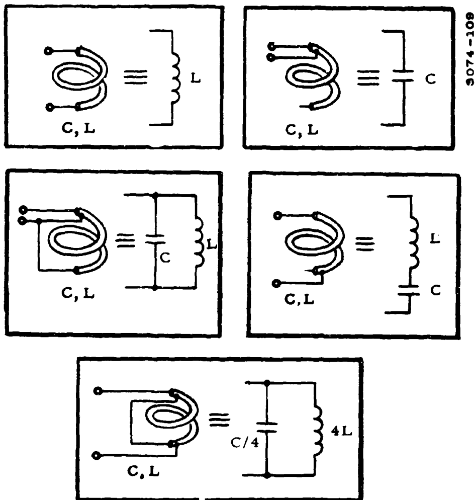
Figure K-6. Possible Connections of a Helix of Coaxial Cable
