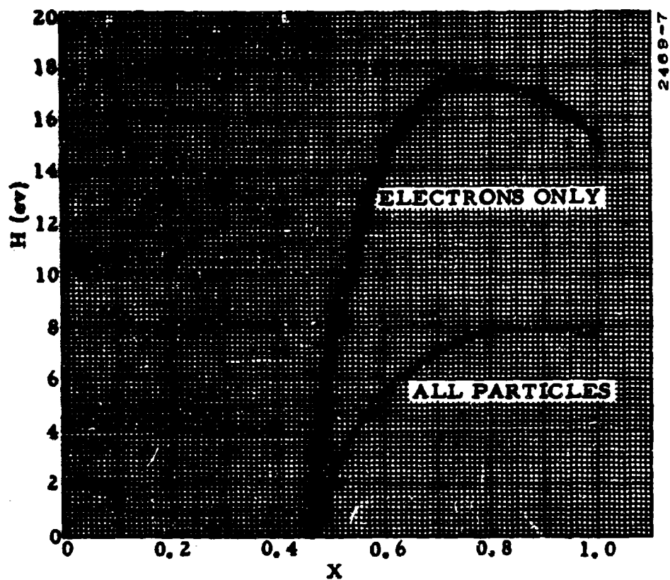
Figure 2-5. Plot of Heat Energy vs Fraction of Ionized Molecules
