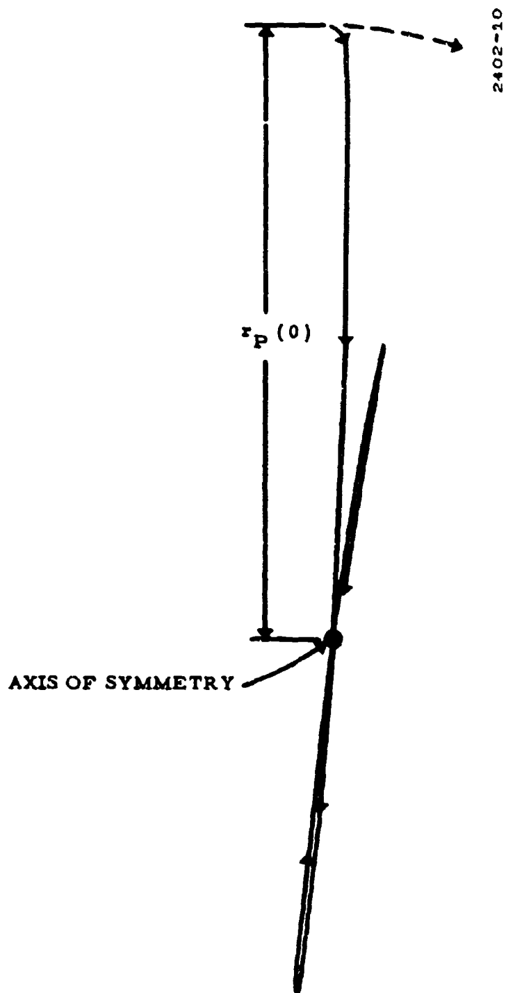
Figure 2. Motion in A Uniform Field
