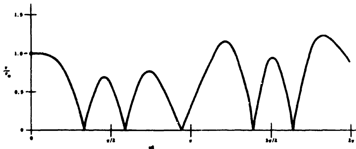
Figure 3. Motion in a Uniform Field, \lambda = 1/4 , \phi(0) = 0
