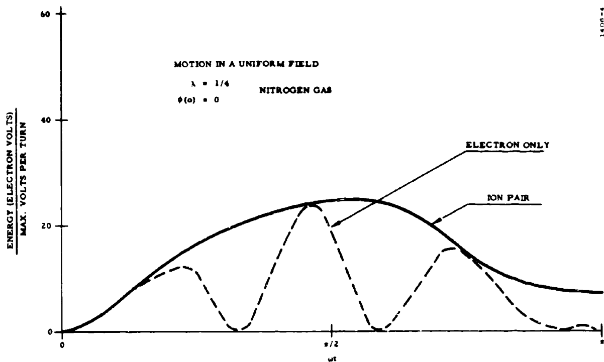
Figure 4. Motion in a Uniform Field, \lambda = 1/4 , \phi(o) = 0 (Energy Plot)
