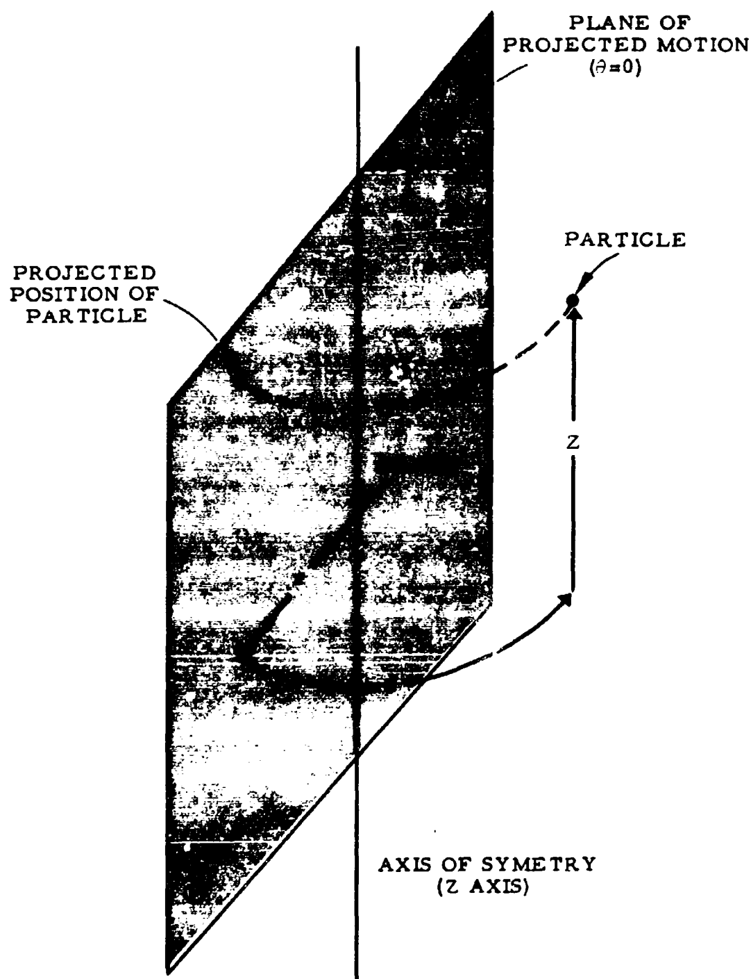
Figure 1. Diagram to Define the Plane of Projected Motion
