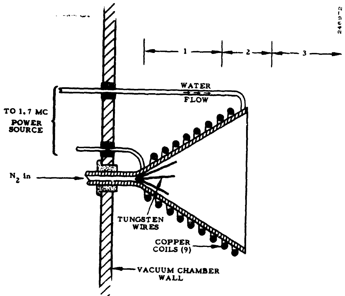
Figure 2-1. Schematic Description of Accelerator
