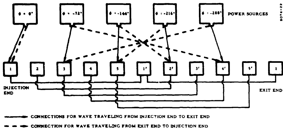
Figure 4-13. Outer Coil Phasing
