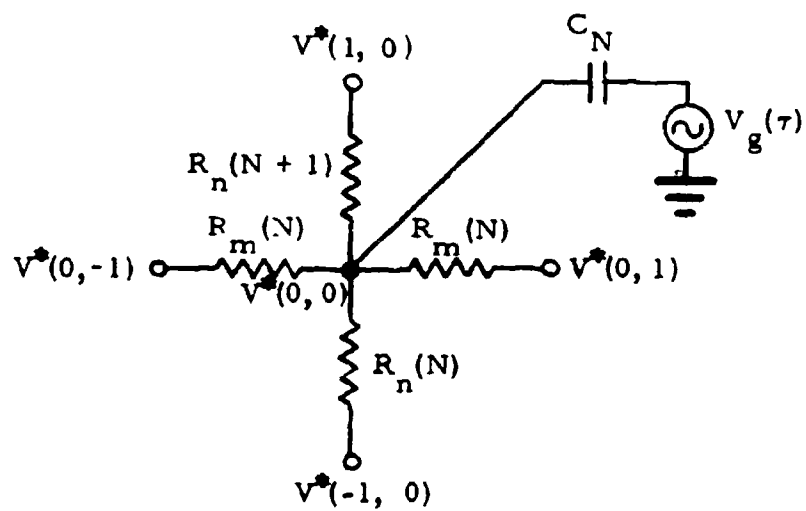
Figure G-6. Constant-Voltage Analog
