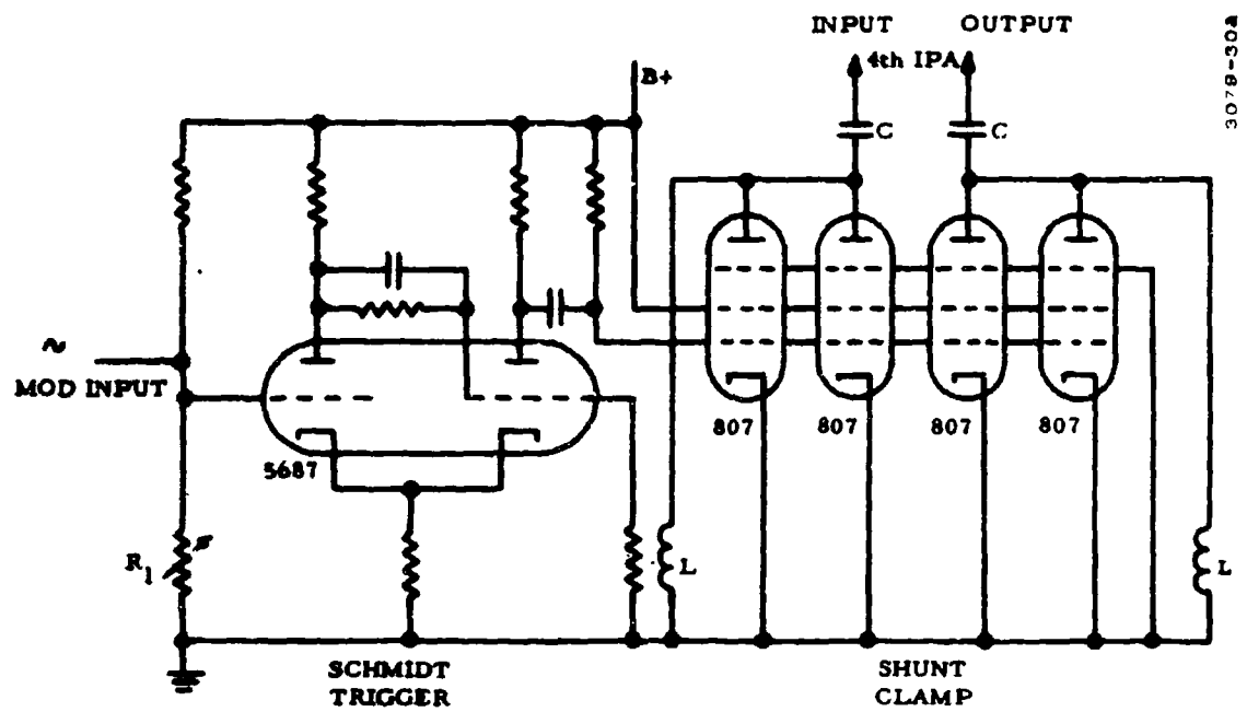
Figure I-7. Shunt Modulator
