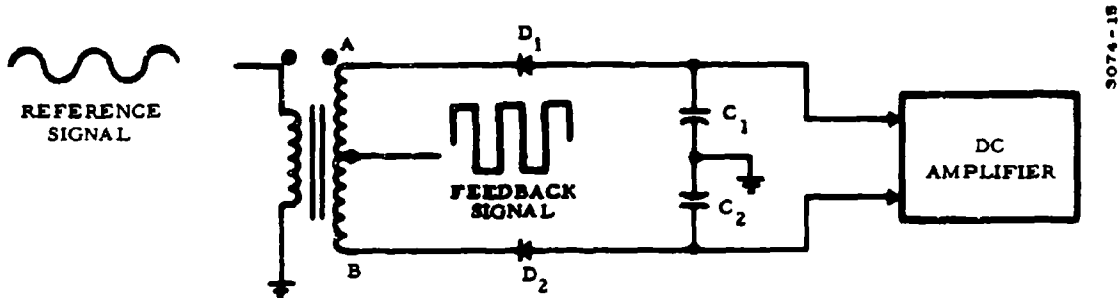
Figure J-3. Phase Detector
