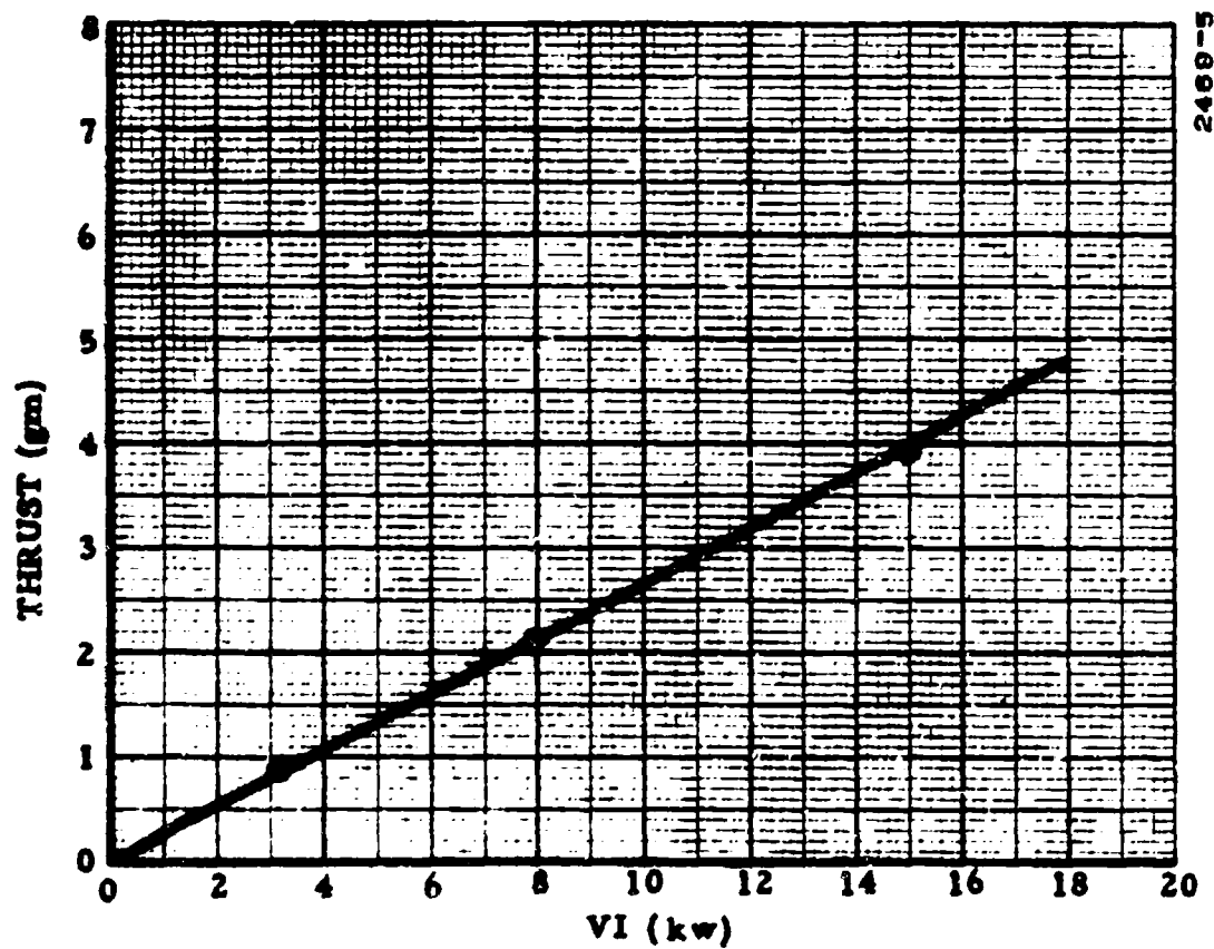
Figure 2-4. Plot of Measured Thrust vs Voltage - Current Product
