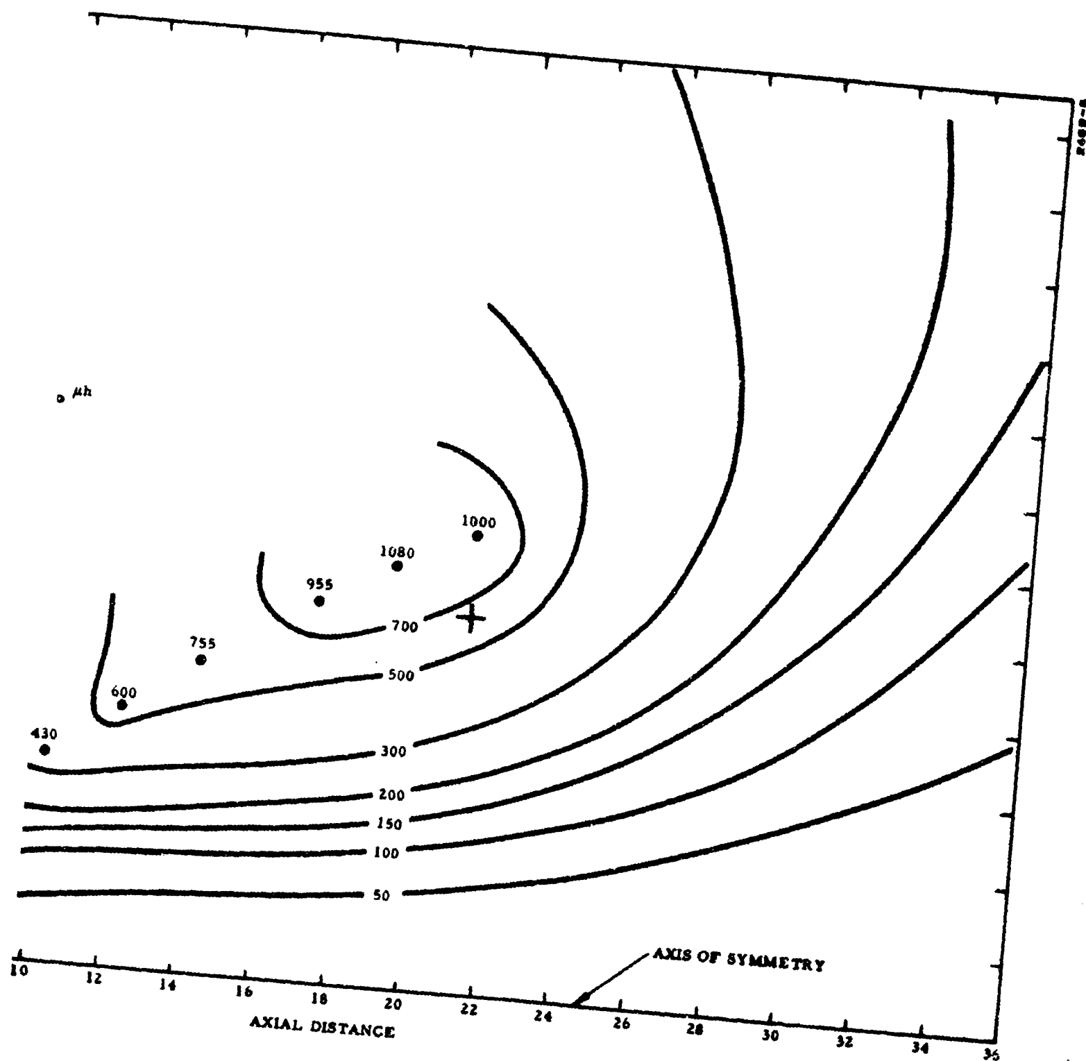
Figure 3-1. Magnetic Field Pattern
