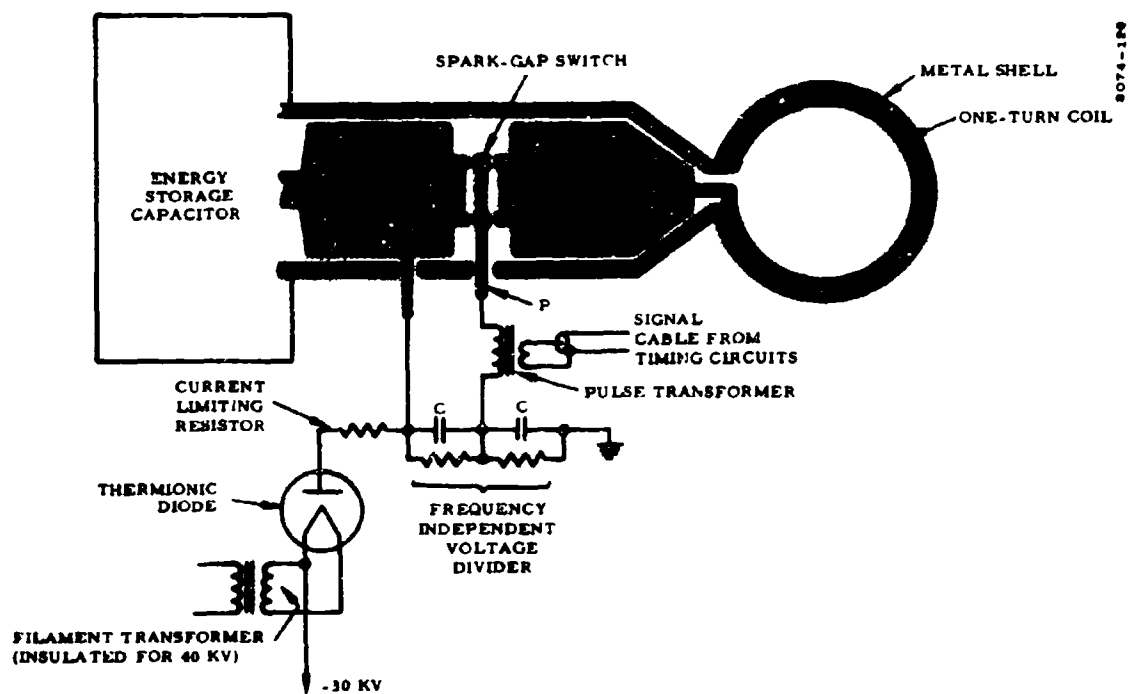
Figure A-2. Cross-Sectional Sketch of One Coil-Capacitor Assembly
