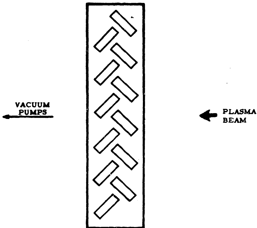
Figure H-12. Schematic of Beam Stop
