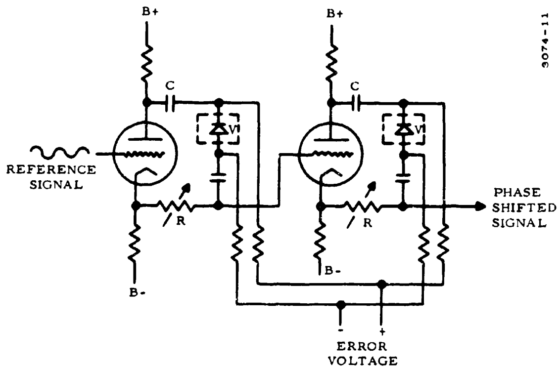
Figure J-7. Phase-Shifting Circuit
