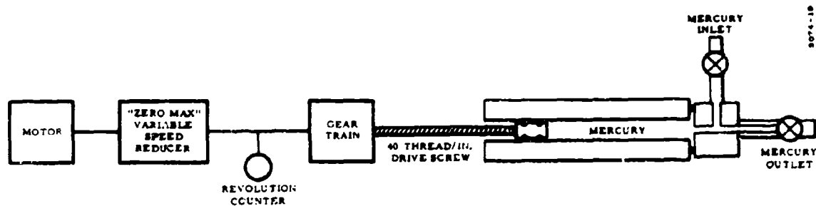
Figure H-19. Schematic of Mercury System
