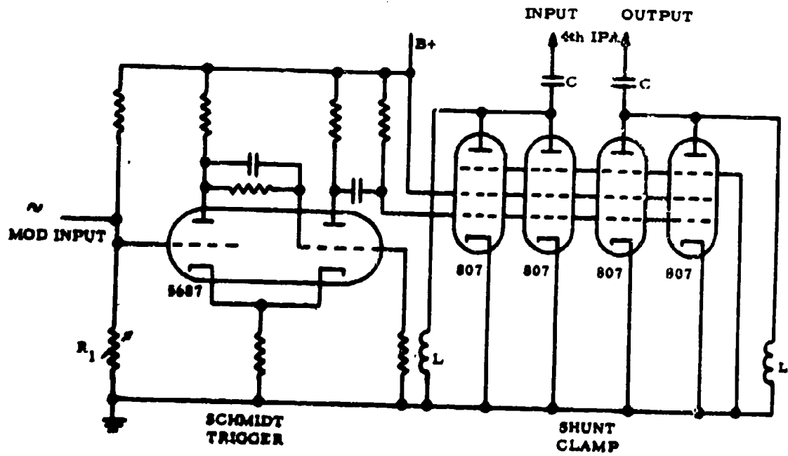
Figure I-7. Shunt Modulator
