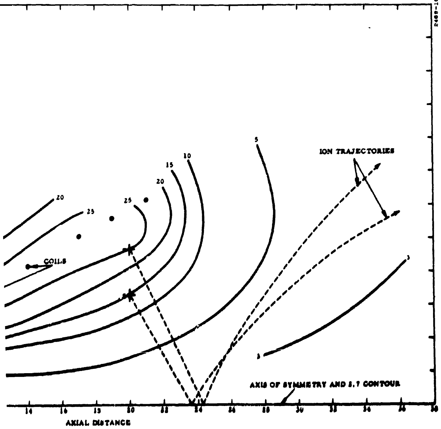
Figure 3-4, Plot of Potential Without E^1 Term
