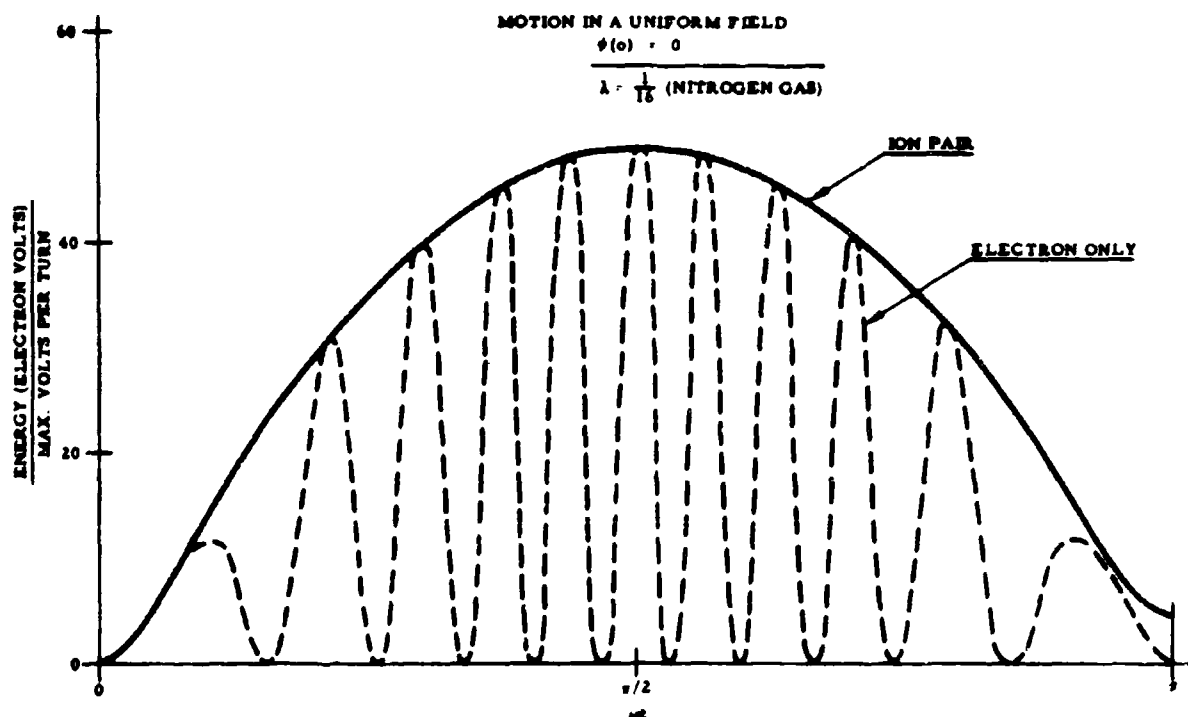
Figure 2. Motion in a Uniform Field, \lambda = 1/16 , \phi(o) = 0 (Energy Plot)
