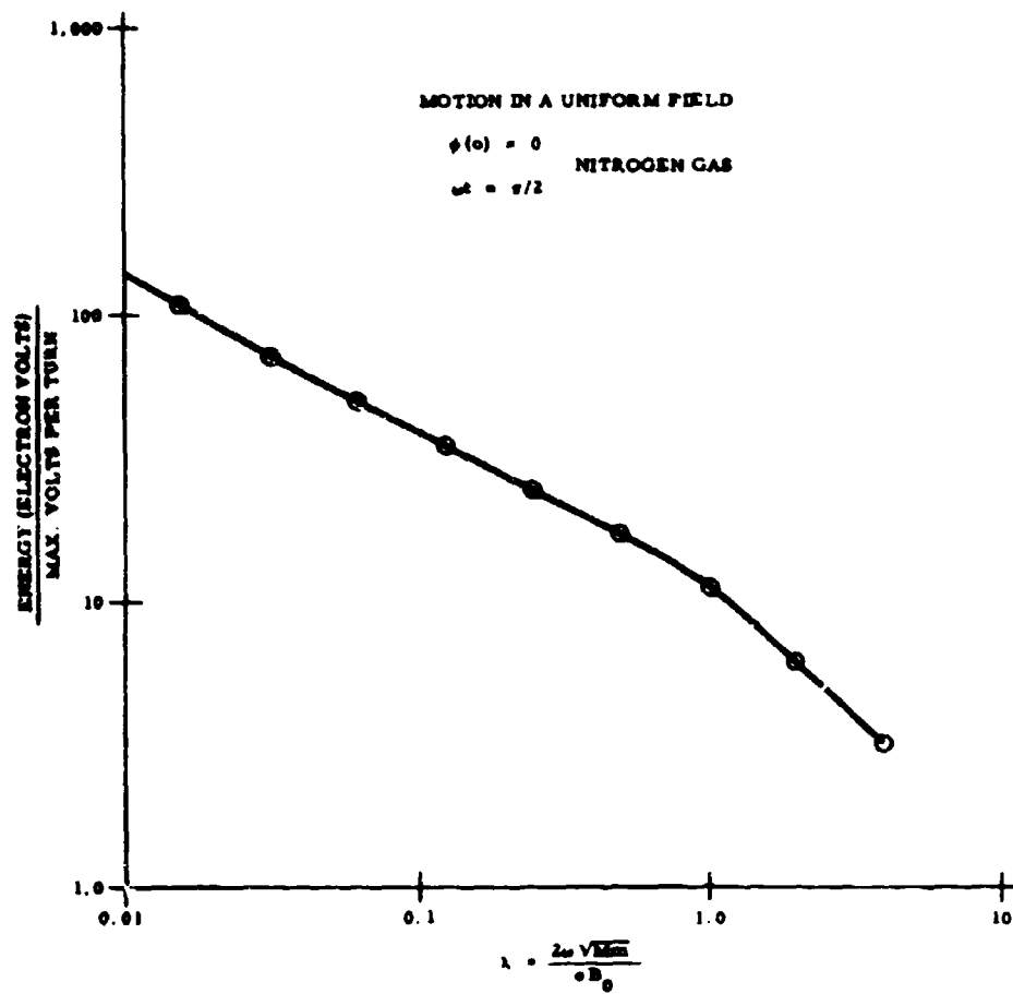
Figure 5. Summary of Computer Runs for Various Value of \lambda
