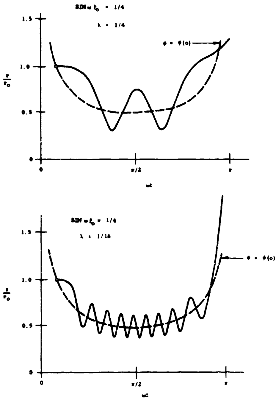
Figure 6. Motion in a Uniform Field, \lambda = 1/4 , \sin \omega t_0 = 1/4 ; \lambda = 1/16 , \sin \omega t_0 = 1/4
