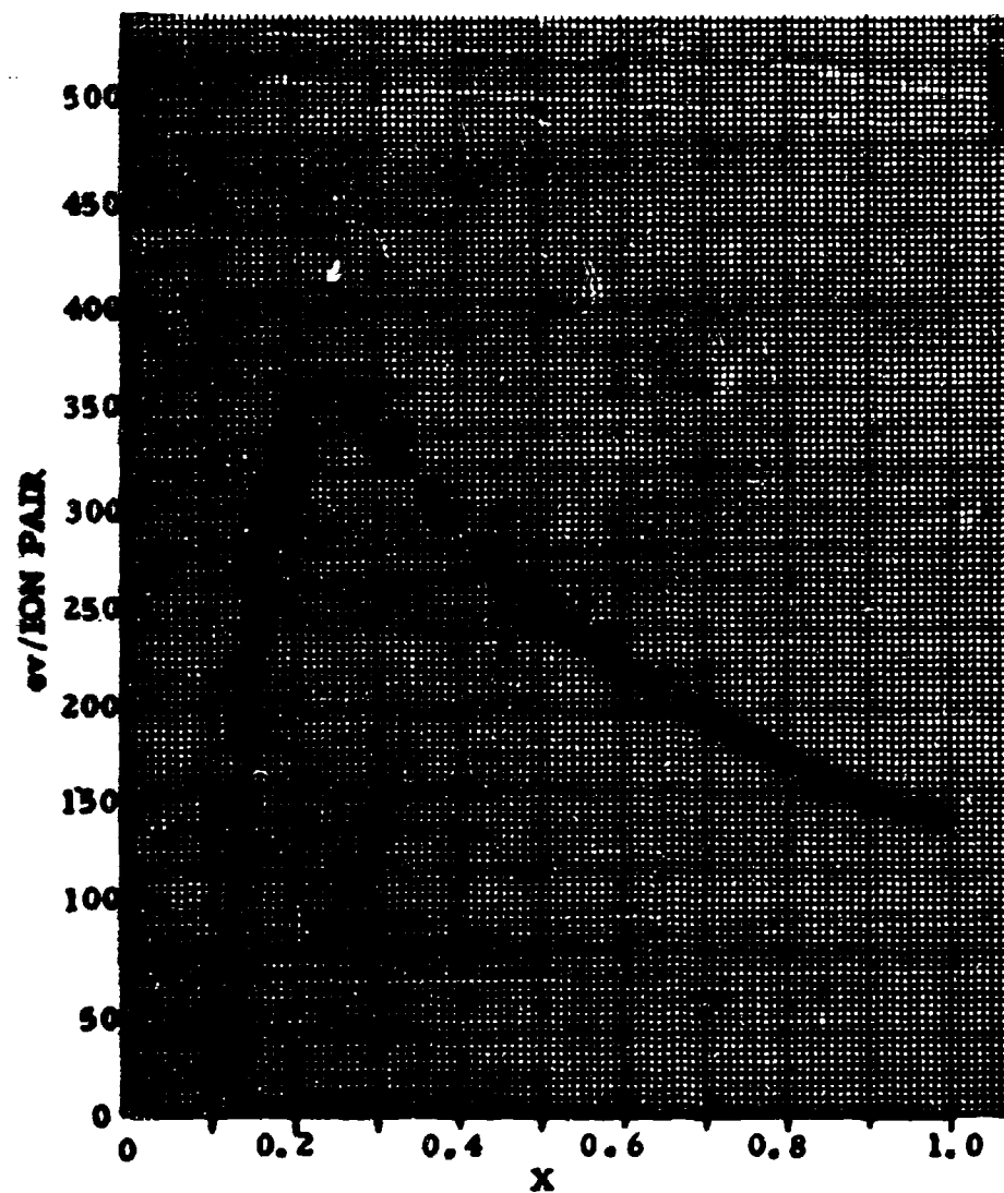
Figure 2-6. Plot of Energy vs Fraction of Ionized Molecules
