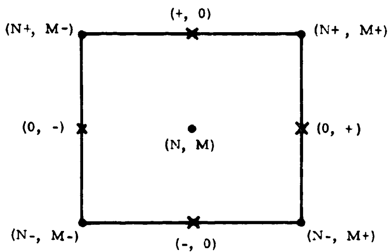
Figure G-2. Power Series Expansion Points
