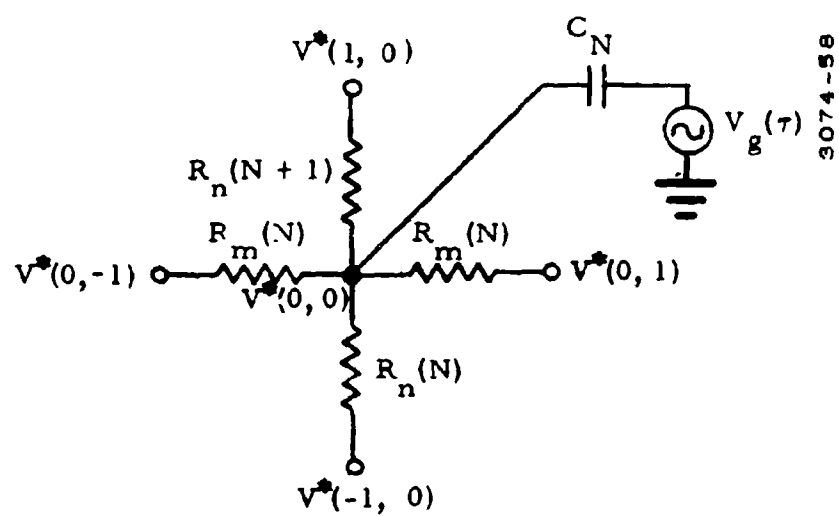
Figure G-6. Constant-Voltage Analog
