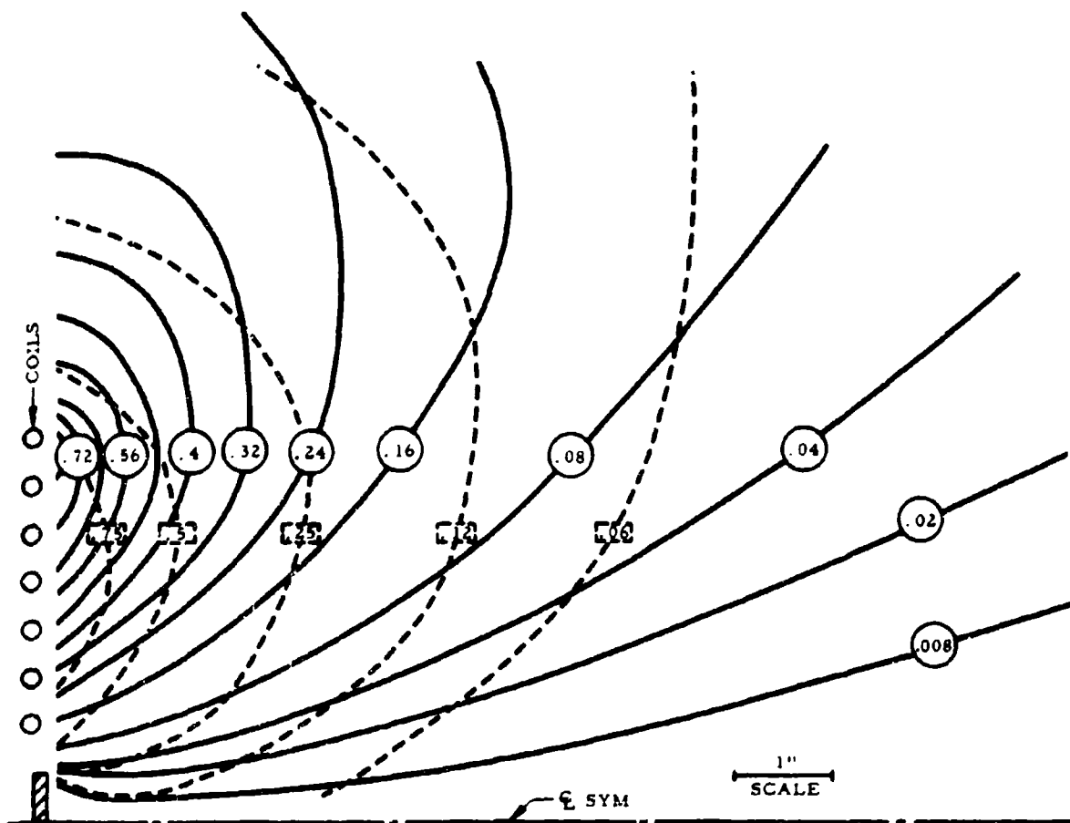
Figure 7. An Inductive Potential Pattern for a Set of Coils
