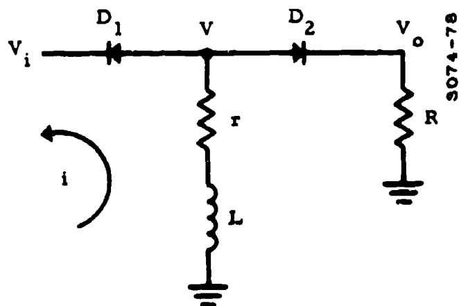
Figure J-13. Circuit to Illustrate Operation of Phase Display
