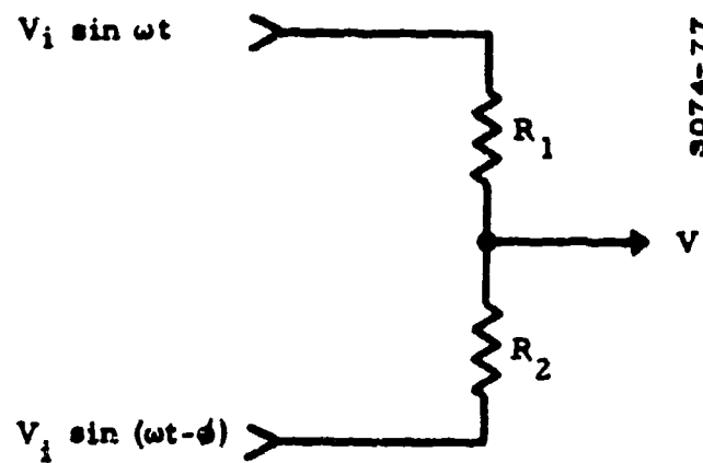
Figure J-9. Matrix Element of Phase Generator
