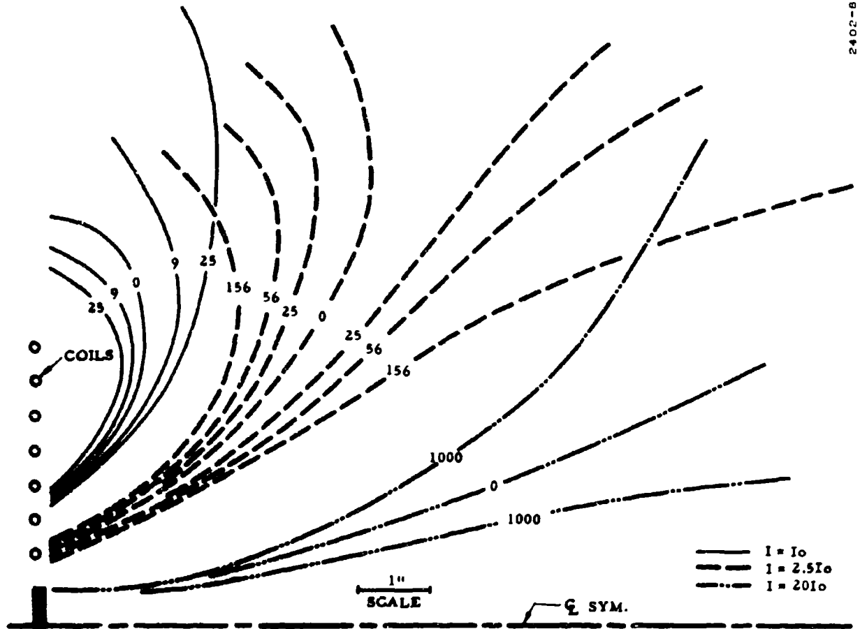
Figure 8. An Inductive Potential Pattern for a Set of Coils
