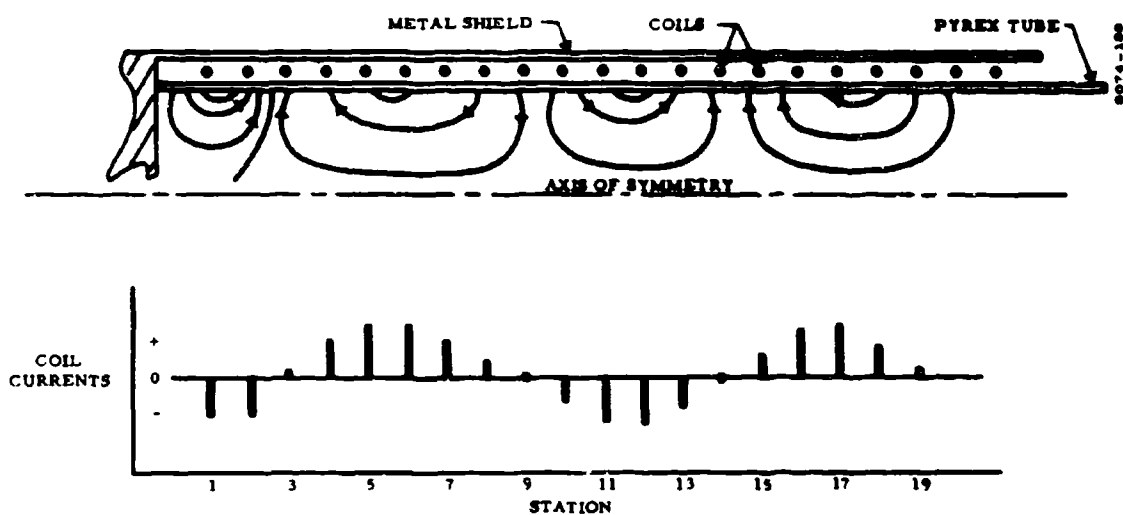
Figure 2-5. Top: Sketch of Magnetic Field Pattern Bottom: Coil Currents at 9 \mu sec.
