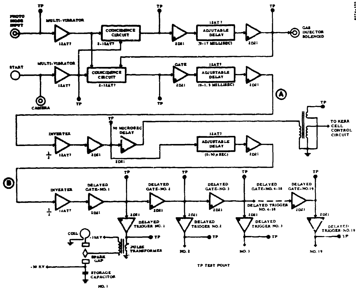
Figure A-6. Schematic of Timing and Control Circuit
