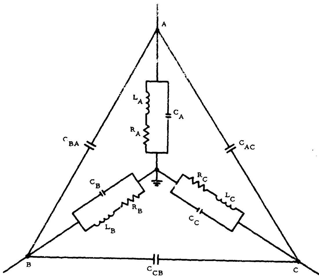
Figure L-1. Ring Circuit
