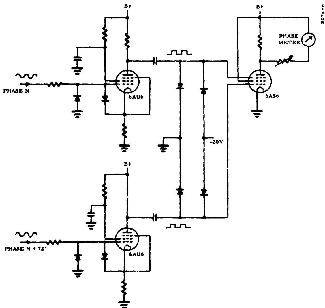
Figure J-11. Phase-Monitoring Circuit
