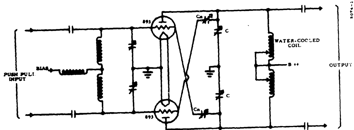
Figure I-1. Simplified Schematic of TBC Power Amplifier (Unmodified)
