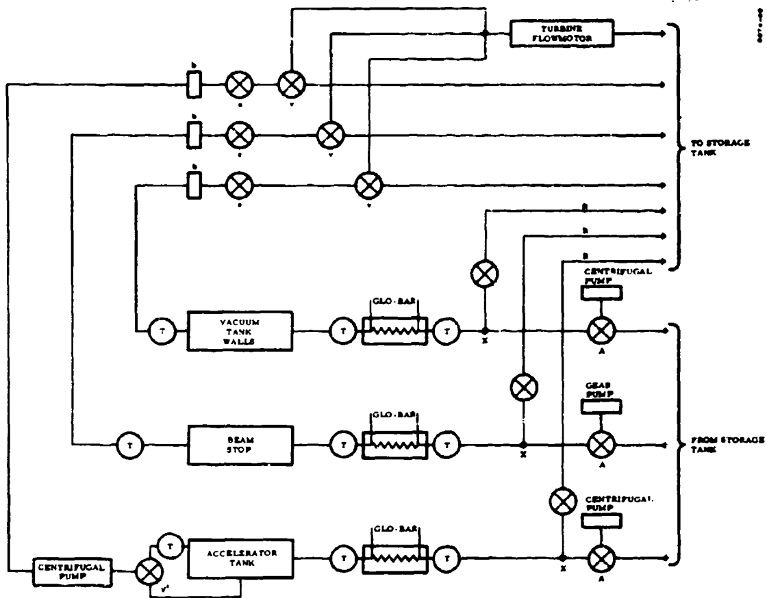
Figure H-14. Schematic of Cooling System
