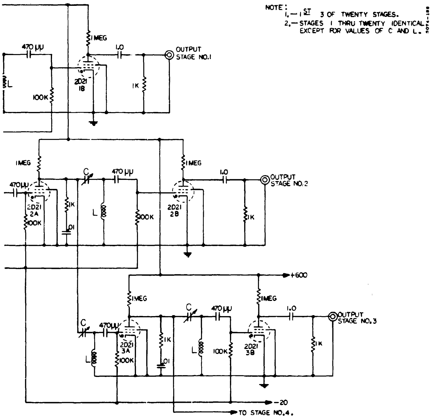
Figure A-9. Schematic of Trigger Circuits
