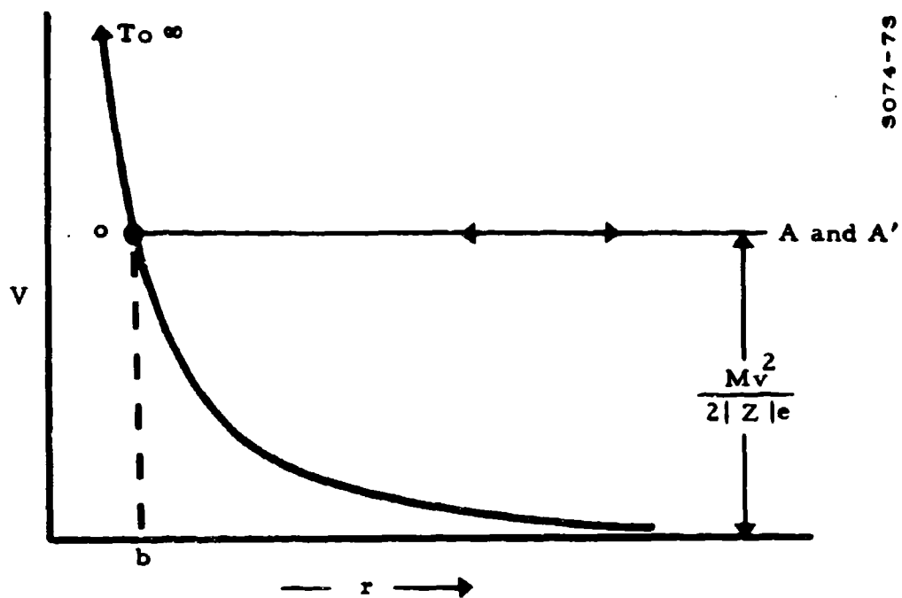
Figure 3-2. Inductive Potential Representation of Straight-Line Motion
