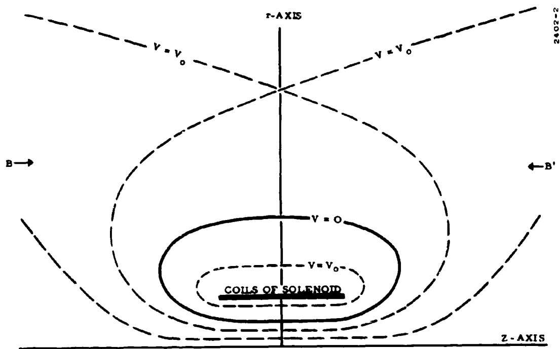
Figure 2. An Inductive Potential Pattern for a Solenoid
