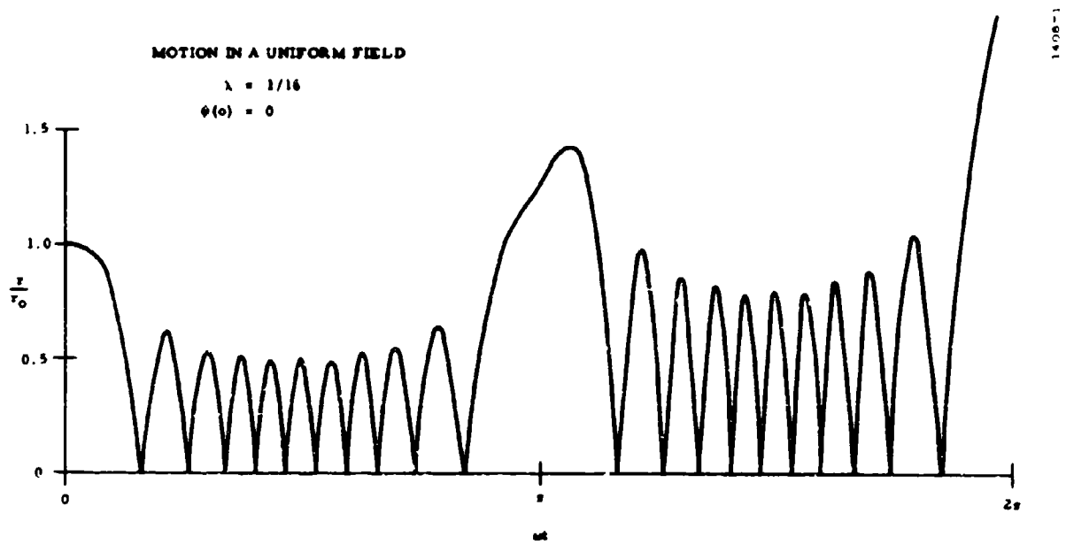
Figure 1. Motion in a Uniform Field, \lambda = 1/16 , \phi(0) = 0
