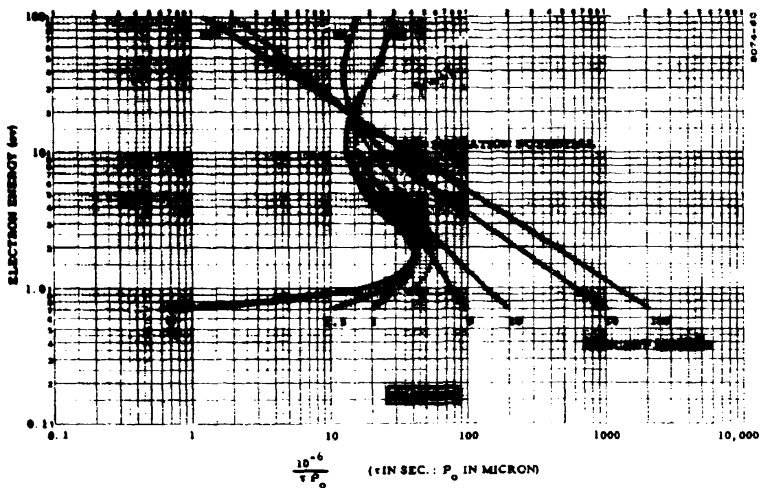
Figure 3-6. Graph for Determining Electron Collision Time in Mercury Gas
