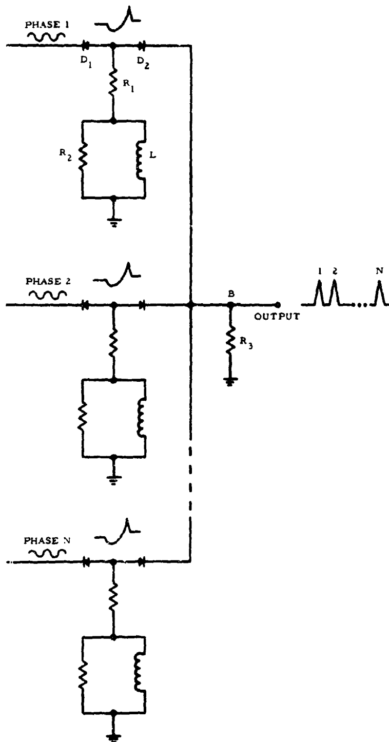
Figure J-12. Multiphase Display
