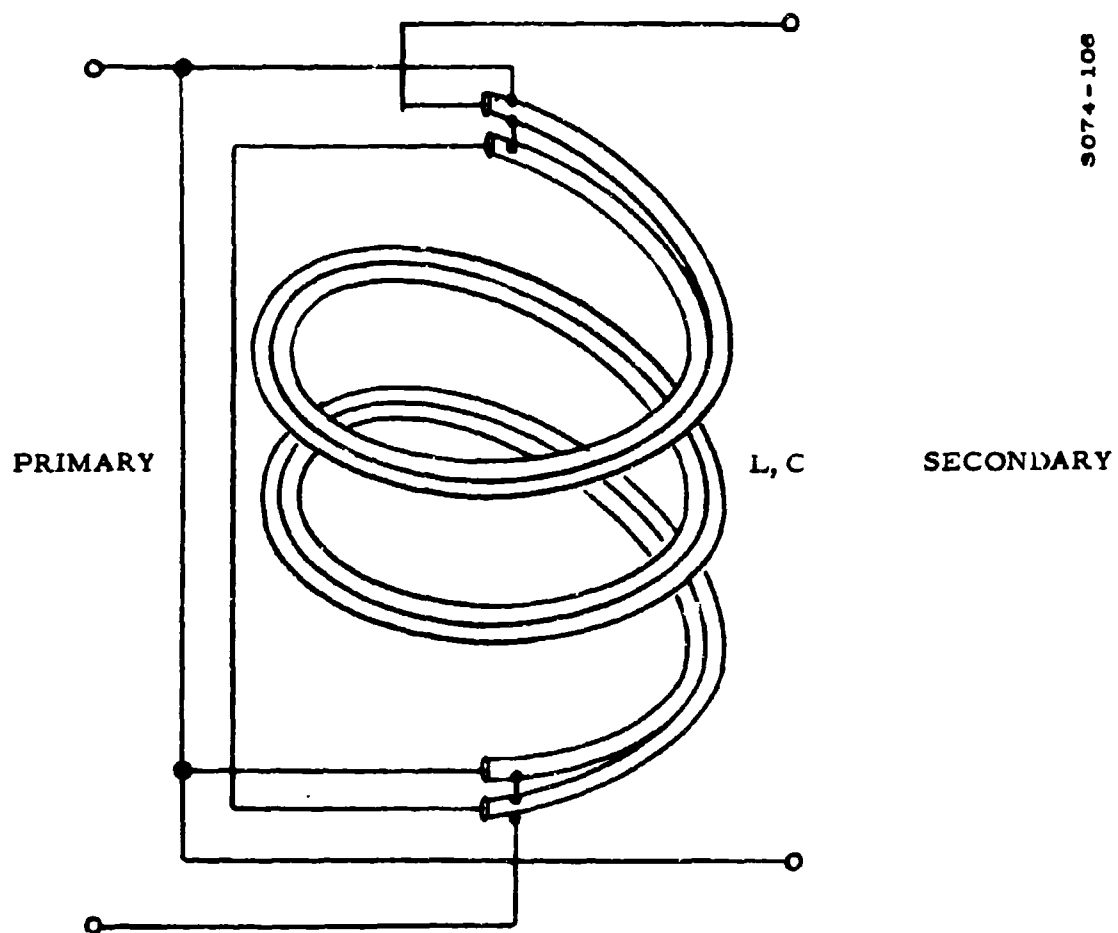
Figure K-3. A 2:1 Transformer of Coaxial Cable
