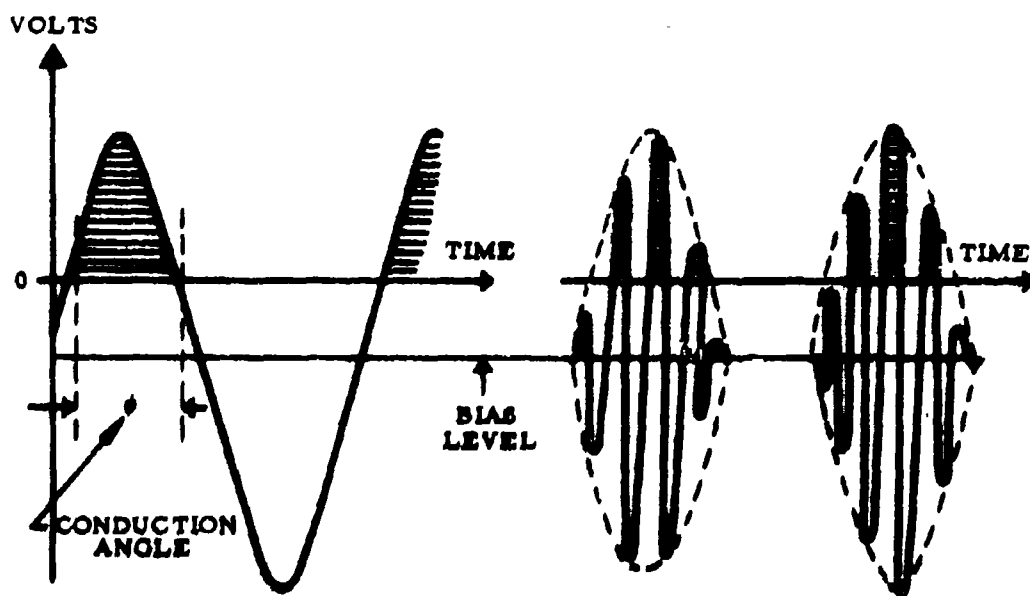
a) STANDARD CLASS C GRID DRIVE b) MODULATED-CARRIER GRID DRIVE
