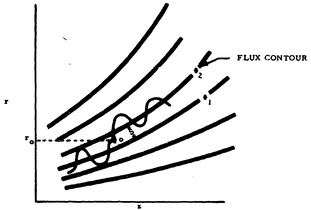
Figure 3-3. Representation of a Scattering Event
