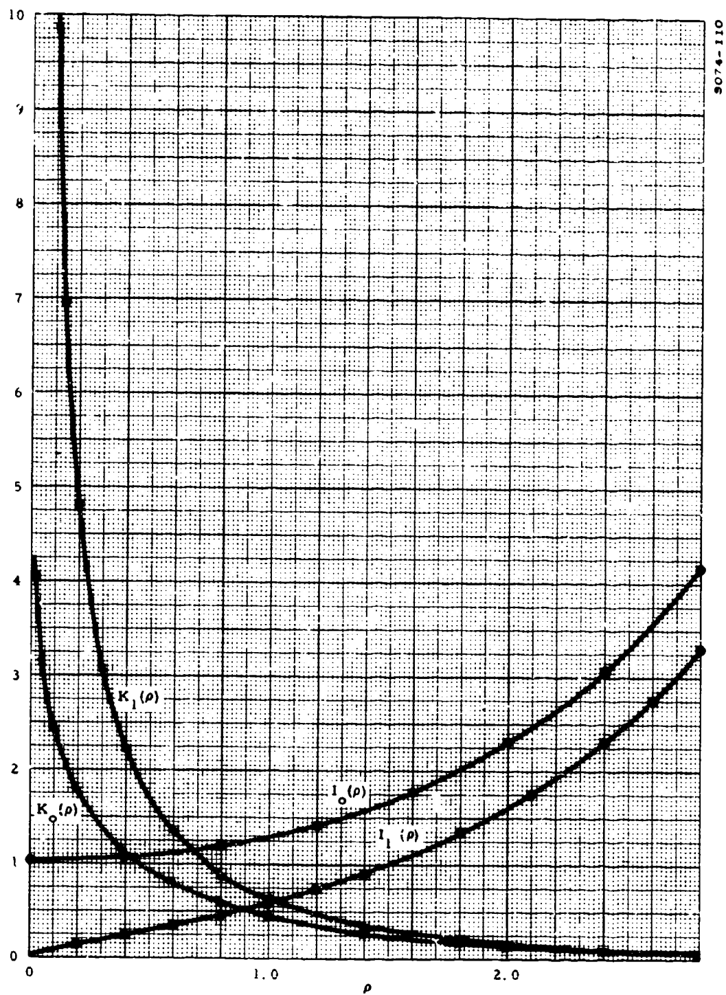
Figure 4-1. Plot of Zeroth- and First- Order Hyperbolic Bessel Functions
