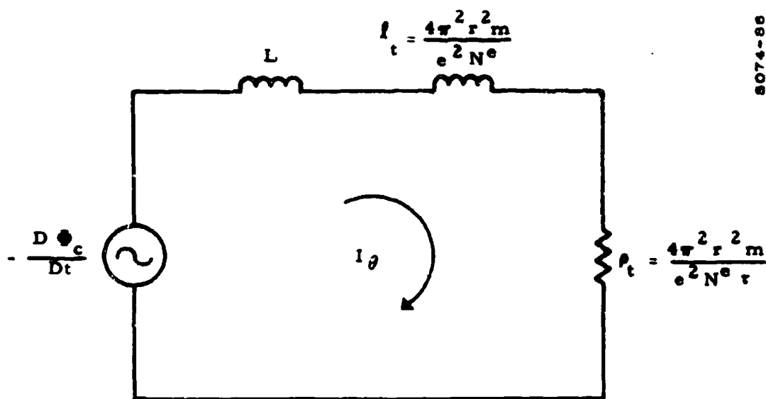
Figure 3-10. Equivalent Electric Circuit for a Torus
