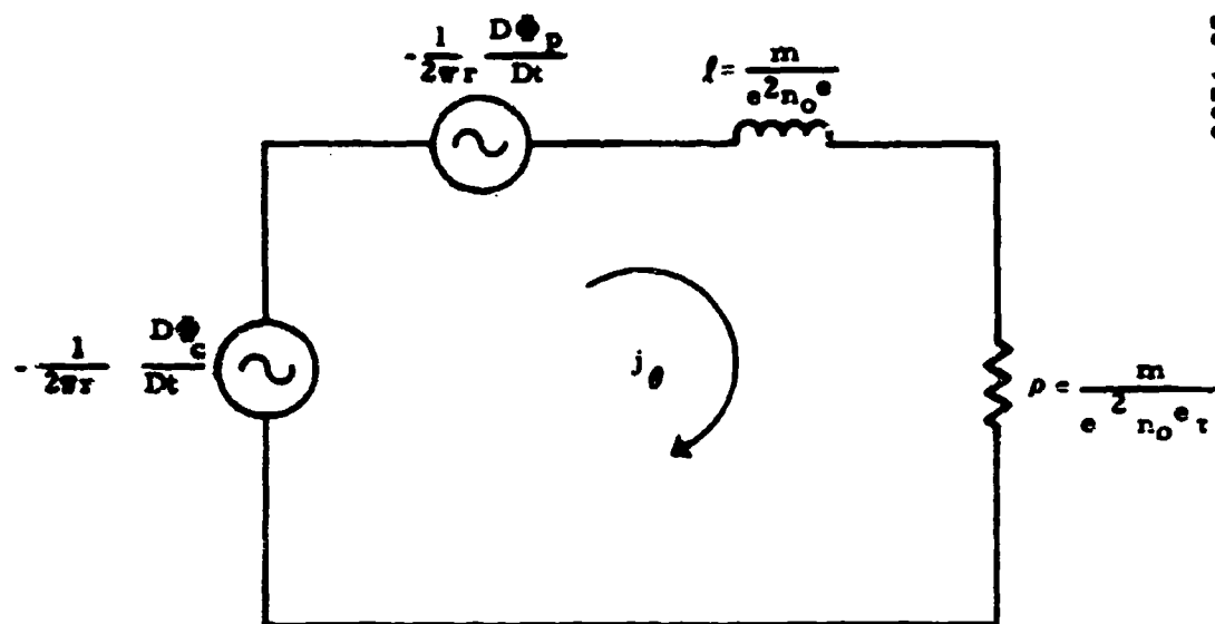
Figure 3-9. Equivalent Electric Circuit for a Plasma
