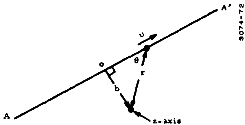
Figure 3-1. Parameters of the Straight-Line Motion of a Particle
