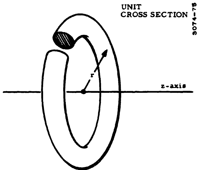
Figure 3-4. Representation of a Torus to Illustrate the Concept of Ring Density
