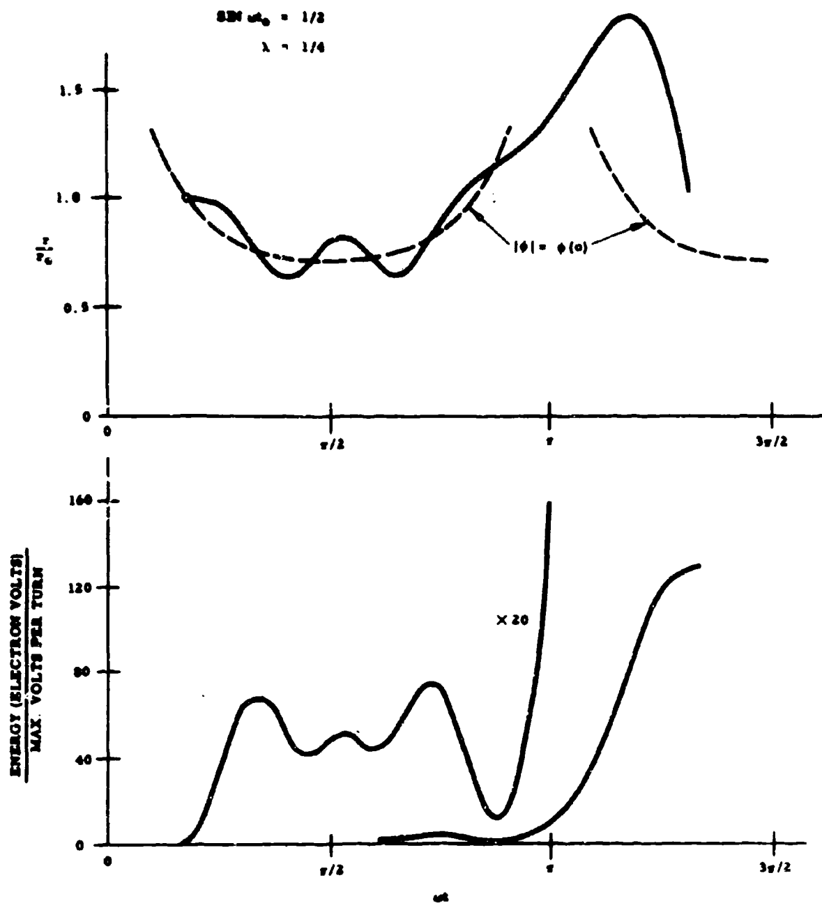
Figure 7. Motion in a Uniform Field, \lambda = 1/4 , \sin \omega t_0 = 1/2
