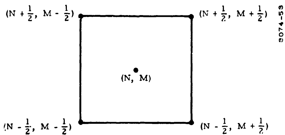
Figure G-1. Rectangle of Integration
