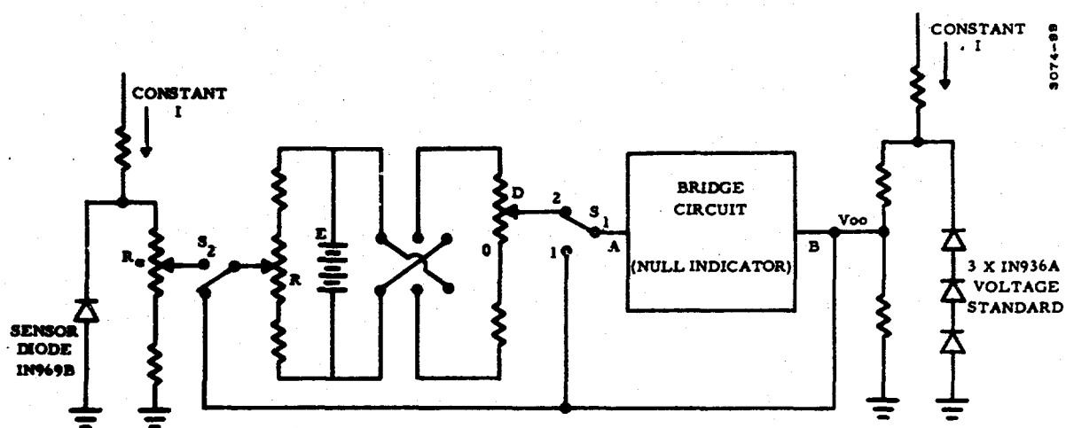
Figure M-1. Basic Arrangement of Sensing Circuit
