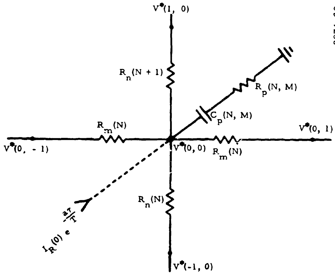
Figure G-8. Plasma Analog
