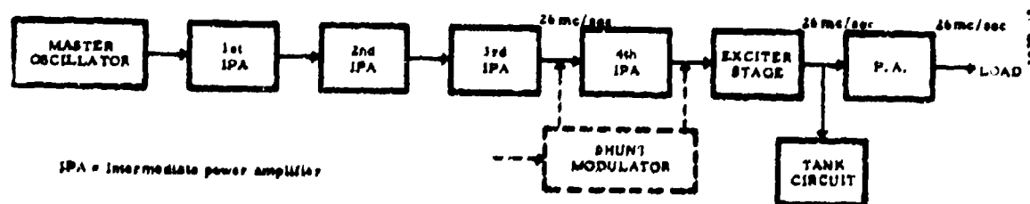
Figure I-5. Block Diagram of Unmodified TBC-3 Transmitter (Modification Shown Dotted)
