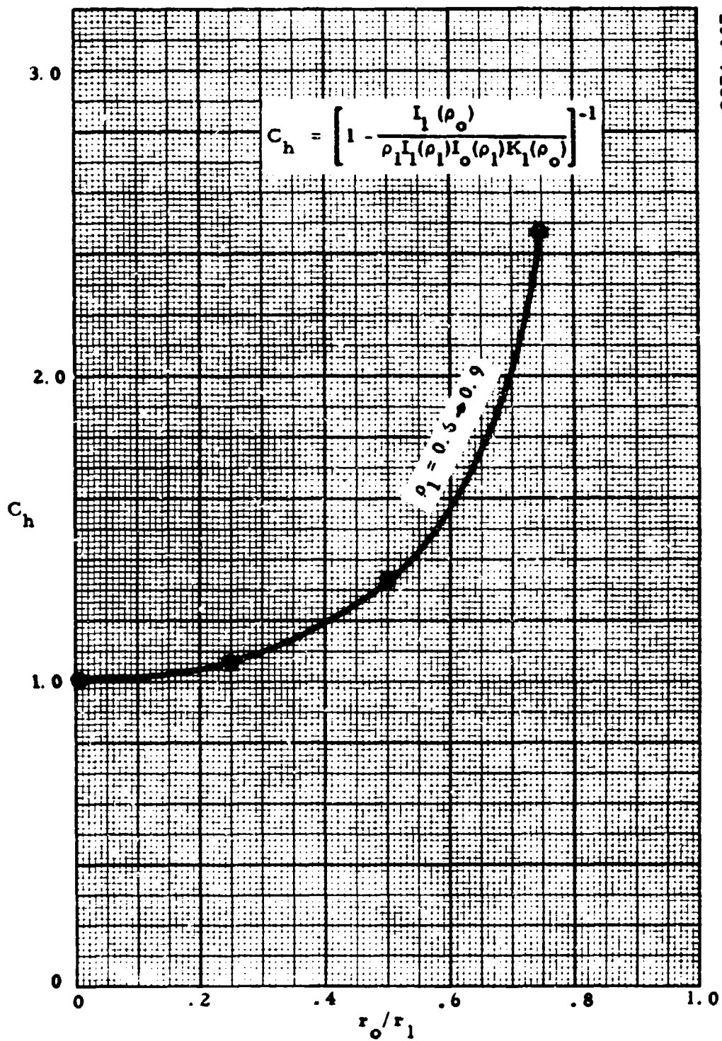
Figure 4-9. Plot of C_h vs r_o/r_1
