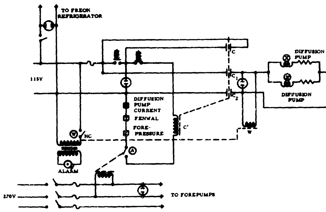
Figure H-11. Schematic of Vacuum System Circuitry
