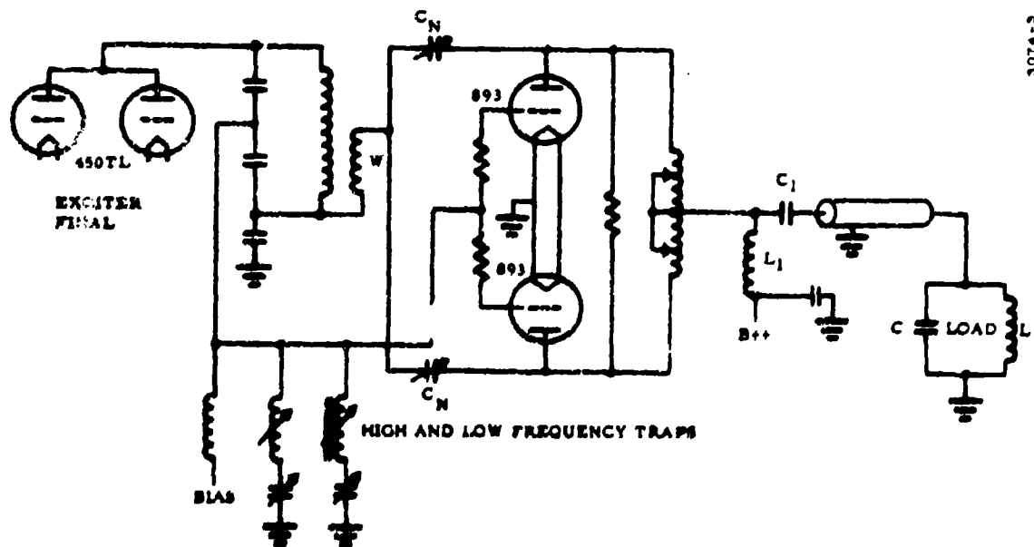
Figure I-3. Neutralization and Grid Traps
