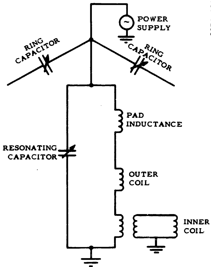
Figure 4-15. Schematic of One Node of Coupling Circuit
