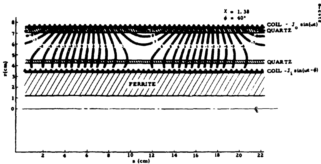
Figure 4-4. Calculated Magnetic Field Pattern of Accelerator
