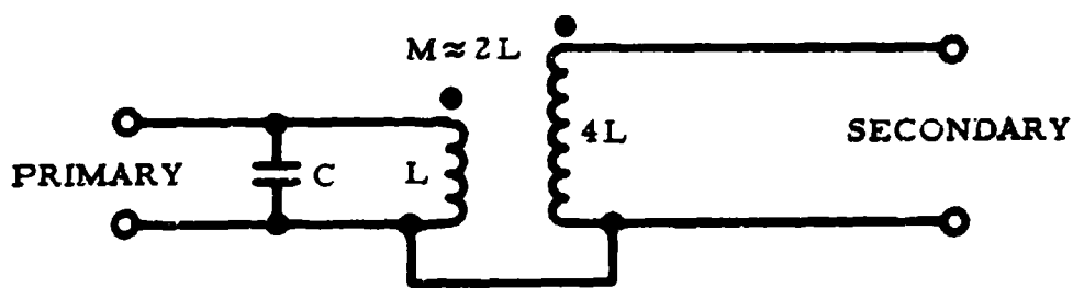
Figure K-5. Equivalent Circuit
