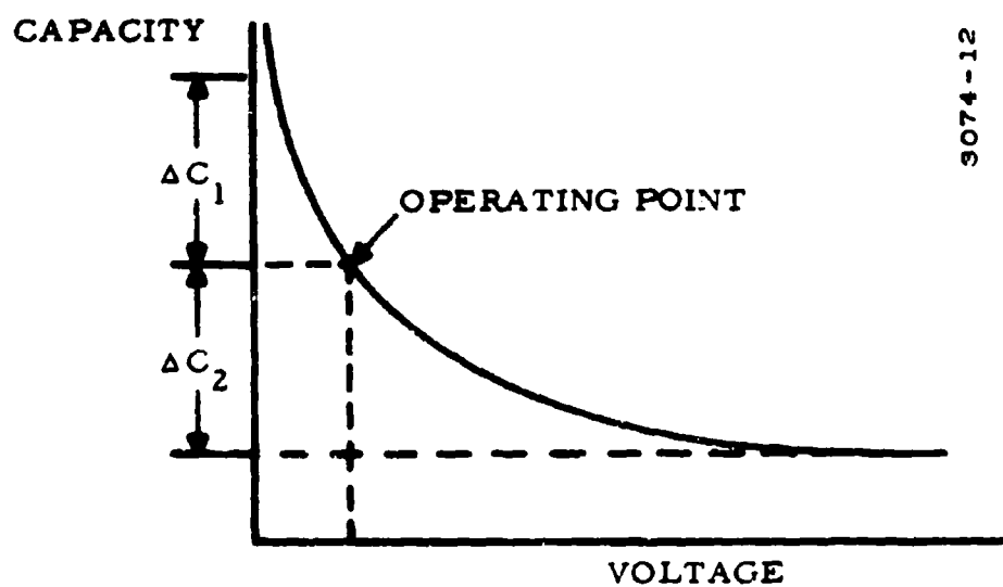
Figure J-6. Typical Operating Characteristics of a Voltage-Variable Capacitor
