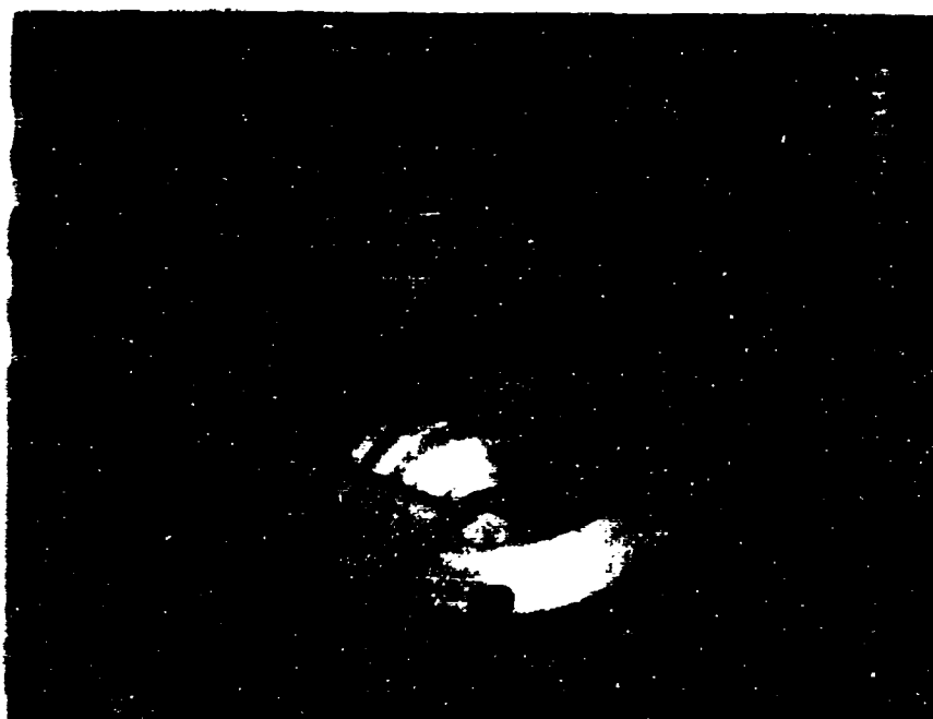
Figure A-3. Interior of a Spark Gap Chamber Showing Arc Pits on the Wall
