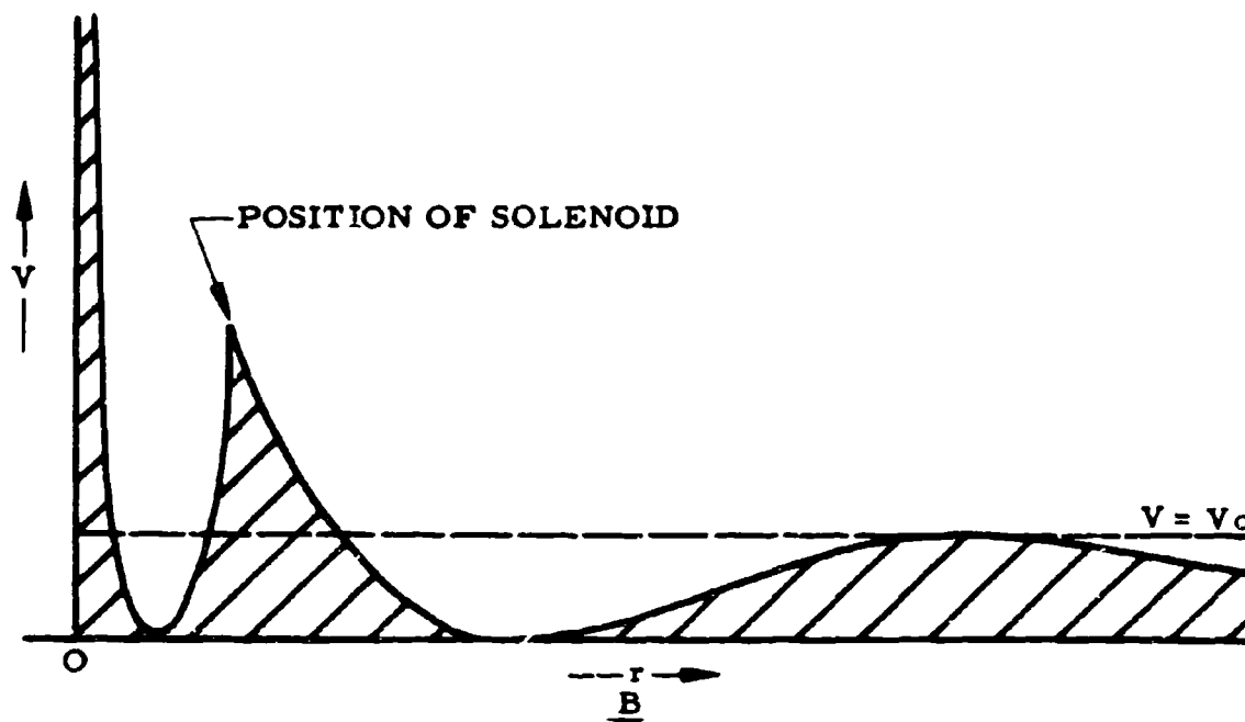
Figure 3. Cross Sections of an Inductive Potential Pattern for a Solenoid
