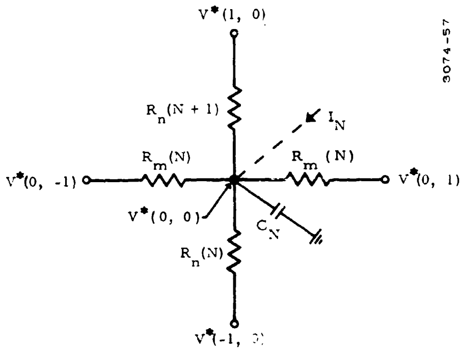
Figure G-5. Analog for Metal Objects
