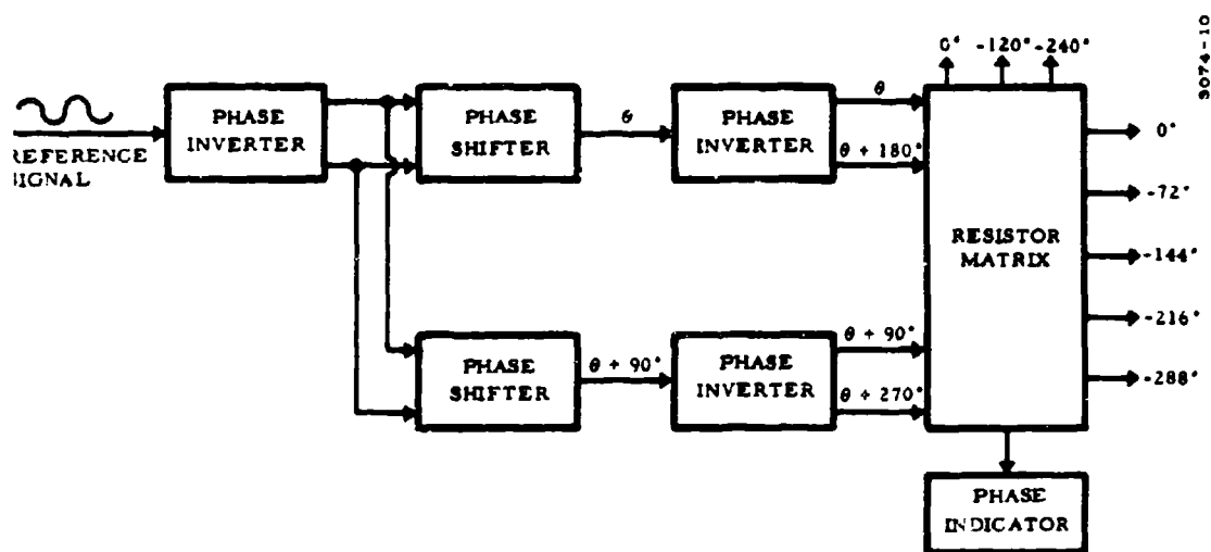
Figure J-8. Polyphase Generator
