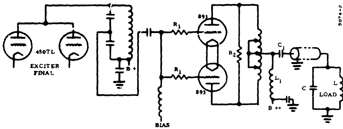
Figure I-2. Modified Output Circuit with Parasitic Resistors
