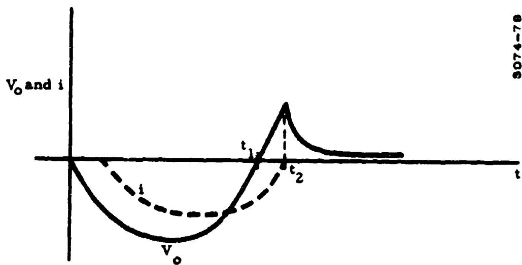
Figure J-14. Voltage and Current in Display Circuit
