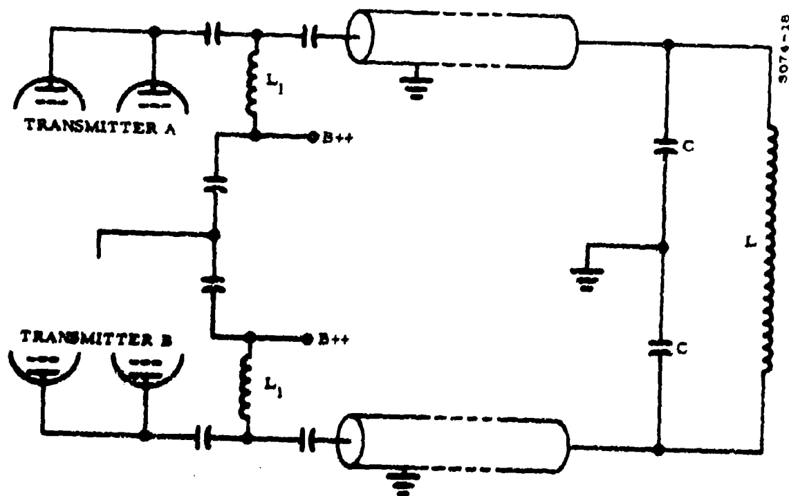
Figure 1-4. Push-Pull Load Using Two Transmitters
