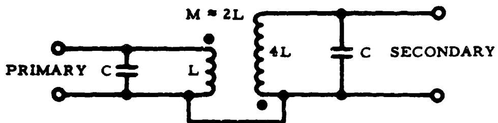
Figure K-4. Equivalent Circuit of the Transformer in Figure K-3
