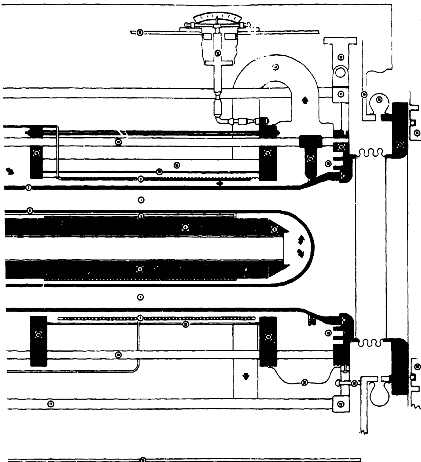
Figure H-2. Accelerator Cross Section
