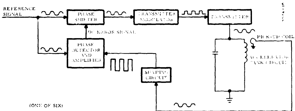
Figure J-2. Phase Control System
