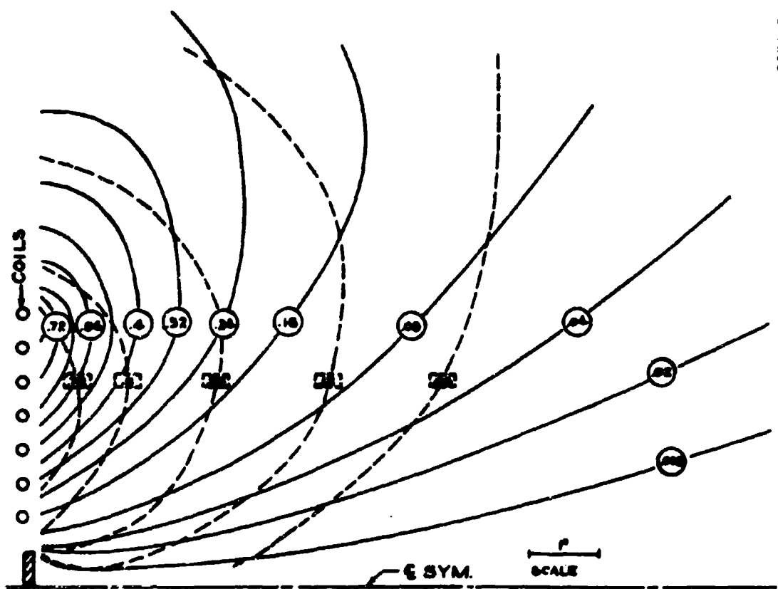
Figure F-1. Field Patterns from an Array of Coils Excited at 1 Mc
