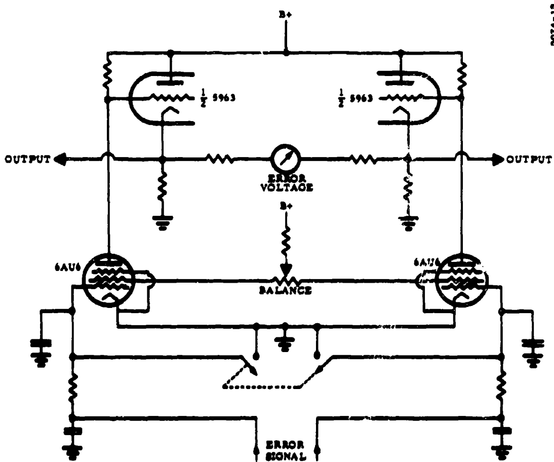
Figure J-5. Differential Amplifier
