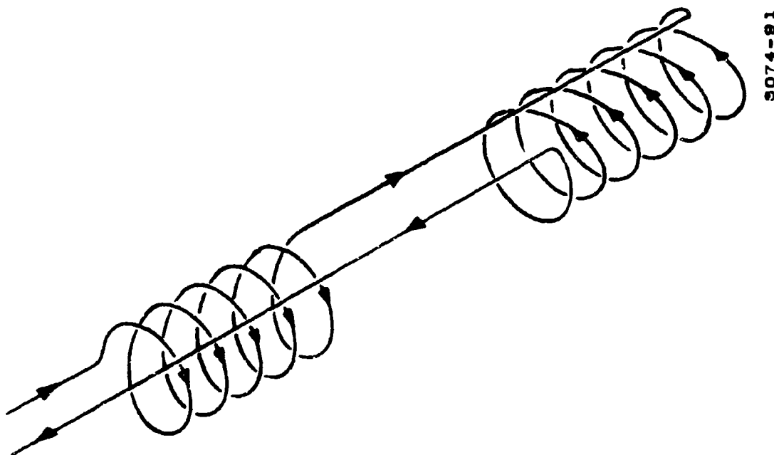
Figure H-6. Field Coil Winding
