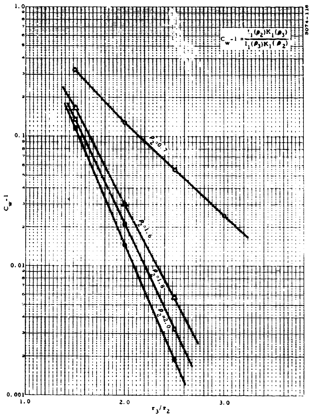
Figure 4-8. Plot of C_w - 1 vs r_3/r_2
