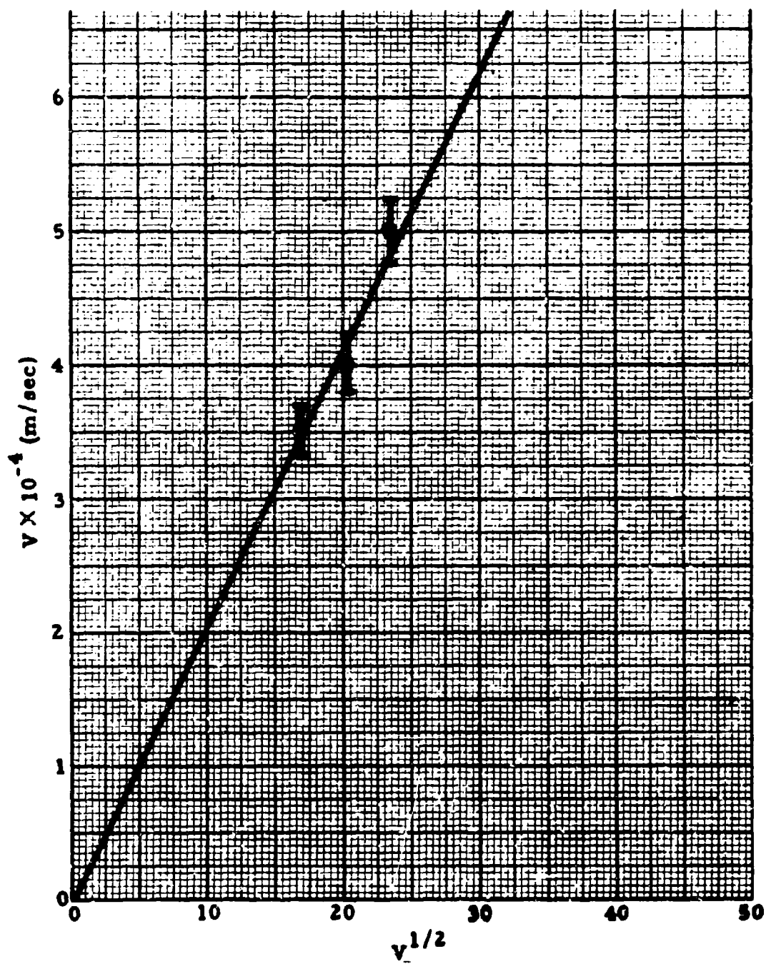
Figure 2-3. Plot of Measured Speeds vs Square Root of Voltage
