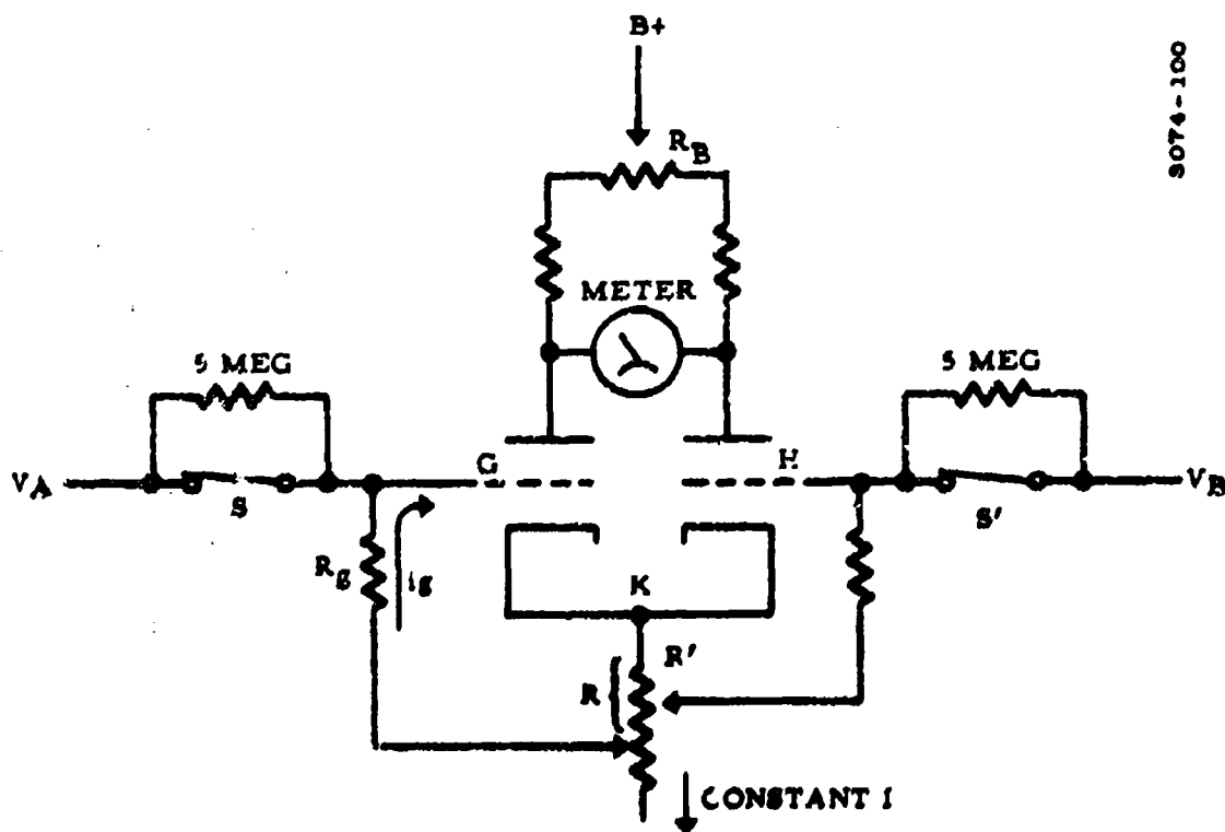
Figure M-2. Basic Circuit of Null-Indicating Bridge
