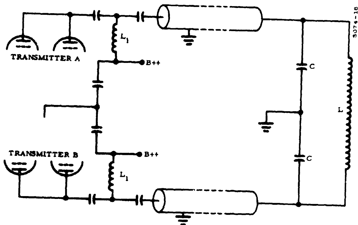
Figure I-4. Push-Pull Load Using Two Transmitters
