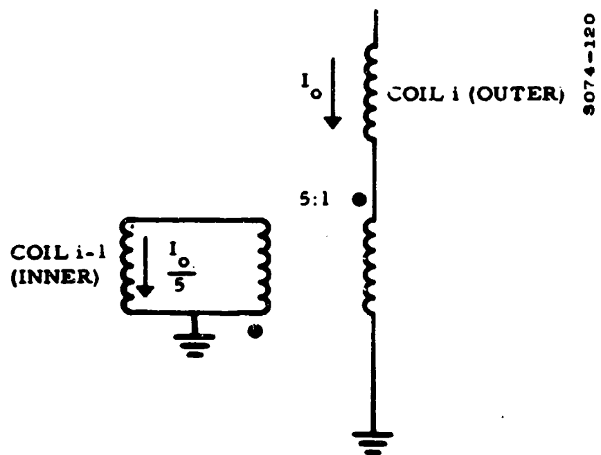
Figure 4-14. Coupling System for Inner Coils
