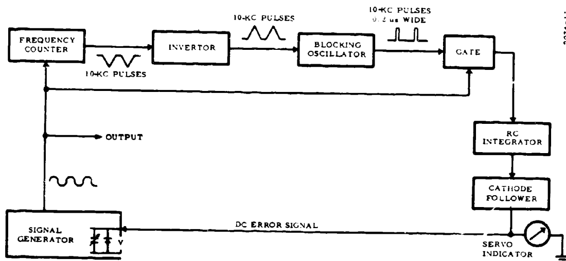
Figure J-1. Block Diagram of the Stable Frequency Source
