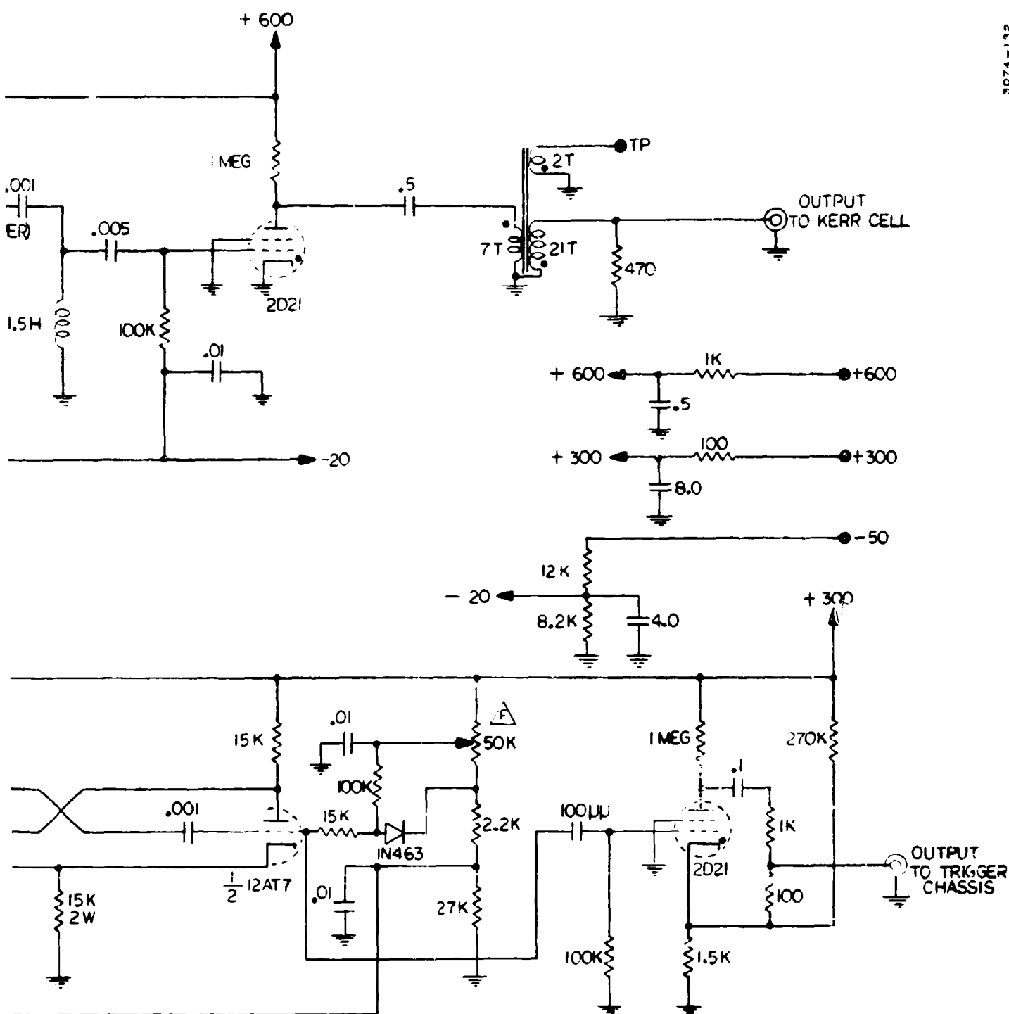
Figure A-8. Kerr Cell Timing Chassis Schematic
