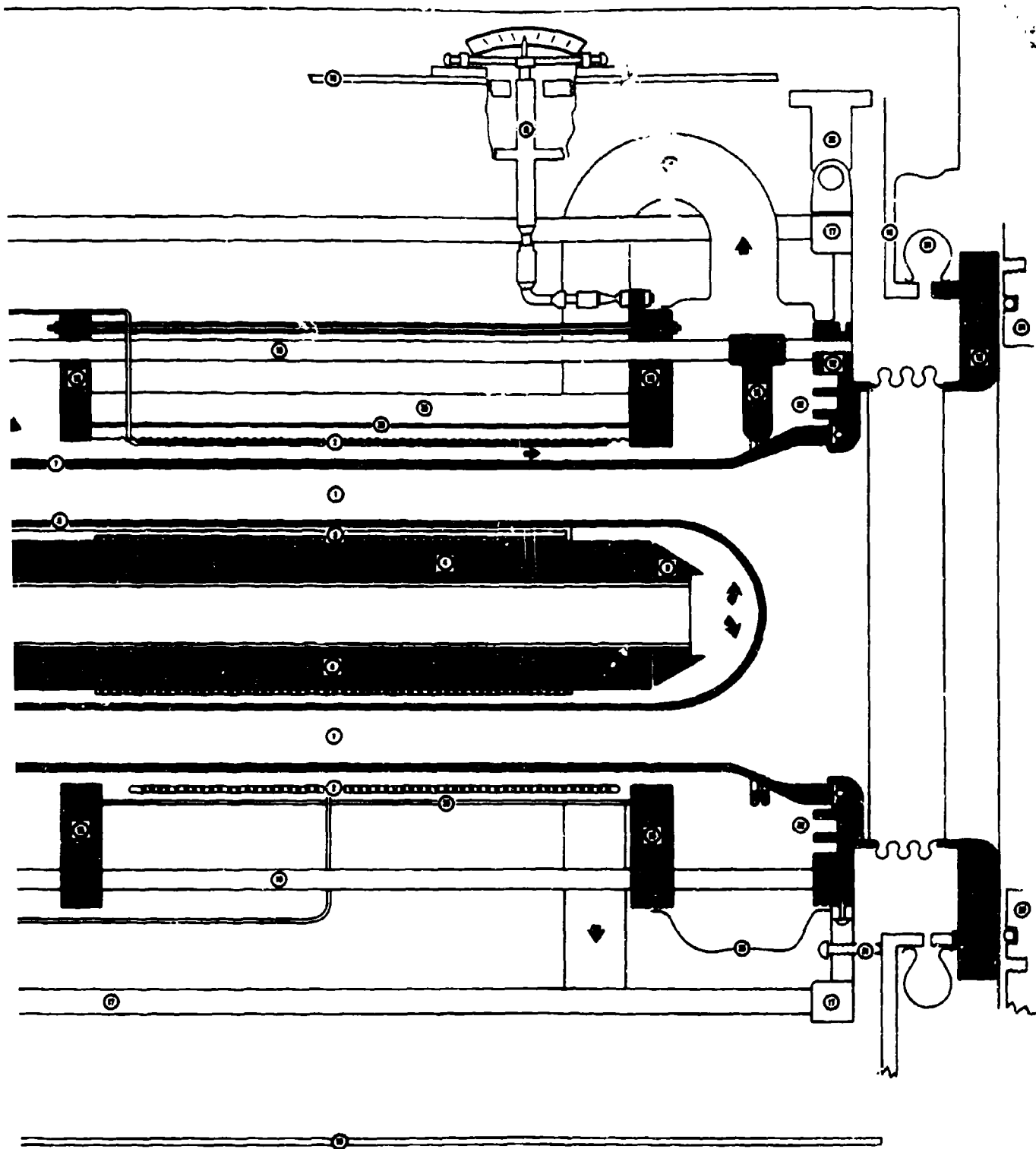
Figure H-2. Accelerator Cross Section
