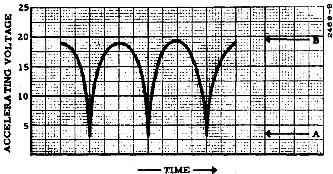
Figure 3-3. Plot of Accelerating Voltage vs Time
