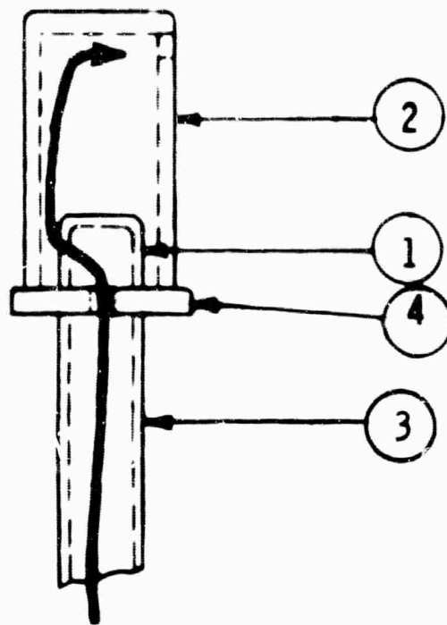
Fig. 2—Chamber for heating ThO 2 specimens in pure oxygen
