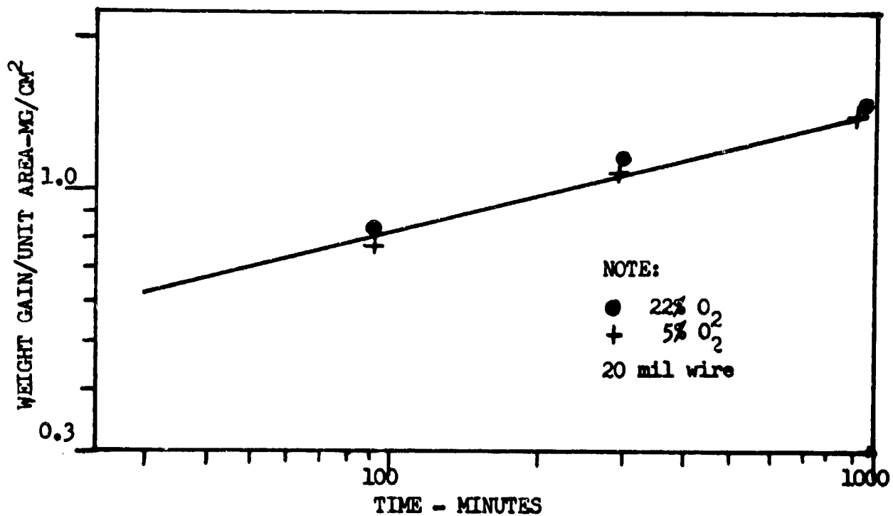
FIG.28 EFFECT OF O 2 PARTIAL PRESSURE ON OXIDATION OF T D NICKEL AT 1600 F
