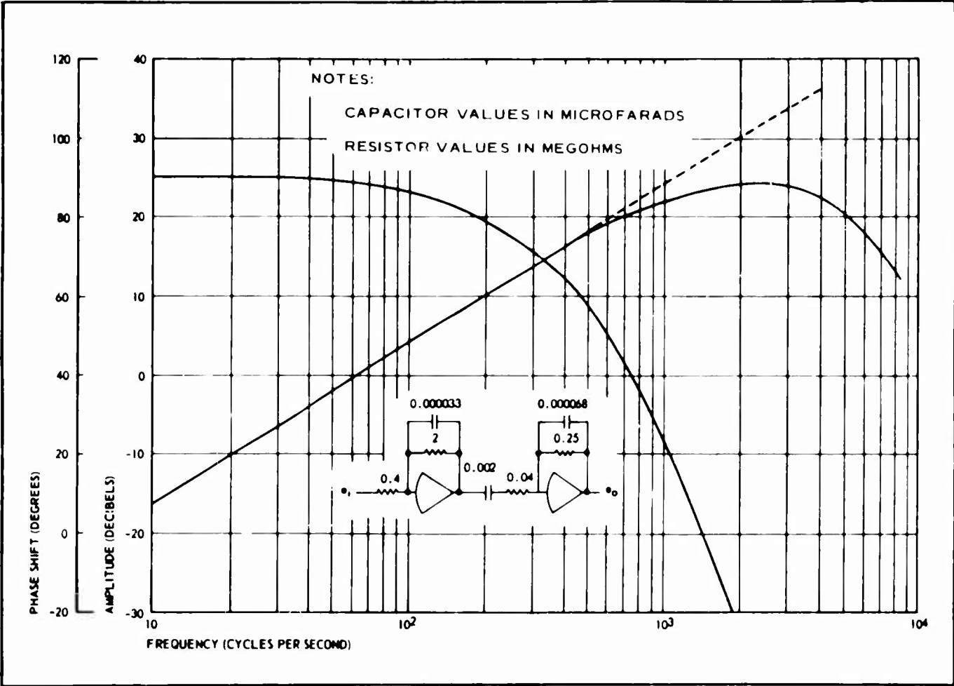
Figure 28 - Differentiator Characteristics
