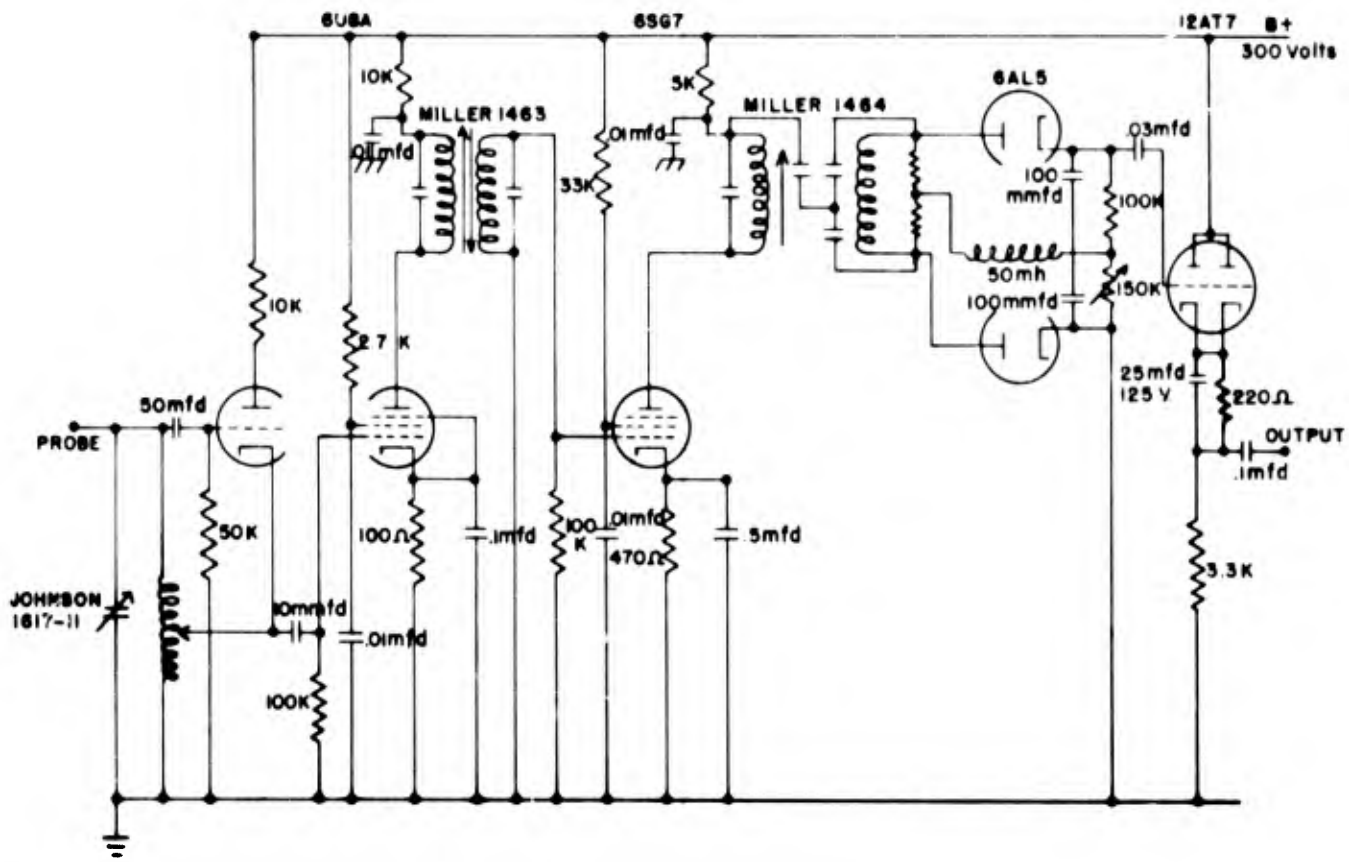
Figure 3: Circuit Diagram of the Displacement Detector
