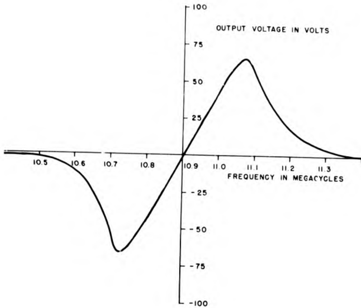
Figure 2: Output Voltage - Frequency Relationship for FM Discriminator
