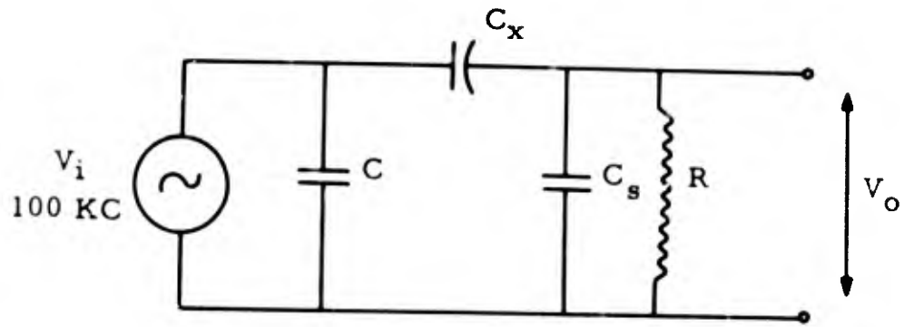
Figure 1: Diagrammatic Representation of Békésy's Displacement Measuring System.
