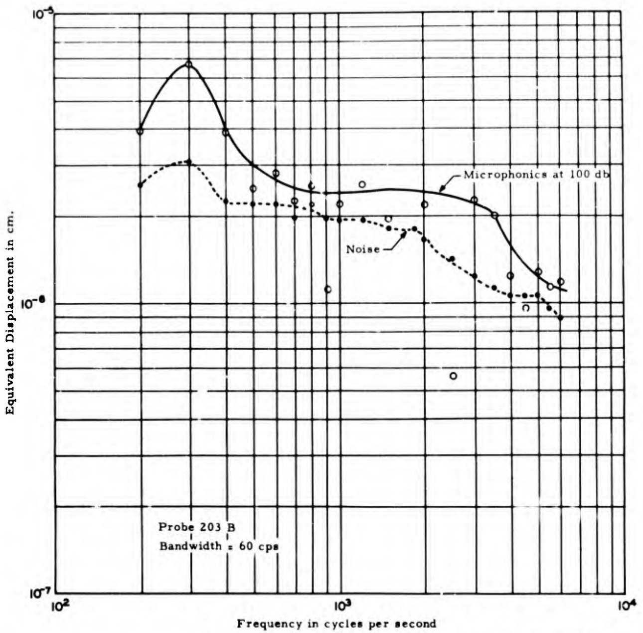
Figure 5: Noise Equivalent Displacement and Microphonic Equivalent Displacement for Probe #203B.
