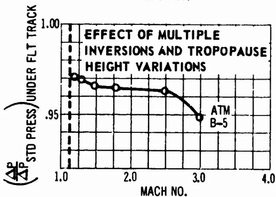
Fig. 10 Effect of Pressure Variations on Sonic Boom Produced Under the Flight Track.
