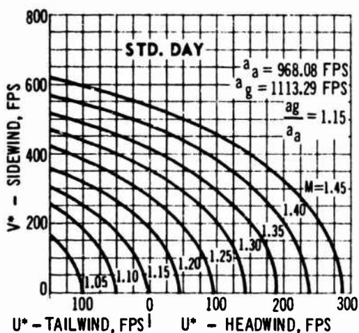
Fig. 25 Wind speeds Required to Produce Focusing Off the Flight Track.
