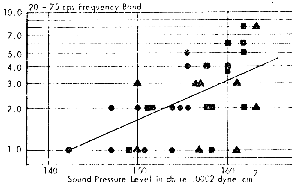
Figure 12- Comparison of Internal Vibration of Structure and Adjacent External Sound Pressure Level for Two Frequency Ranges.
