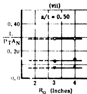
FIGURE 27a. EFFECT OF DEFLECTION SURFACE RADII ON THE NON-DIMENSIONAL LIFT FORCE FOR VARIOUS HORIZONTAL AND VERTICAL GAP SIZES AND NOZZLE PRESSURE RATIOS.
