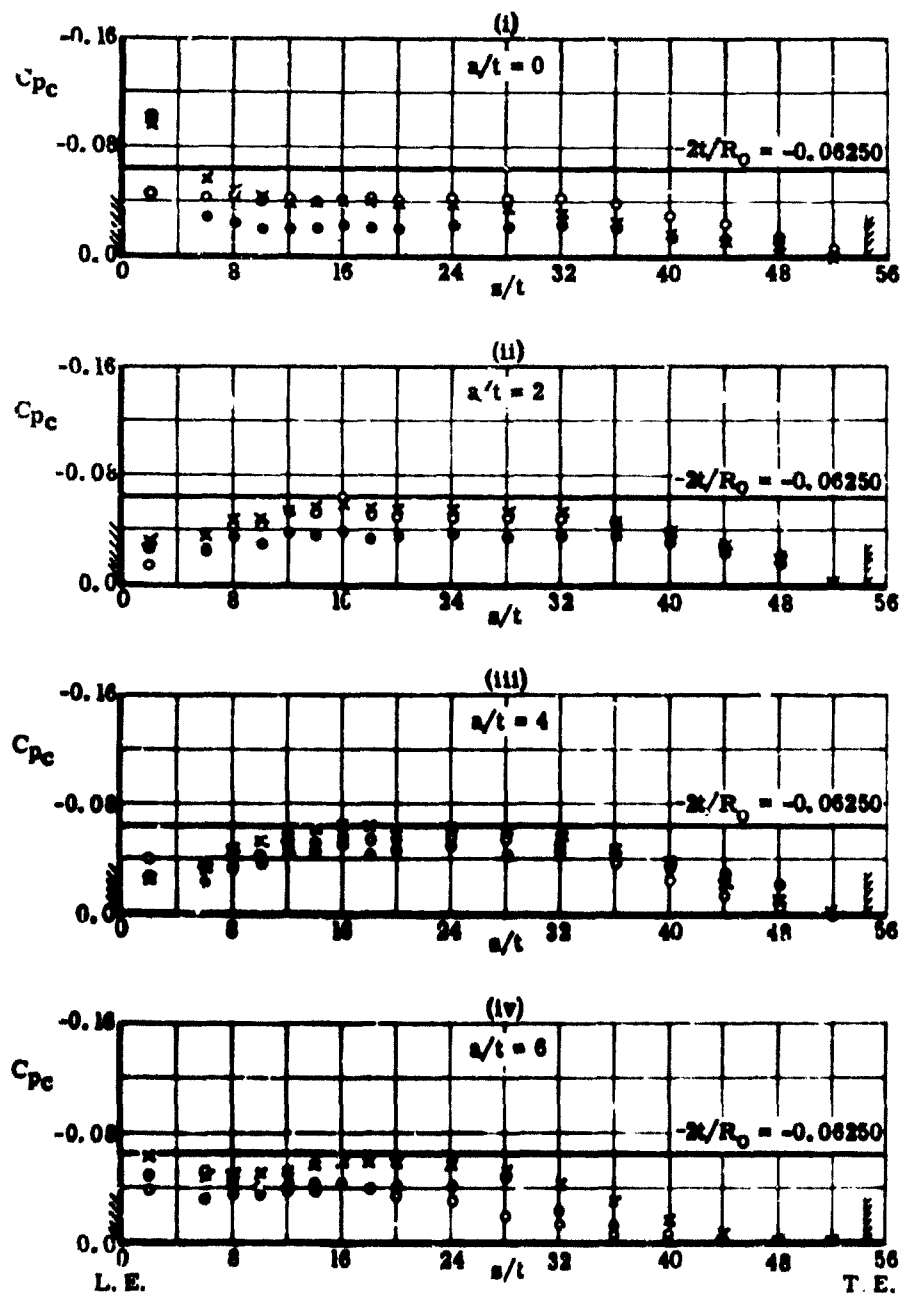
FIGURE 14d. EFFECT OF THE VERTICAL GAP SIZE ON THE PRESSURE COEFFICIENTS CORRECTED FOR FLOW COMPRESSIBILITY AT VARIOUS NOZZLE PRESSURE RATIOS.
