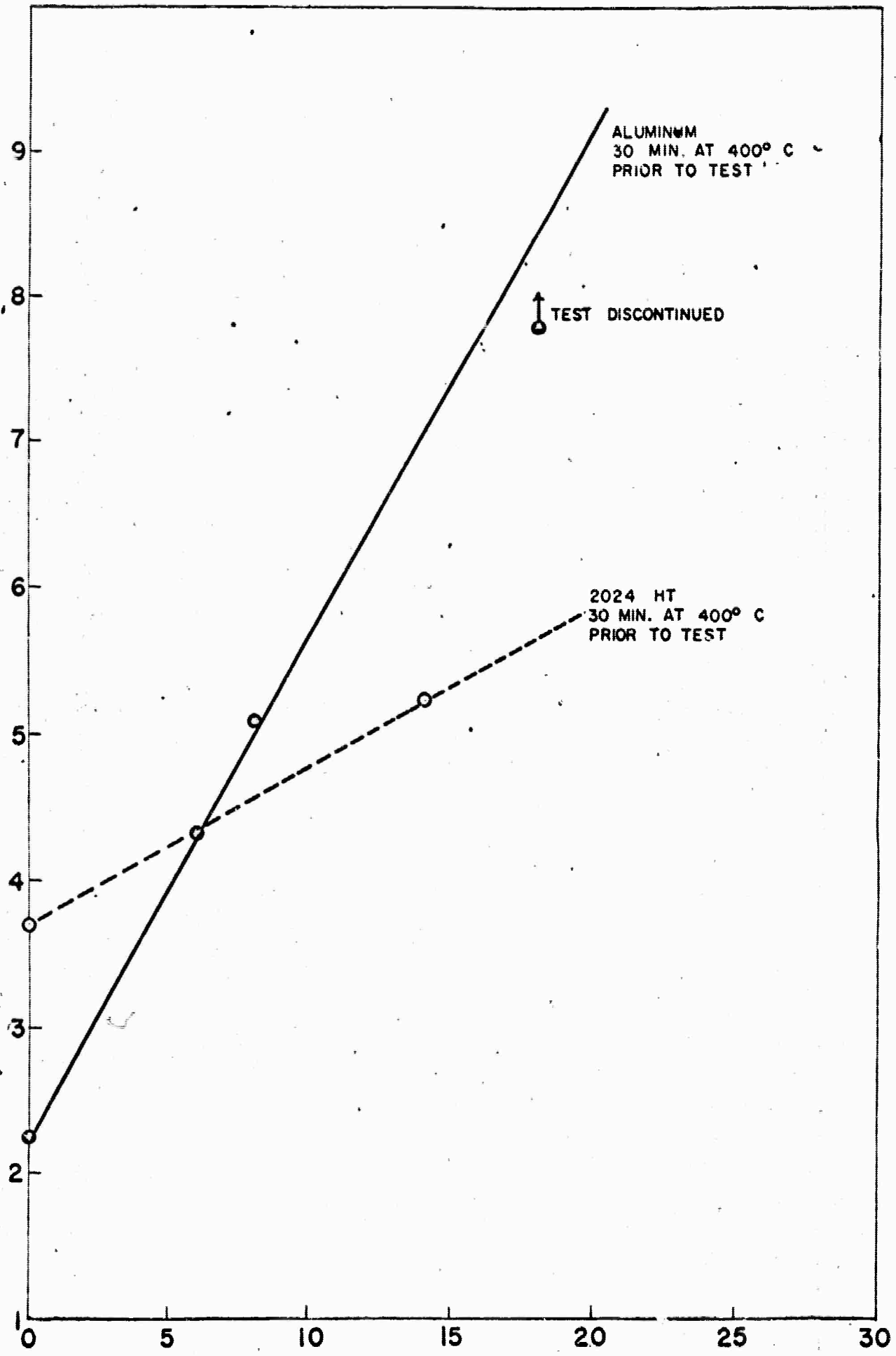
EFFECT OF FIBER ON HIGH TEMPERATURE (400° C) STRENGTH
