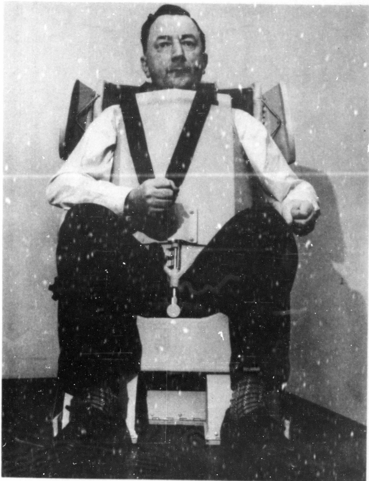
FIGURE 6a. SEAT MOCK-UP - FRONT VIEW
