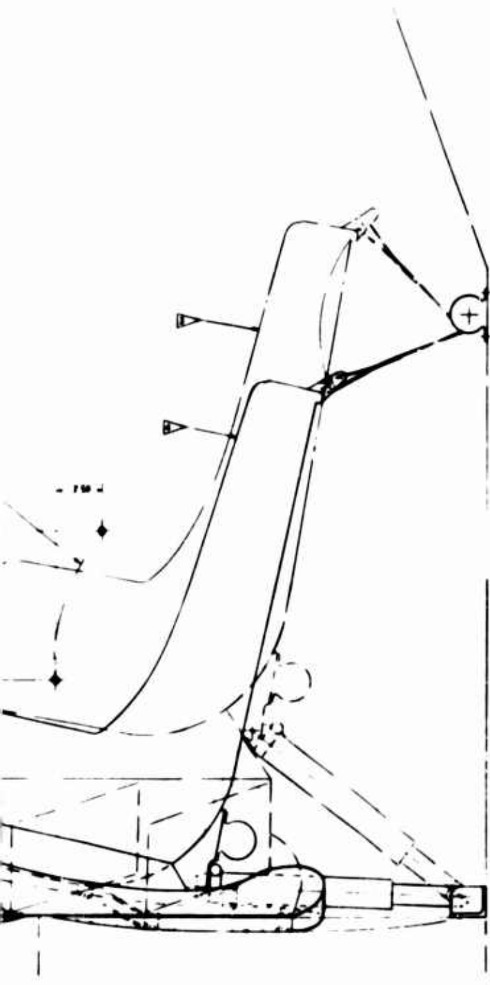
SEAT POSITION PRIOR TO VERTICAL CRASH LOAD
