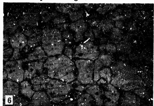
G-251-15R Avg. Particle Size 19 Microns Density = 5.26 gm/cm 3
