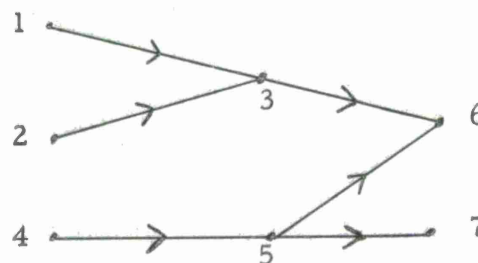
Precedence Graph
