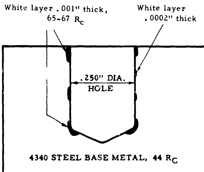
FIGURE 3. WHITE UNTEMPERED MARTENSITIC LAYER ON SURFACE OF DRILLED HOLE; 4340 STEEL, Q&T TO 44 R_C
