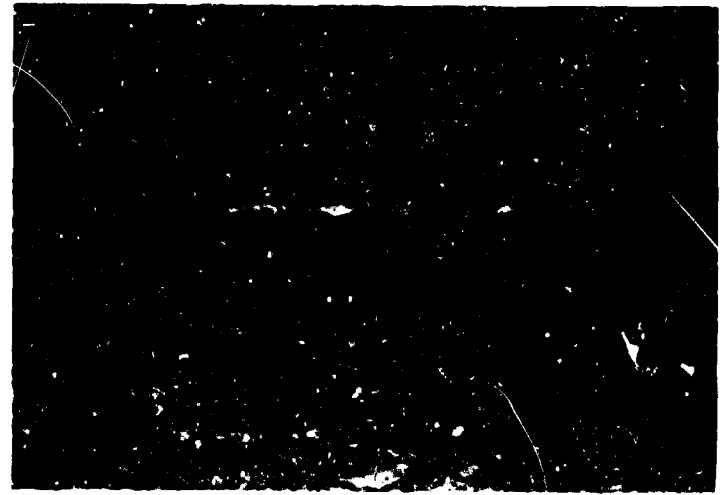
FIGURE 19. FRACTURE PATH THROUGH AUSTENITE BANDS IN SMOOTH TENSION-TEST FRACTURE SHOWN IN FIGURE 18. LIGHT MICROGRAPH OF POLISHED AND ETCHED LONGITUDINAL SECTION.
