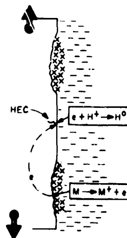
FIGURE 5. HYDROGEN-EMBRITTLEMENT CRACKING (HEC) FROM AQUEOUS CORROSION (SCHEMATIC, CONJECTURAL)
