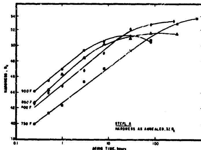
FIGURE 7. AGING RESPONSE OF MARAGING (250) STEEL A
