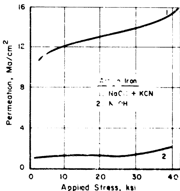
FIGURE 13. DEPENDENCE OF PERMEATION ON APPLIED STRESS
