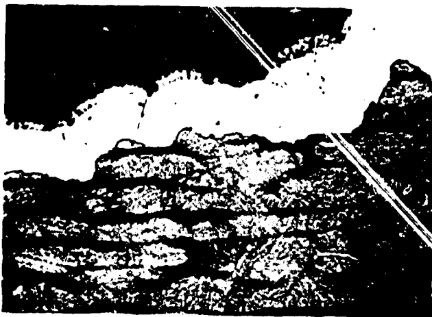
FIGURE 23. FRACTURE PROFILE OF "POP-IN" REGION OF SPECIMEN "D". LIGHT MICROGRAPH OF POLISHED AND ETCHED SECTION
