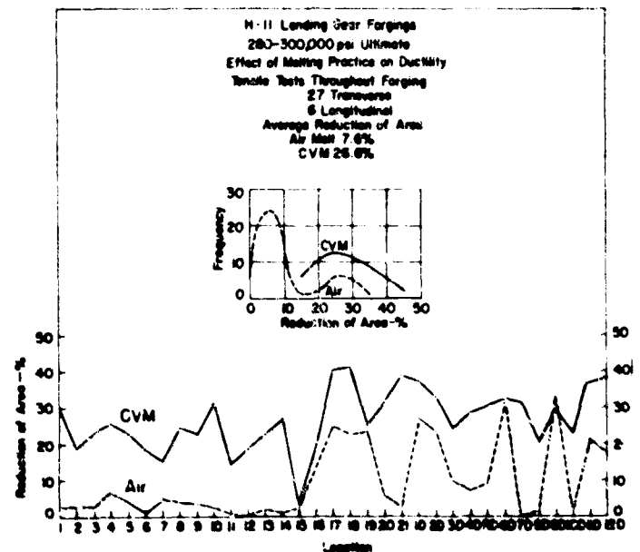
FIGURE 4. COMPARATIVE DUCTILITY OF AIR-MELT AND CONSUMABLE-VACUUM-MELT SPECIMENS FROM LOCATIONS SHOWN IN FIGURE 3. FREQUENCY DISTRIBUTION OF ALL TESTS SHOWN IN INSERT (Ladish, Cleveland Pneumatic)
