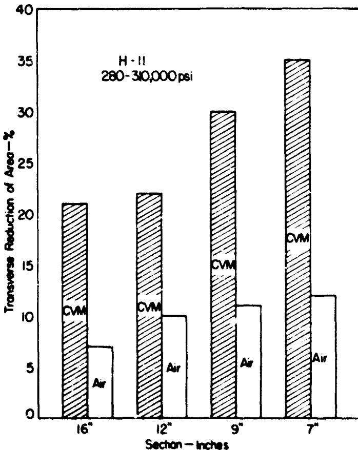
FIGURE 2. EFFECT OF CONSUMABLE-VACUUM MELTING ON TRANSVERSE DUCTILITY AT 280-310-KSI ULTIMATE TENSILE STRENGTH IN LARGE BILLETS OF H-11 FOR AEROSPACE COMPONENTS
