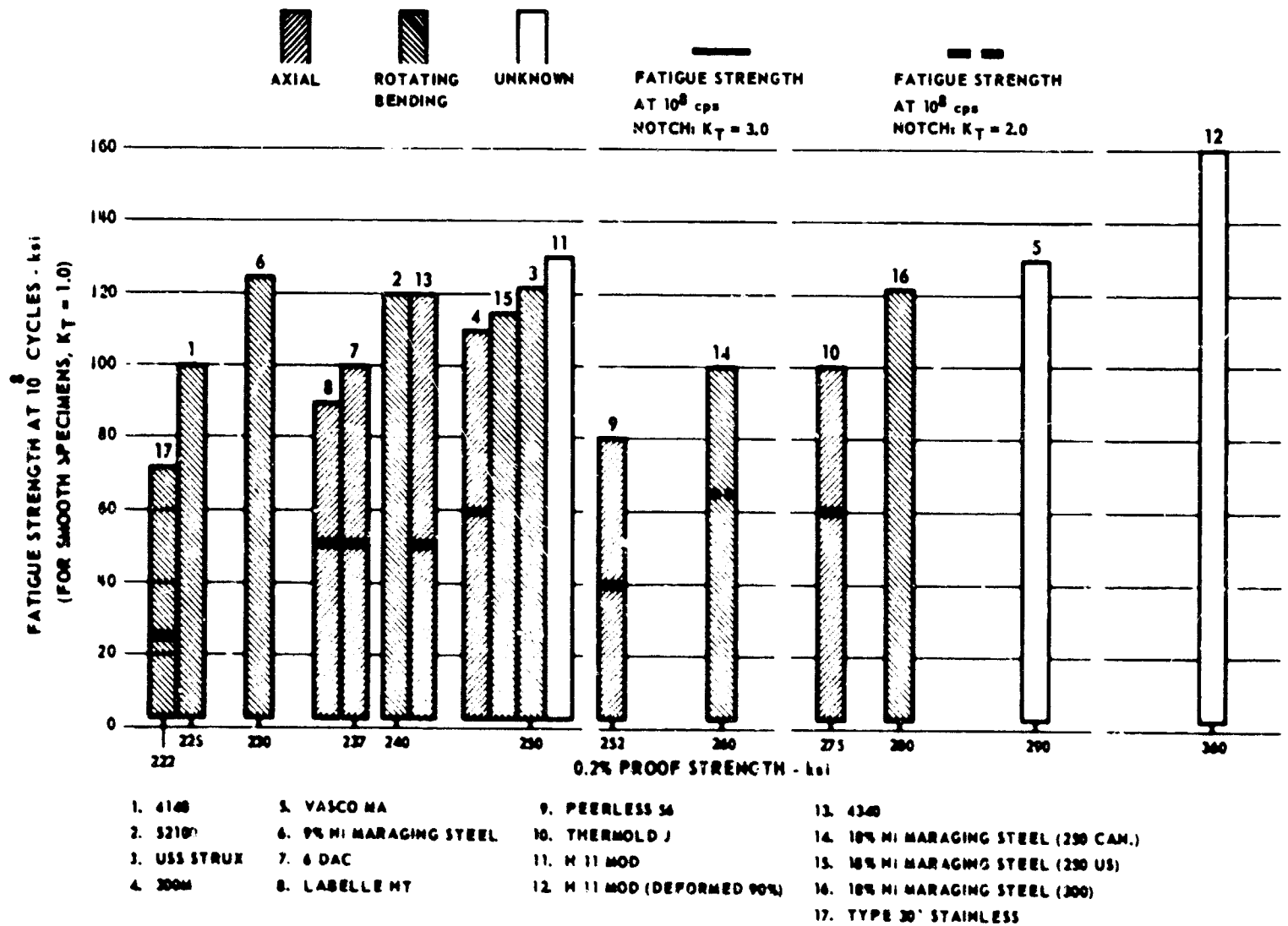
FIGURE 1b. FATIGUE STRENGTHS OF ULTRAHIGH-STRENGTH STEELS
