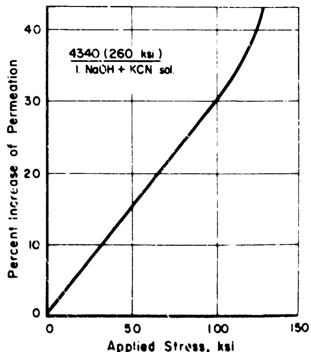
FIGURE 14. PERCENTAGE INCREASE IN PERMEATION WITH INCREASED APPLIED STRESS
