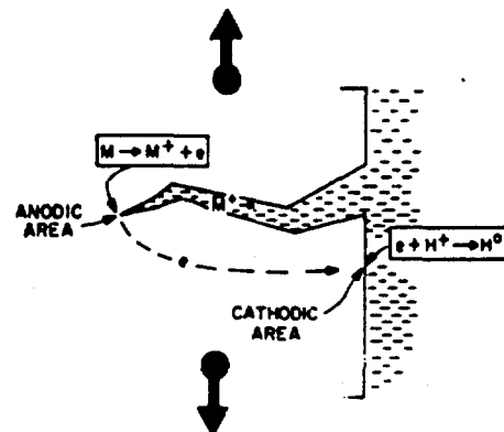
FIGURE 3. STRESS-CORROSION CRACKING (SCHEMATIC)
