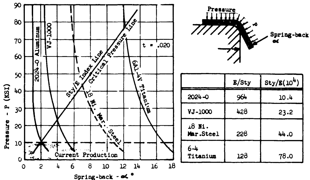
FIGURE 5. RUBBER FORMING STRAIGHT FLANGES
