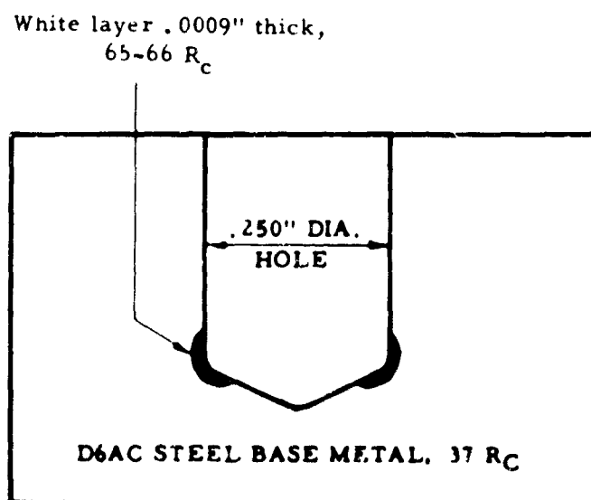
FIGURE 4. WHITE UNTEMPERED MARTENSITIC LAYER ON SURFACE OF DRILLED HOLE; D6AC STEEL, ANNEALED TO 37 R_C
