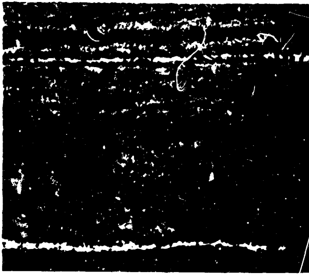
FIGURE 17. AUSTENITE AND SEGREGATION BANDS IN ROLLED PLATE OF MARAGING (250) STEEL. LIGHT MICROGRAPH OF POLISHED AND ETCHED LONGITUDINAL SECTION.
