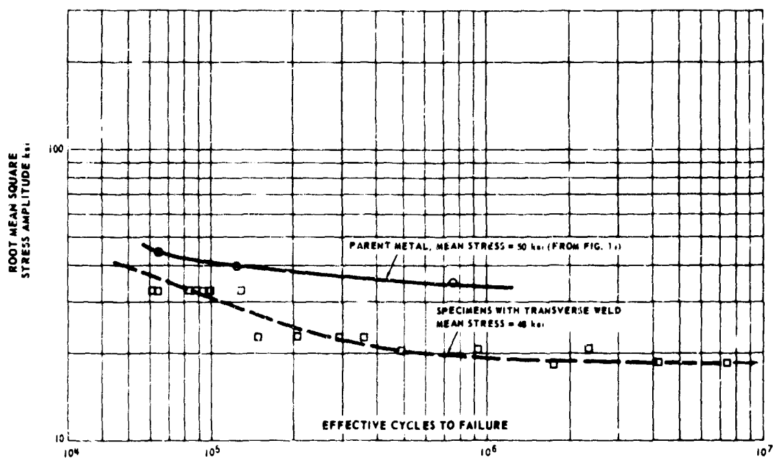
FIGURE 16. RANDOM LOAD FATIGUE \sigma -N CURVES FOR AIR TESTS USING CONSUMABLE ELECTRODE VACUUM-MELT AND VACUUM-CAST MARAGING STEEL
