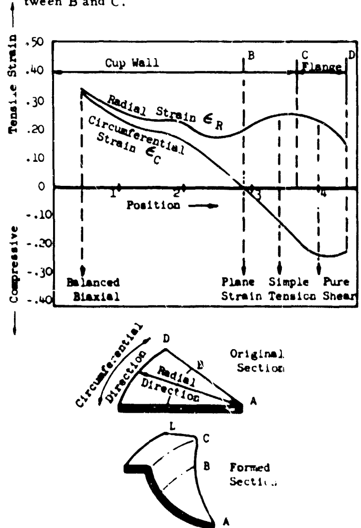
FIGURE 11. BIAxIAL STRAINS IN EXPLOSIVE FORMING OF DOME
