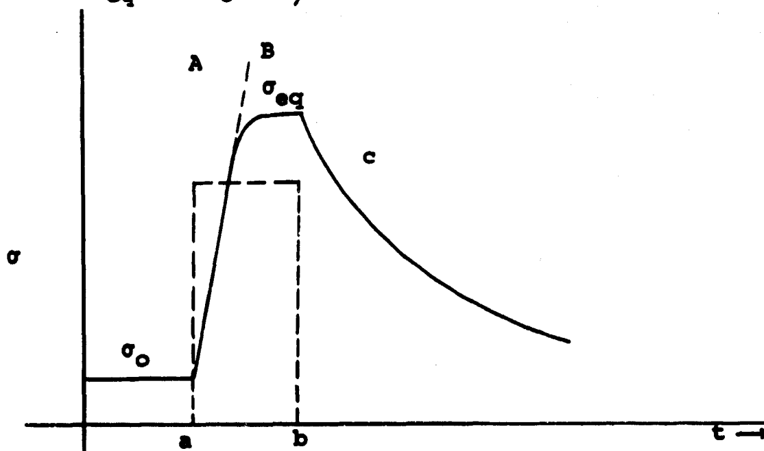
Figure 5. The Conductivity-Time Behavior for the Gamma Pulse Shown.
