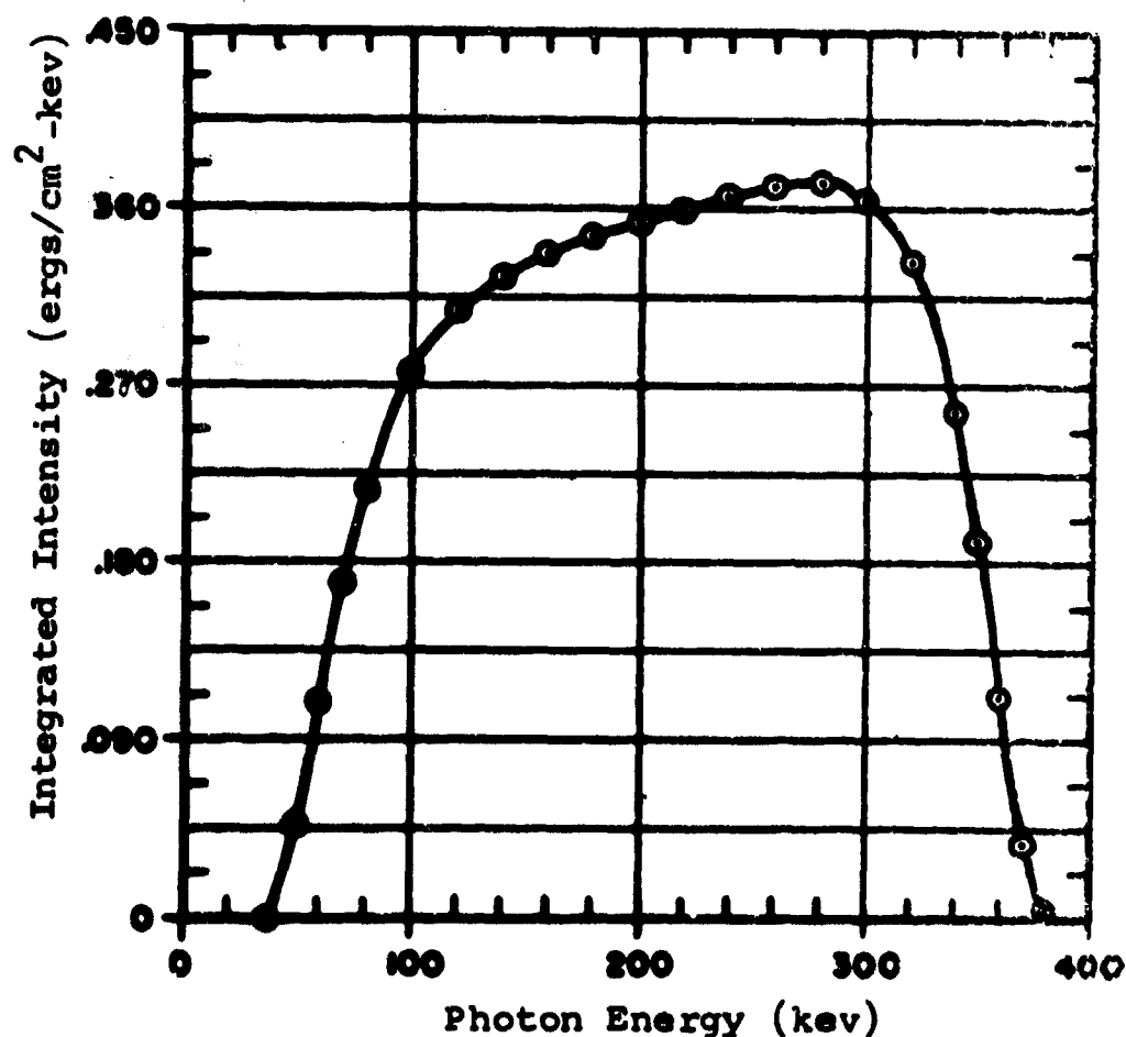
Figure 33. Time-Integrated Intensity Spectrum of 400-kev X-Ray Machine at 20 in. From the Target. The Total Energy was 90 ergs/cm² with the Geometry Shown in Figure 24. The X-Ray Beam was Filtered with .050 in. of Copper.
