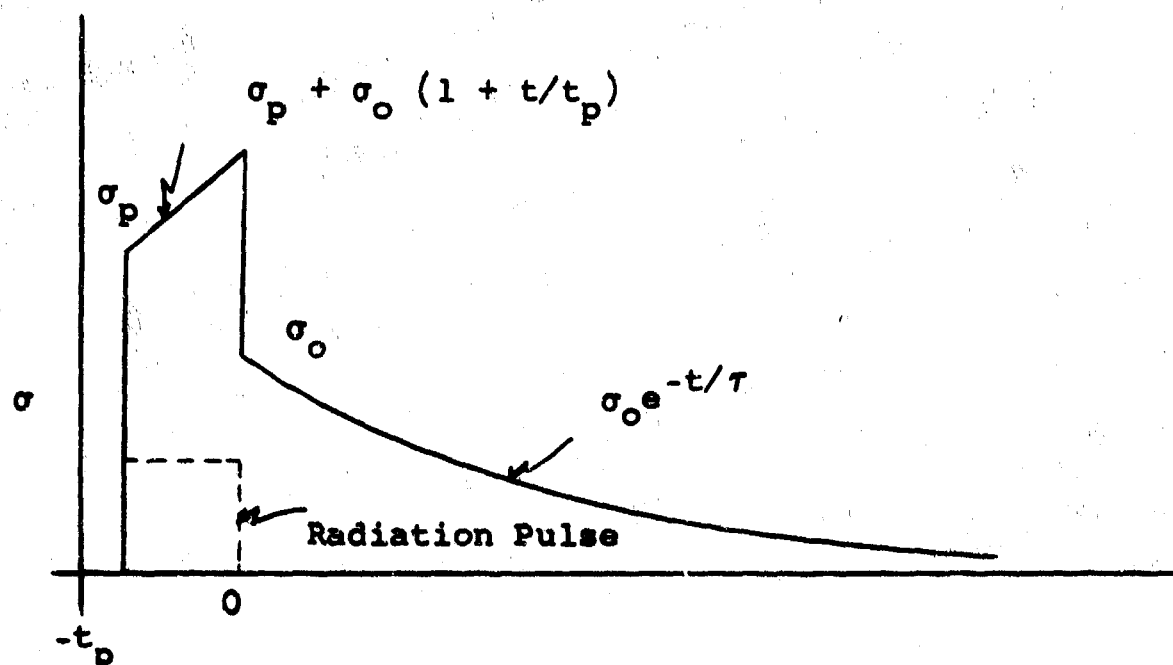
Figure 4. Induced Conductivity-Time Curve in a Capacitor due to the Radiation Pulse Shown.
