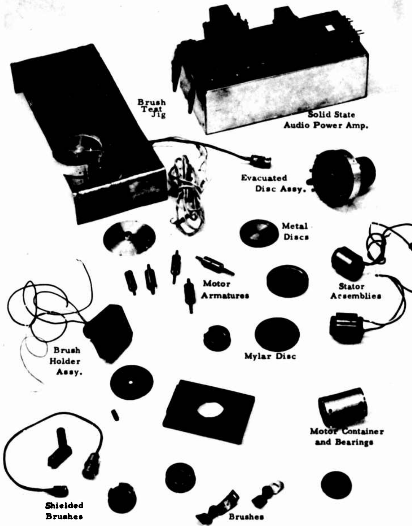
FIG. 20 - MOTOR/MAGNETIC HARDWARE
