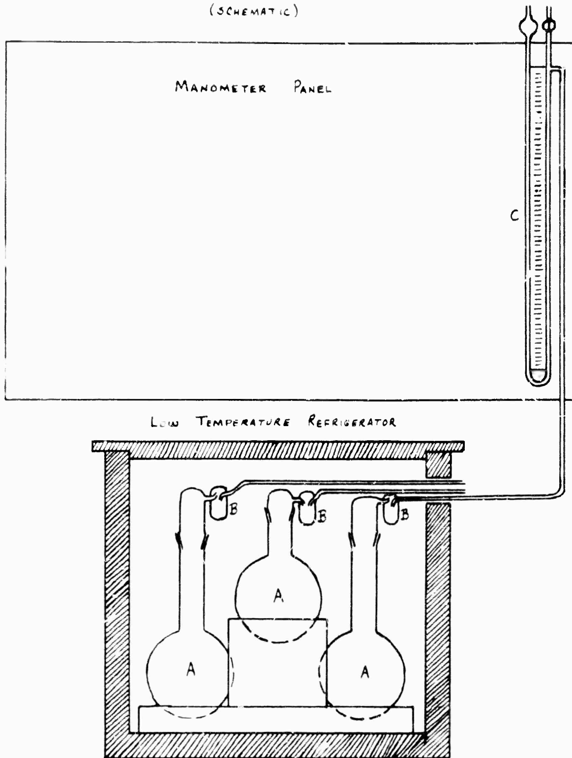
A- DECOMPOSITION FLASKS (3 OF 12 SHOWN) B- KEROSENE TRAPS (3 OF 12 SHOWN) C- KEROSENE DIFFERENTIAL MANOMETER (1 OF 12 SHOWN)
