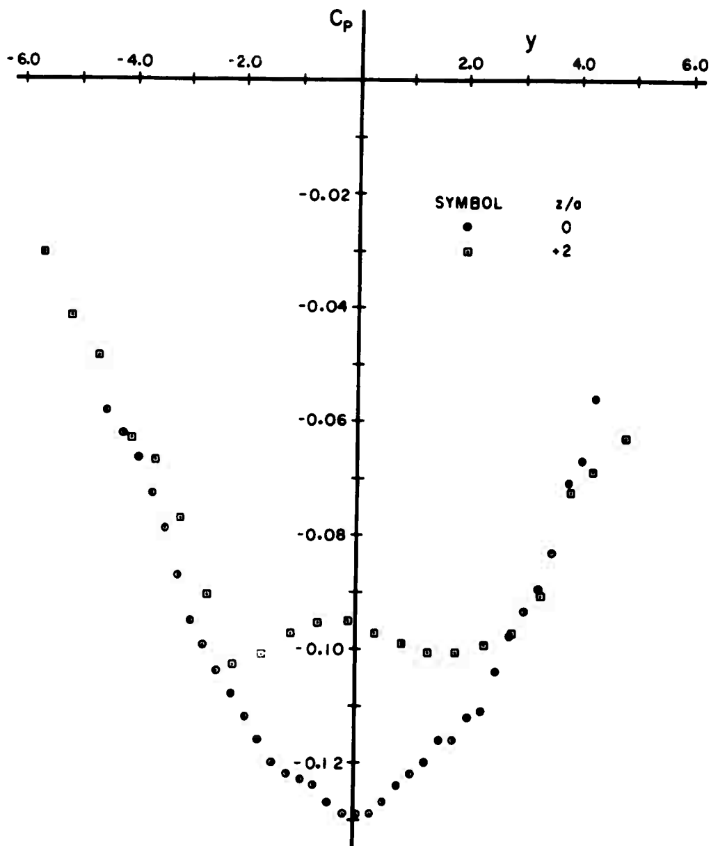
FIG. 25 C_p(y) VERSUS y FOR x/a=30 , z/a=0, 0.2
