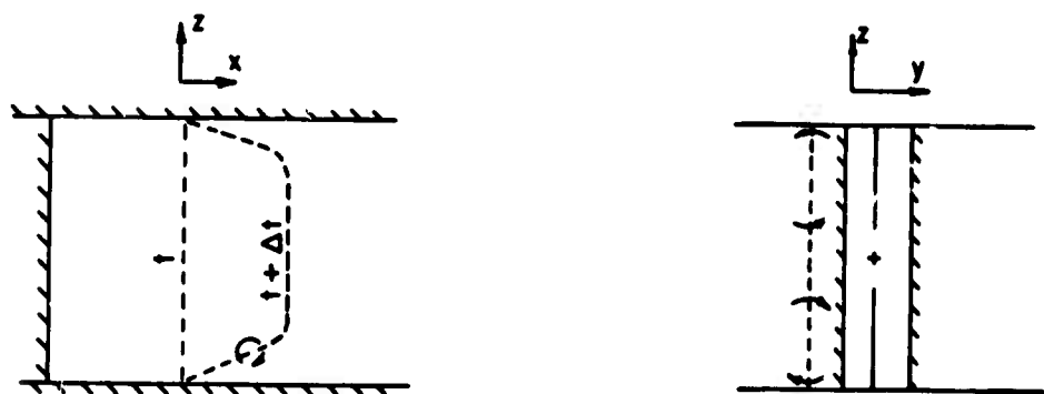
(a.) VORTEX GENERATION AT TIME t
