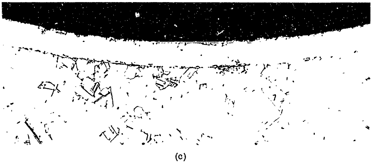
Fig. 10 - Silver-clad OFHC copper outer conductor after 200 hours at 350°C in air. X150.
