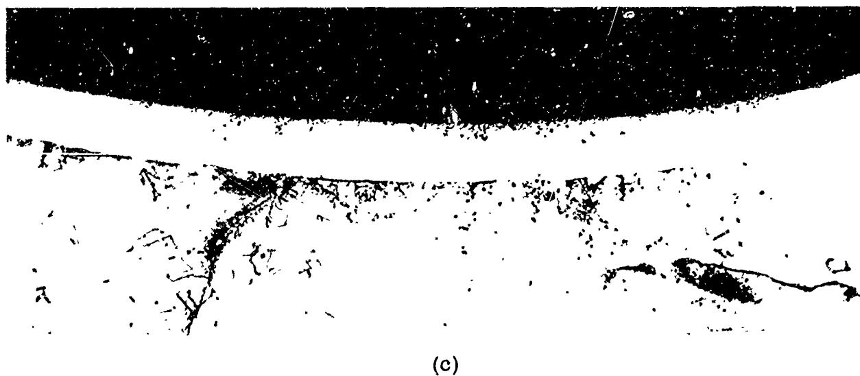
Fig. 12 - Silver-clad OFHC copper outer conductor after 200 hours at 350^{\circ}\text{C} in nitrogen. X150.
