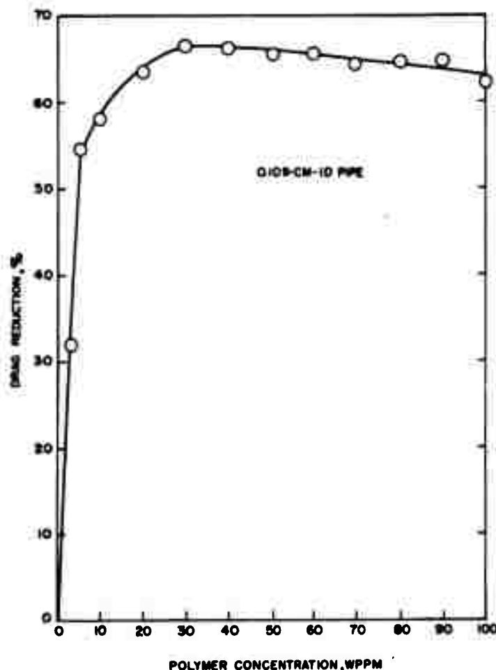
FIG. 18. Turbulent-Flow Rheometer Data for Poly(Ethylene Oxide).
