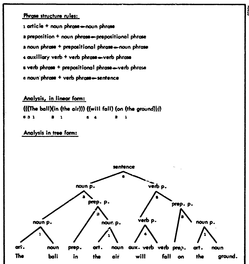
Figure 1. Examples of phrase-structure rules and the analysis of a sentence, in linear form and in tree form, through the use of these rules.
