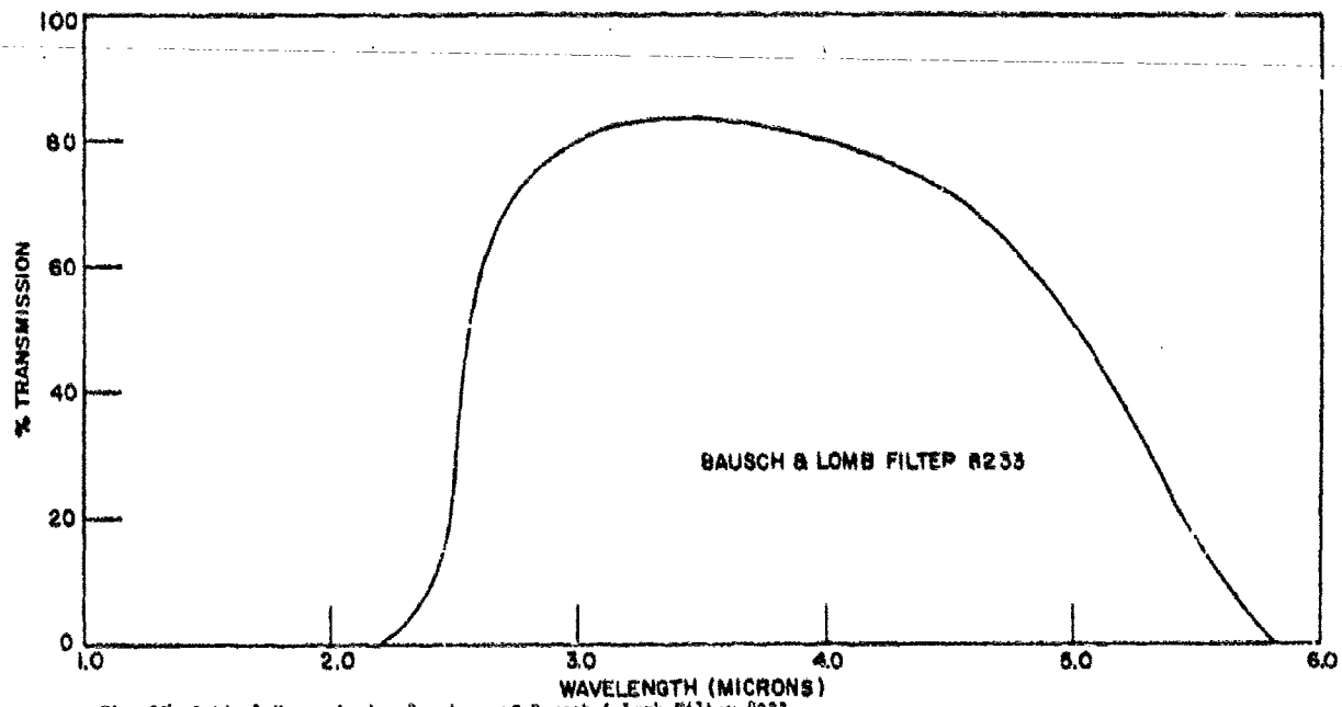
Fig. 15. Optical Transmission Spectrum of Bausch & Lomb Filter R233
