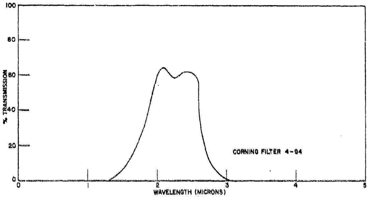
Fig. 22 Optical Transmission Spectrum of Corning Filter 4-94
