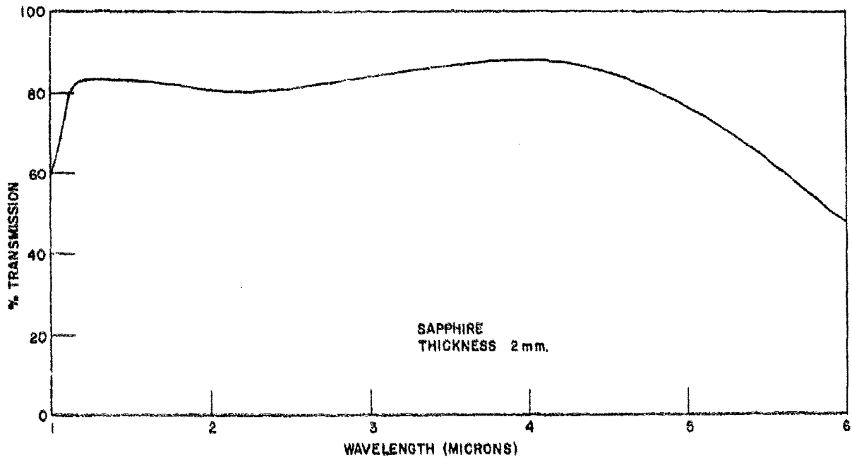
Fig. 6 Optical Transmission Spectrum of Sapphire
