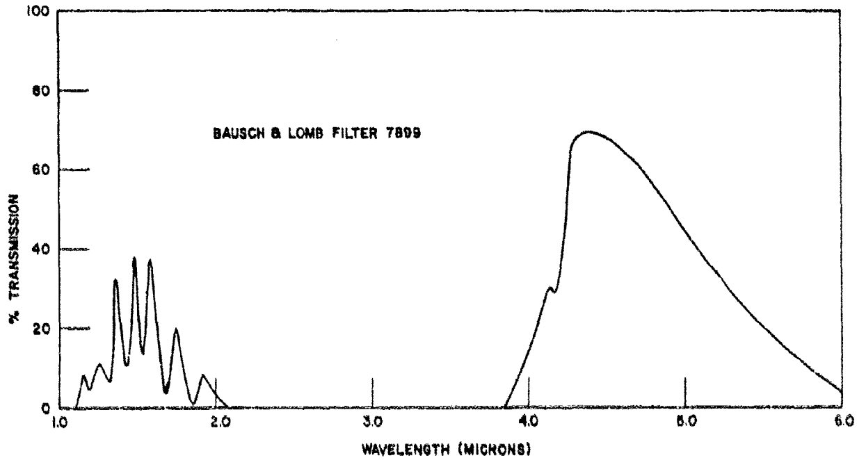
Fig. 18 Optical Transmission Spectrum of Bausch & Lomb Filter 7899
