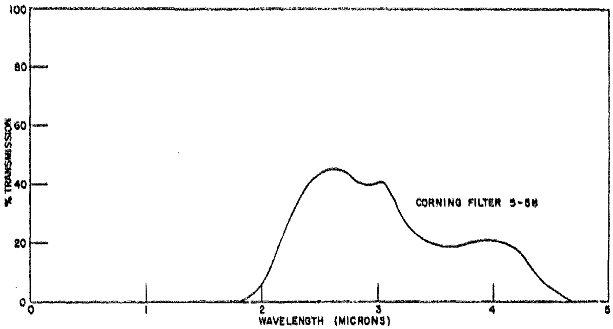
Fig. 23 Optical Transmission Spectrum of Corning Filter 5-68
